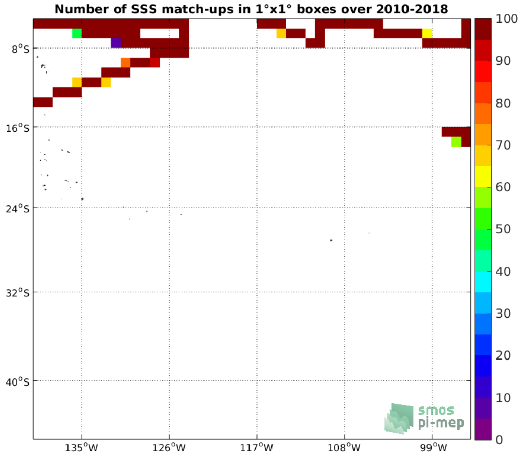
Figure 4: Number of SSS match-ups between TSG (SAMOS) SSS and the SMOS SSS L3 v317 - Monthly - 25 km (CATDS-CPDC) SSS product for the OTT zone Pi-MEP region over 1^\circ \times 1^\circ boxes and for the full satellite product period.
