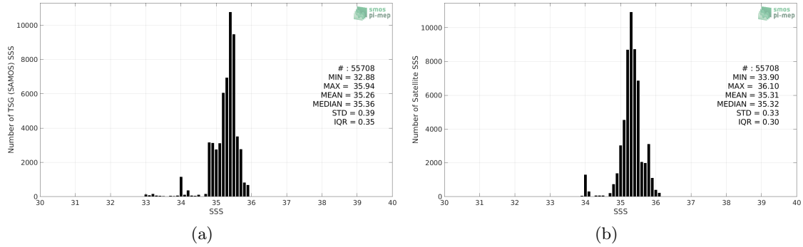
Figure 2: Histograms of SSS from TSG (SAMOS) (a) and SMOS SSS L3 v317 - Monthly - 25 km (CATDS-CPDC) (b) considering all match-up pairs per bins of 0.1 over the OTT zone Pi-MEP region and for the full satellite product period.
