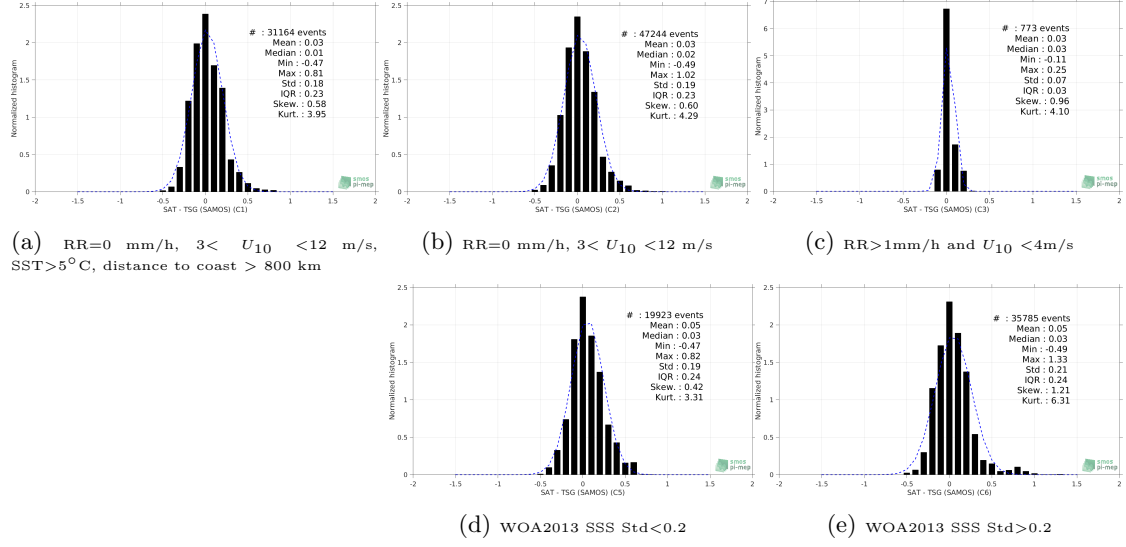
Figure 13: Normalized histogram of \Delta SSS (SMOS SSS L3 v317 - Monthly - 25 km (CATDS-CPDC) - TSG (SAMOS)) for 5 different subdatasets corresponding to: RR=0 mm/h, 3 < U_{10} < 12 m/s, SST > 5^\circ C , distance to coast > 800 km (a), RR=0 mm/h, 3 < U_{10} < 12 m/s (b), RR > 1 mm/h and U_{10} < 4 m/s (c), WOA2013 SSS Std < 0.2 (d), WOA2013 SSS Std > 0.2 (e).
