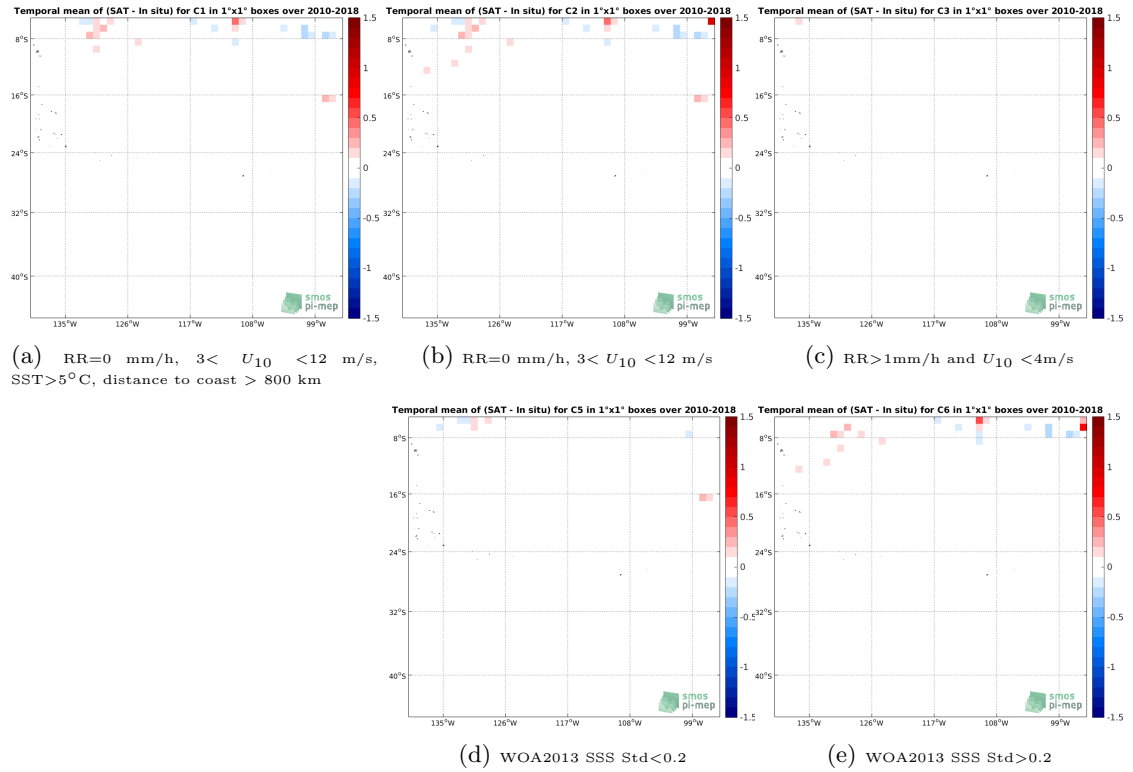
Figure 12: Temporal mean gridded over spatial boxes of size 1^\circ \times 1^\circ of \Delta SSS (SMOS SSS L3 v317 - Monthly - 25 km (CATDS-CPDC) - TSG (SAMOS)) for 5 different subdatasets corresponding to: RR=0 mm/h, 3 < U_{10} < 12 m/s, SST > 5^\circ C , distance to coast > 800 km (a), RR=0 mm/h, 3 < U_{10} < 12 m/s (b), RR > 1 mm/h and U_{10} < 4 m/s (c), WOA2013 SSS Std < 0.2 (d), WOA2013 SSS Std > 0.2 (e).
