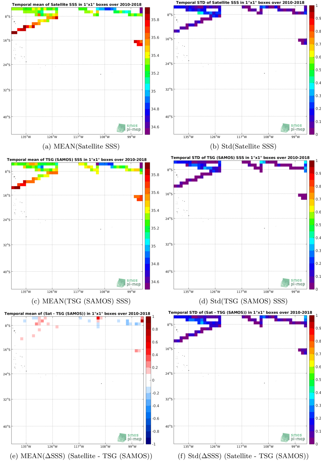
Figure 6: Temporal mean (left) and Std (right) of SSS from SMOS SSS L3 v317 - Monthly - 25 km (CATDS-CPDC) (top), TSG (SAMOS) (middle), and of \Delta SSS (Satellite - TSG (SAMOS)). Only match-up pairs are used to generate these maps.
