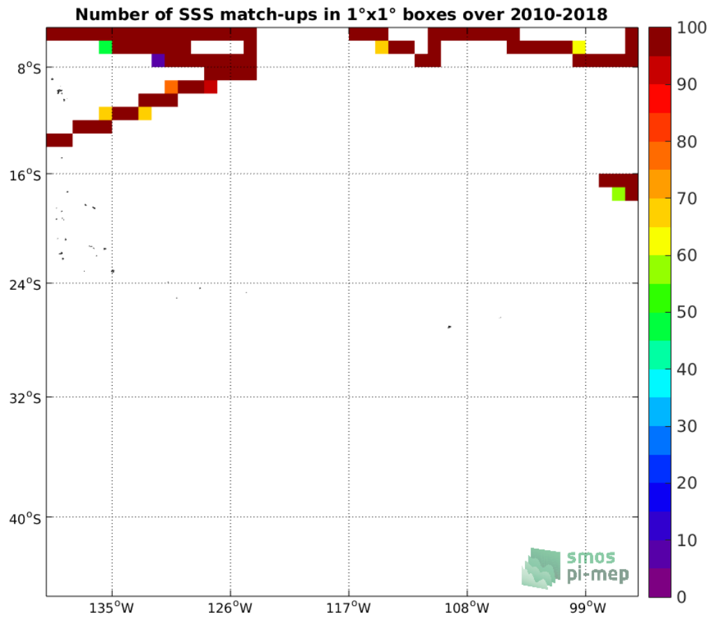
Figure 4: Number of SSS match-ups between TSG (SAMOS) SSS and the SMOS SSS L3 v317 - Monthly - 25 km (CATDS-CPDC) SSS product for the OTT zone Pi-MEP region over 1°x1° boxes and for the full satellite product period.
