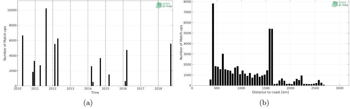
Figure 1: Number of match-ups between TSG (SAMOS) and SMOS SSS L3 v317 - Monthly - 25 km (CATDS-CPDC) SSS as a function of time (a) and as function of the distance to coast (b) over the OTT zone Pi-MEP region and for the full satellite product period.
