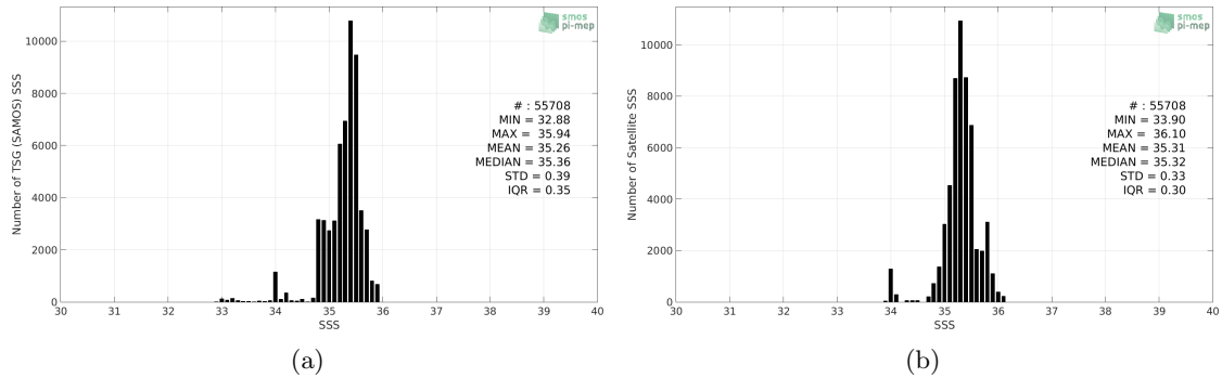
Figure 2: Histograms of SSS from TSG (SAMOS) (a) and SMOS SSS L3 v317 - Monthly - 25 km (CATDS-CPDC) (b) considering all match-up pairs per bins of 0.1 over the OTT zone Pi-MEP region and for the full satellite product period.
