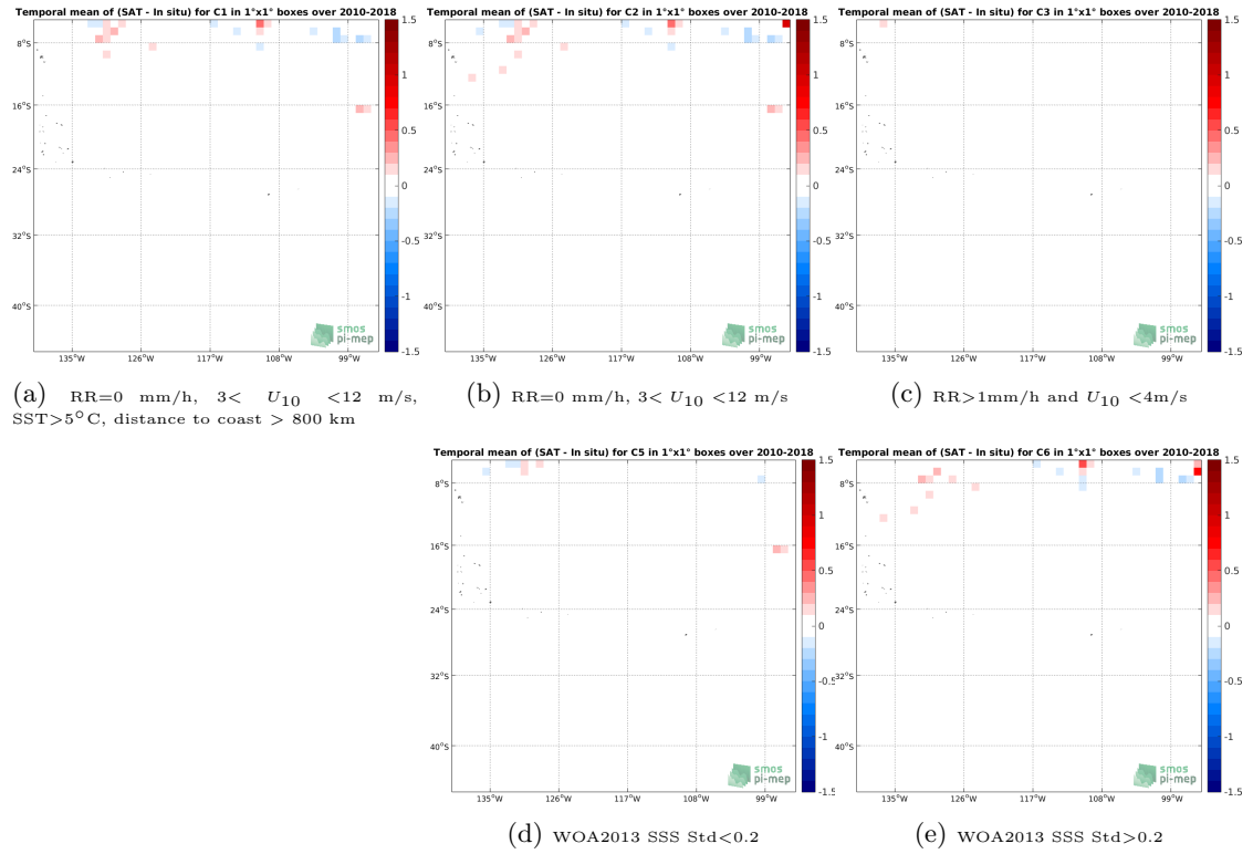
Figure 12: Temporal mean gridded over spatial boxes of size 1^\circ \times 1^\circ of \Delta SSS (SMOS L3 v317 - Monthly - 25 km (CATDS-CPDC) - TSG-SAMOS) for 5 different subdatasets corresponding to: RR=0 mm/h, 3 < U_{10} < 12 m/s, SST >5^\circ C, distance to coast > 800 km (a), RR=0 mm/h, 3 < U_{10} < 12 m/s (b), RR >1 mm/h and U_{10} < 4 m/s (c), WOA2013 SSS Std <0.2 (d), WOA2013 SSS Std >0.2 (e).
