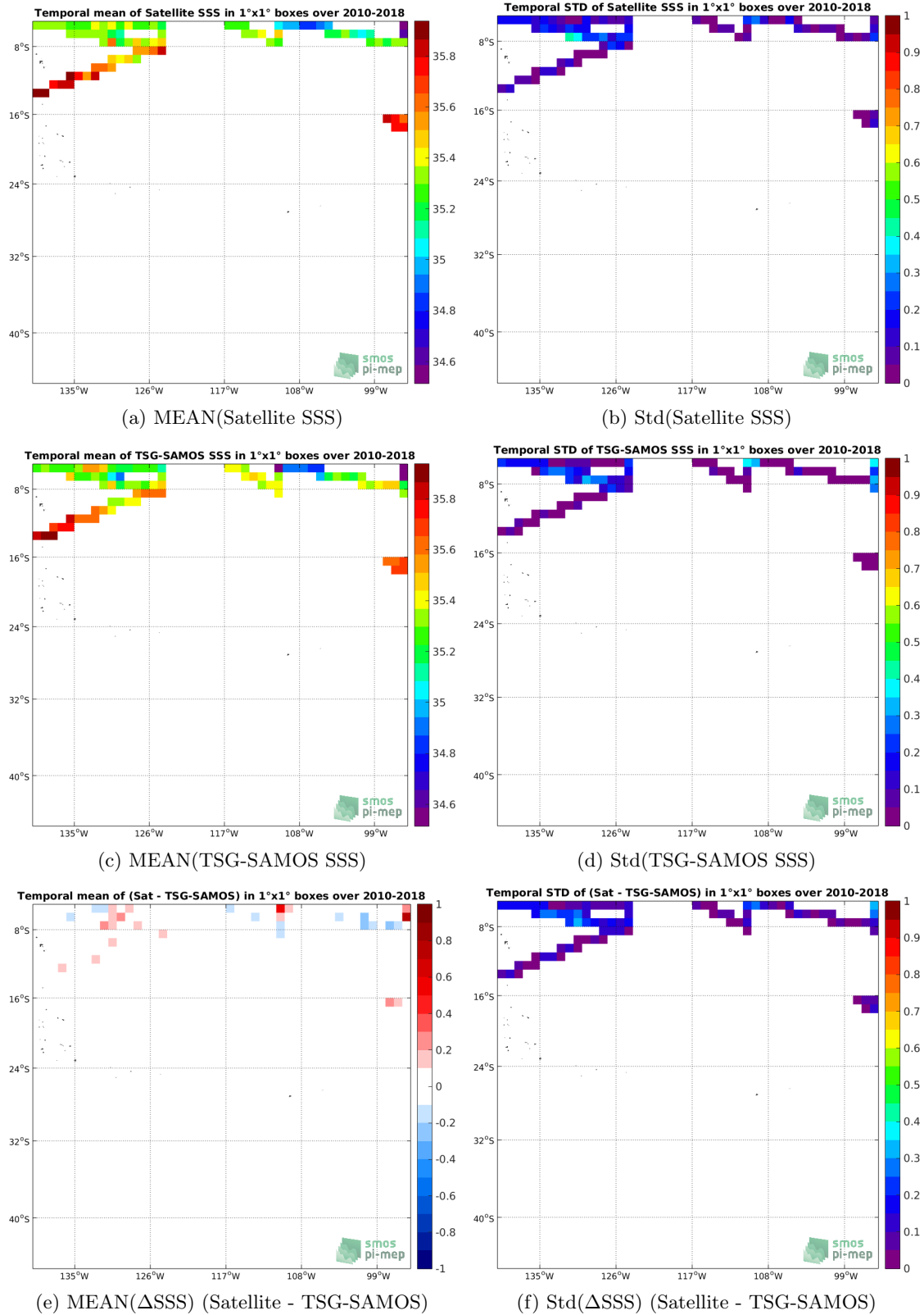
Figure 6: Temporal mean (left) and Std (right) of SSS from SMOS L3 v317 - Monthly - 25 km (CATDS-CPDC) (top), TSG-SAMOS (middle), and of \Delta SSS (Satellite - TSG-SAMOS). Only match-up pairs are used to generate these maps.
