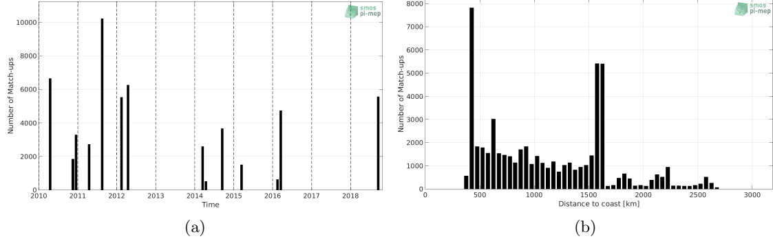
Figure 1: Number of match-ups between TSG-SAMOS and SMOS L3 v317 - Monthly - 25 km (CATDS-CPDC) SSS as a function of time (a) and as function of the distance to coast (b) over the OTT zone Pi-MEP region and for the full satellite product period.
