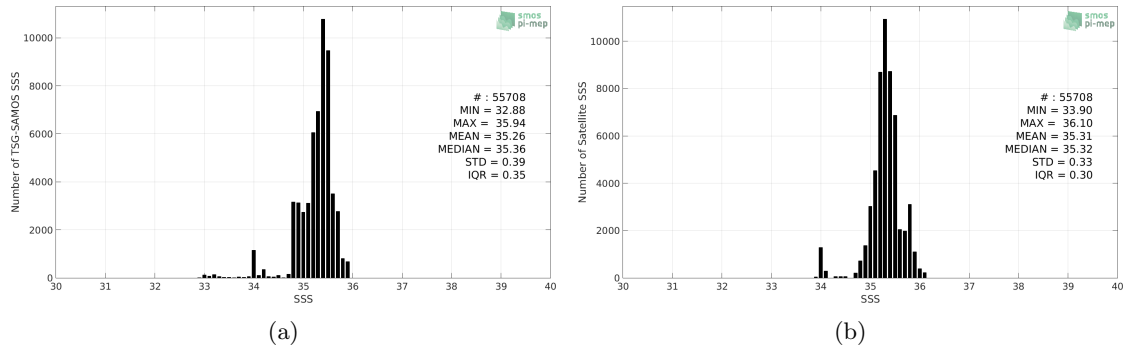
Figure 2: Histograms of SSS from TSG-SAMOS (a) and SMOS L3 v317 - Monthly - 25 km (CATDS-CPDC) (b) considering all match-up pairs per bins of 0.1 over the OTT zone Pi-MEP region and for the full satellite product period.
