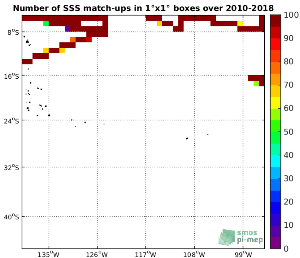
Figure 4: Number of SSS match-ups between TSG-SAMOS SSS and the SMOS-L3-CATDS-CPDC-V317-MONTHLY-25KM SSS product for the OTT zone Pi-MEP region over 1°x1° boxes and for the full satellite product period.
