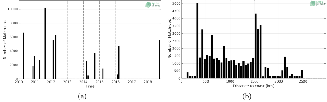
Figure 1: Number of match-ups between TSG-SAMOS and SMOS-L3-CATDS-CPDC-V317-MONTHLY-25KM SSS as a function of time (a) and as function of the distance to coast (b) over the OTT zone Pi-MEP region and for the full satellite product period.
