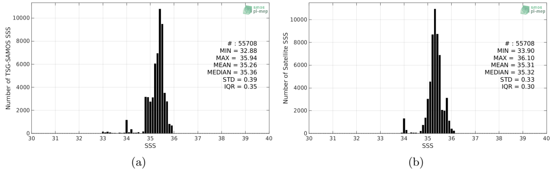
Figure 2: Histograms of SSS from TSG-SAMOS (a) and SMOS-L3-CATDS-CPDC-V317-MONTHLY-25KM (b) considering all match-up pairs per bins of 0.1 over the OTT zone Pi-MEP region and for the full satellite product period.
