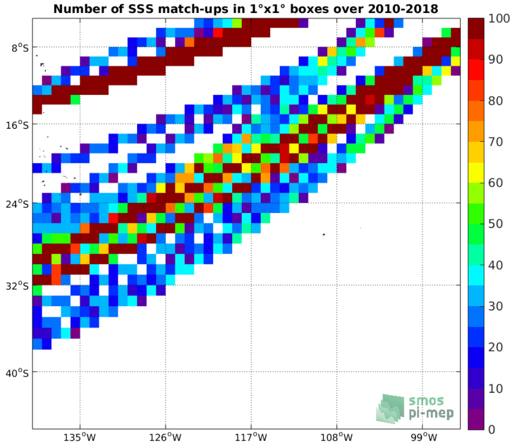
Figure 4: Number of SSS match-ups between TSG (LEGOS-DM) SSS and the SMOS SSS L3 v317 - Monthly - 25 km (CATDS-CPDC) SSS product for the OTT zone Pi-MEP region over 1°x1° boxes and for the full satellite product period.
