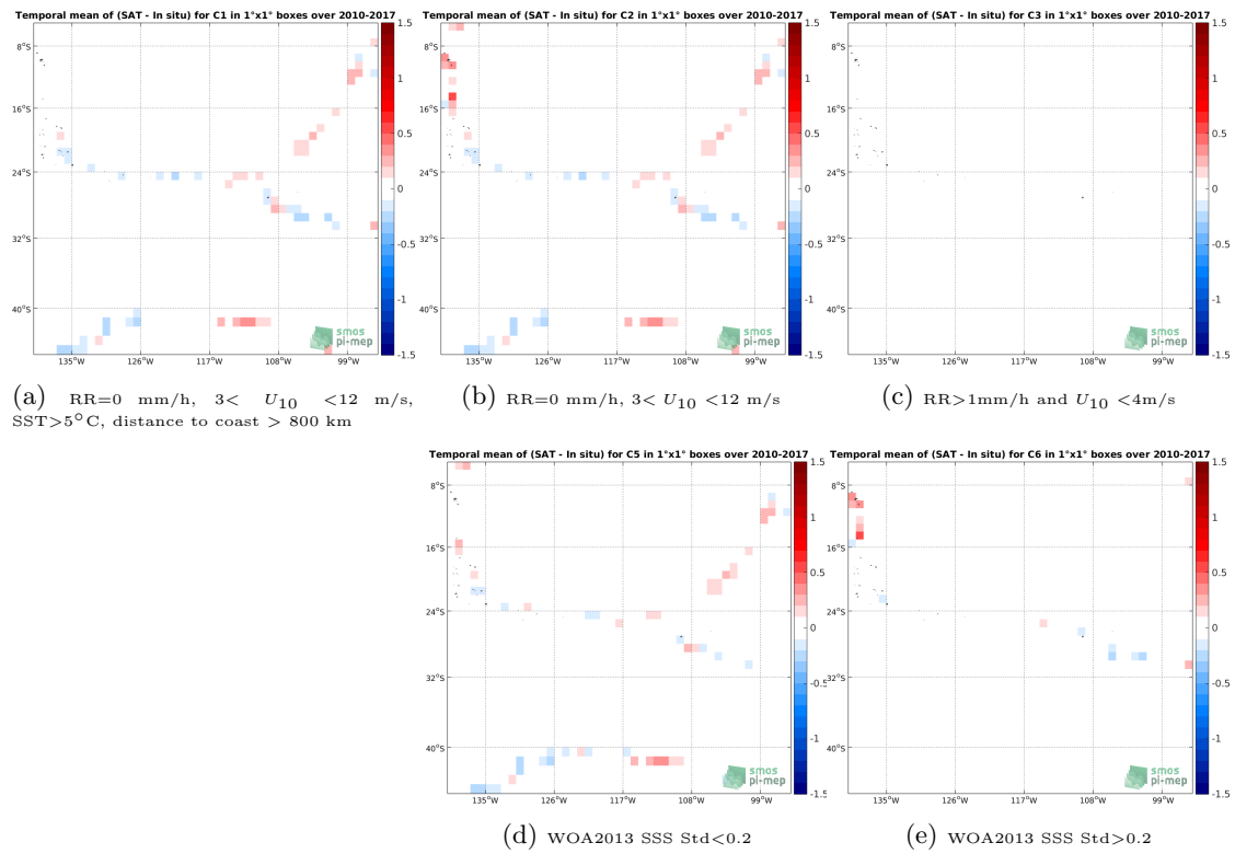
Figure 12: Temporal mean gridded over spatial boxes of size 1^\circ \times 1^\circ of \Delta\text{SSS} (SMOS SSS L3 v317 - Monthly - 25 km (CATDS-CPDC) - TSG (GOSUD-Sailing-ship)) for 5 different subdatasets corresponding to:RR=0 mm/h, 3 < U_{10} < 12 m/s, SST>5°C, distance to coast > 800 km (a), RR=0 mm/h, 3 < U_{10} < 12 m/s (b), RR>1mm/h and U_{10} < 4 m/s (c), WOA2013 SSS Std<0.2 (d), WOA2013 SSS Std>0.2 (e).
