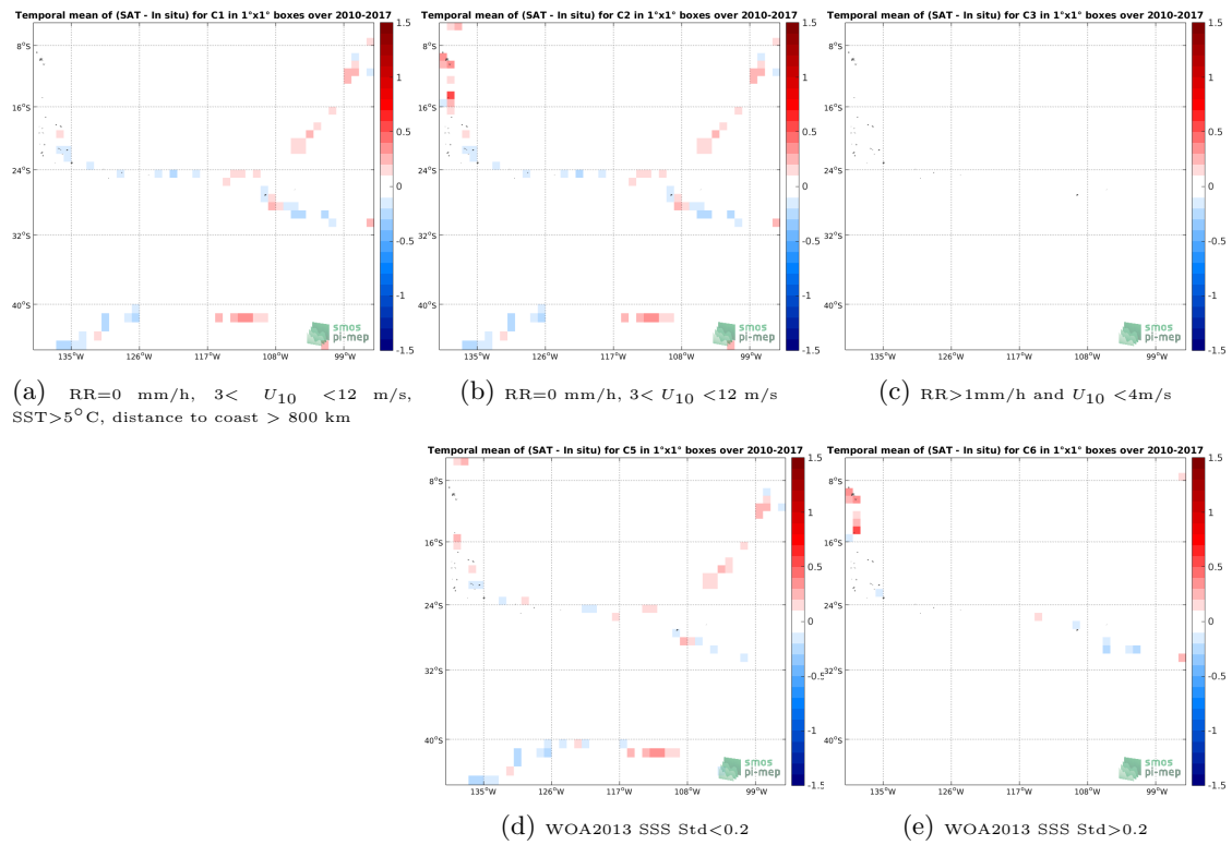
Figure 12: Temporal mean gridded over spatial boxes of size 1^\circ \times 1^\circ of \Delta\text{SSS} (SMOS SSS L3 v317 - Monthly - 25 km (CATDS-CPDC) - TSG (GOSUD-Sailing-ship)) for 5 different subdatasets corresponding to: \text{RR}=0 \text{ mm/h} , 3 < U_{10} < 12 \text{ m/s} , \text{SST} > 5^\circ\text{C} , distance to coast > 800 \text{ km} (a), \text{RR}=0 \text{ mm/h} , 3 < U_{10} < 12 \text{ m/s} (b), \text{RR} > 1 \text{ mm/h} and U_{10} < 4 \text{ m/s} (c), WOA2013 SSS Std < 0.2 (d), WOA2013 SSS Std > 0.2 (e).
