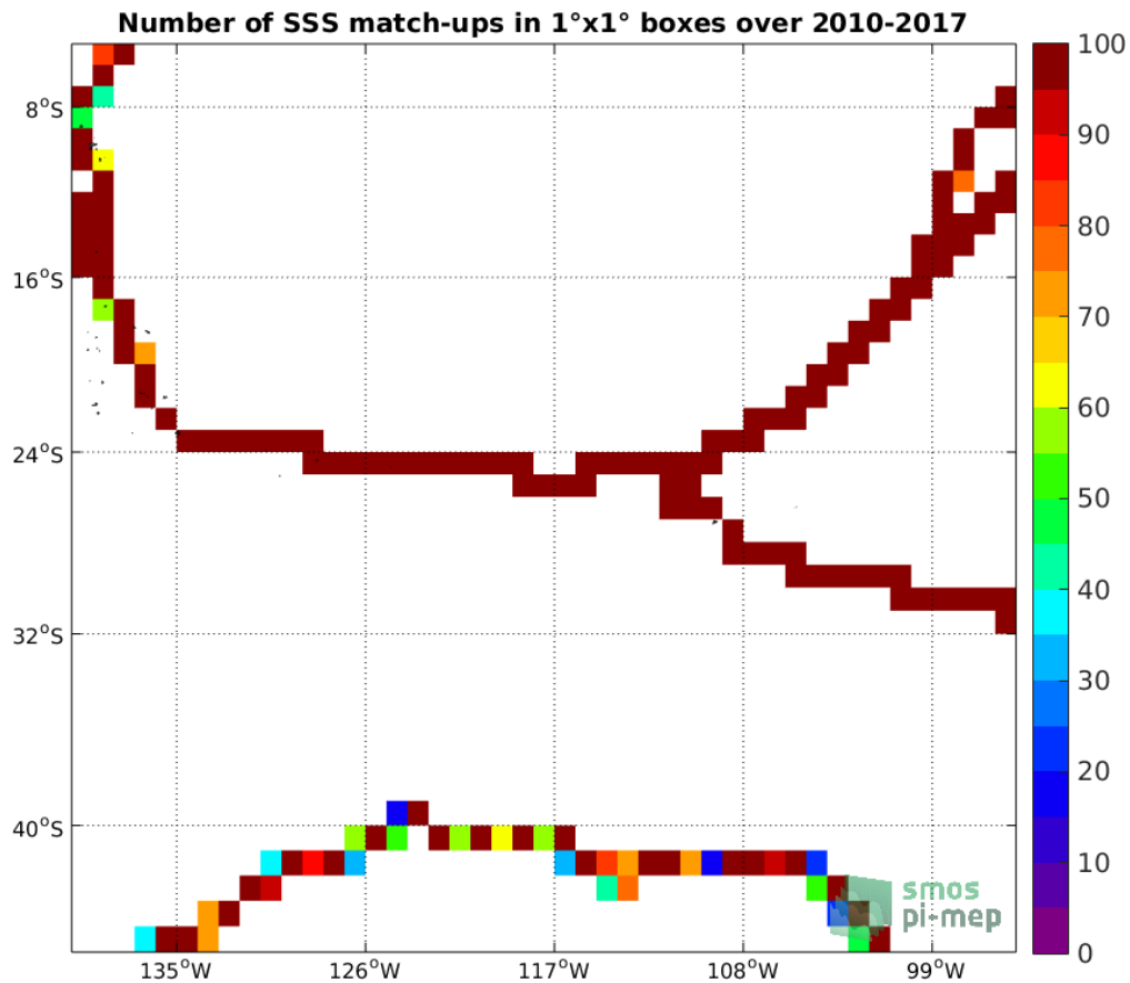
Figure 4: Number of SSS match-ups between TSG (GOSUD-Sailing-ship) SSS and the SMOS SSS L3 v317 - Monthly - 25 km (CATDS-CPDC) SSS product for the OTT zone Pi-MEP region over 1^\circ \times 1^\circ boxes and for the full satellite product period.
