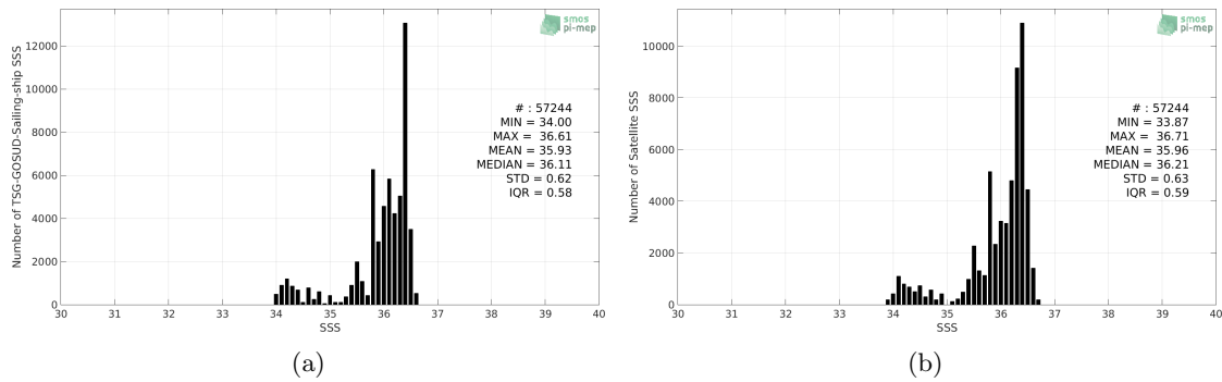
Figure 2: Histograms of SSS from TSG-GOSUD-Sailing-ship (a) and SMOS L3 v317 - Monthly - 25 km (CATDS-CPDC) (b) considering all match-up pairs per bins of 0.1 over the OTT zone Pi-MEP region and for the full satellite product period.
