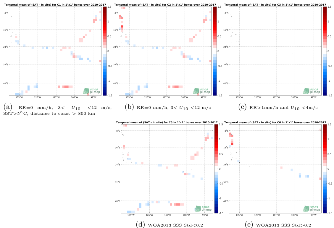
Figure 12: Temporal mean gridded over spatial boxes of size 1^\circ \times 1^\circ of \Delta SSS (SMOS L3 v317 - Monthly - 25 km (CATDS-CPDC) - TSG-GOSUD-Sailing-ship) for 5 different subdatasets corresponding to:RR=0 mm/h, 3 < U_{10} < 12 m/s, SST >5^\circ\text{C} , distance to coast > 800 km (a), RR=0 mm/h, 3 < U_{10} < 12 m/s (b), RR >1 mm/h and U_{10} < 4 m/s (c), WOA2013 SSS Std <0.2 (d), WOA2013 SSS Std >0.2 (e).
