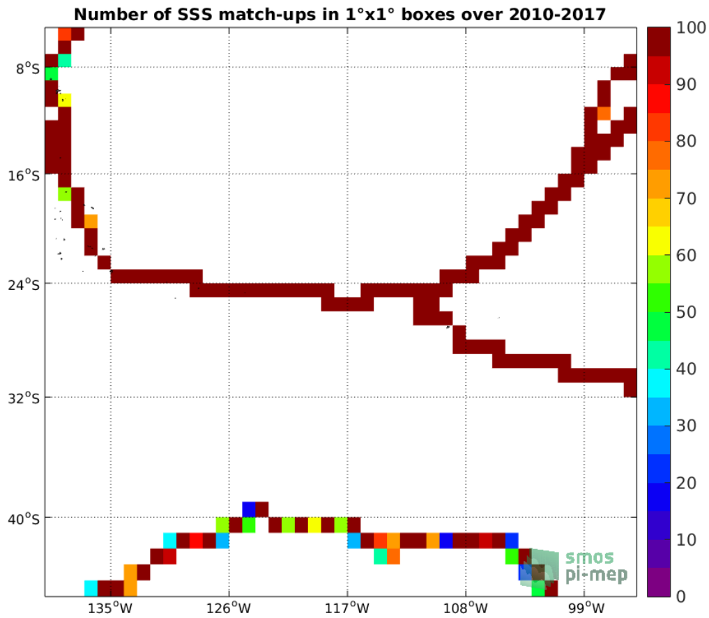
Figure 4: Number of SSS match-ups between TSG-GOSUD-Sailing-ship SSS and the SMOS L3 v317 - Monthly - 25 km (CATDS-CPDC) SSS product for the OTT zone Pi-MEP region over 1°x1° boxes and for the full satellite product period.
