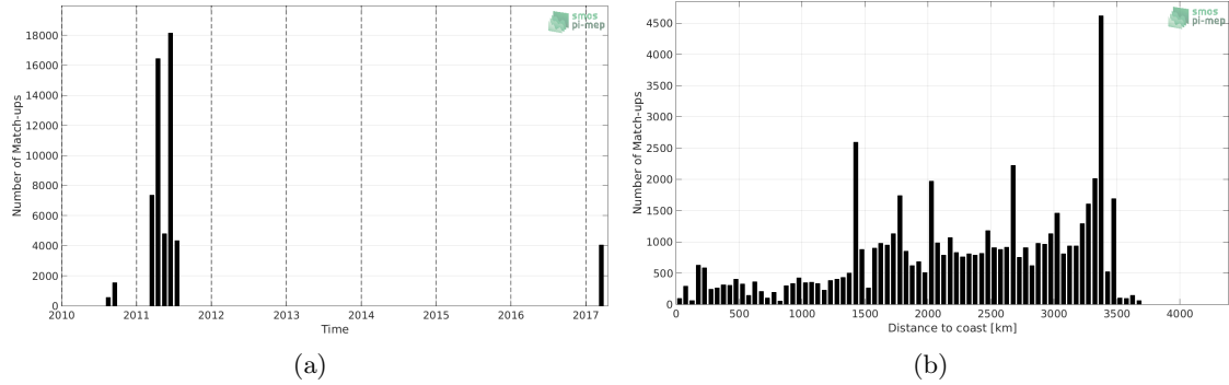
Figure 1: Number of match-ups between TSG-GOSUD-Sailing-ship and SMOS L3 v317 - Monthly - 25 km (CATDS-CPDC) SSS as a function of time (a) and as function of the distance to coast (b) over the OTT zone Pi-MEP region and for the full satellite product period.
