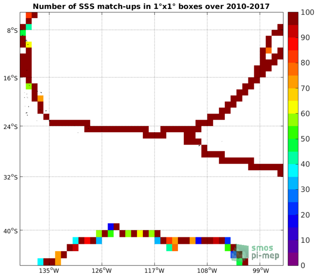
Figure 4: Number of SSS match-ups between TSG-GOSUD-Sailing-ship SSS and the SMOS-L3-CATDS-CPDC-V317-MONTHLY-25KM SSS product for the OTT zone Pi-MEP region over 1°x1° boxes and for the full satellite product period.
