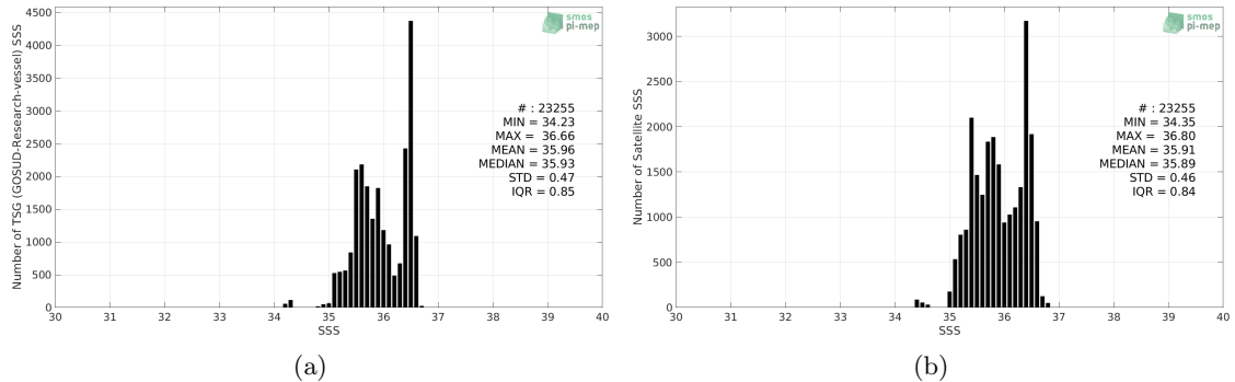
Figure 2: Histograms of SSS from TSG (GOSUD-Research-vessel) (a) and SMOS SSS L3 v317 - Monthly - 25 km (CATDS-CPDC) (b) considering all match-up pairs per bins of 0.1 over the OTT zone Pi-MEP region and for the full satellite product period.
