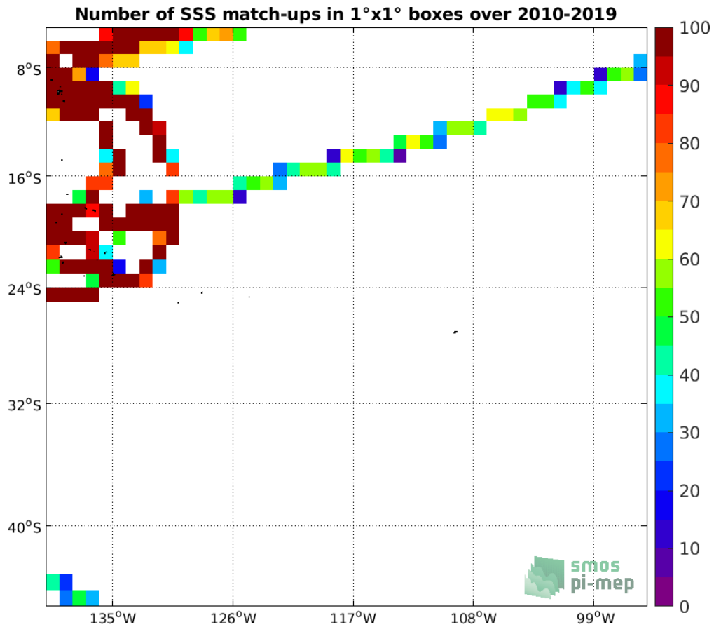
Figure 4: Number of SSS match-ups between TSG (GOSUD-Research-vessel) SSS and the SMOS SSS L3 v317 - Monthly - 25 km (CATDS-CPDC) SSS product for the OTT zone Pi-MEP region over 1^\circ \times 1^\circ boxes and for the full satellite product period.
