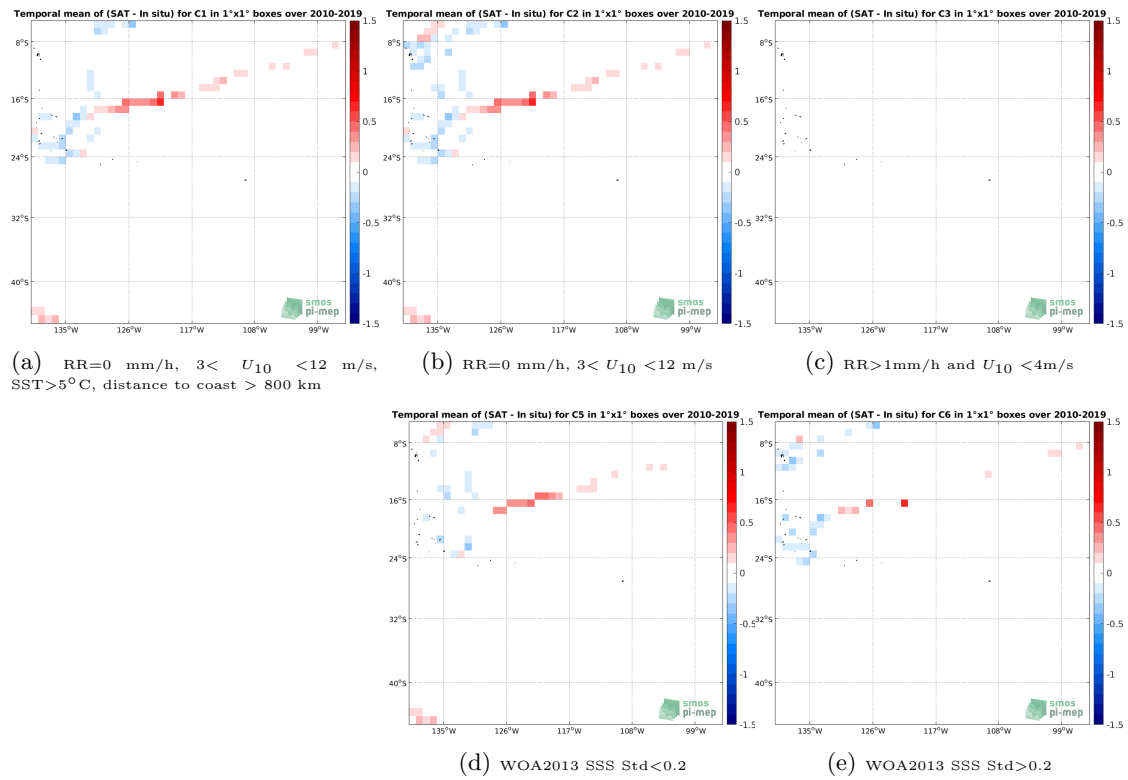
Figure 12: Temporal mean gridded over spatial boxes of size 1^\circ \times 1^\circ of \Delta\text{SSS} (SMOS SSS L3 v317 - Monthly - 25 km (CATDS-CPDC) - TSG (GOSUD-Research-vessel)) for 5 different subdatasets corresponding to: RR=0 mm/h, 3 < U_{10} < 12 m/s, SST > 5°C, distance to coast > 800 km (a), RR=0 mm/h, 3 < U_{10} < 12 m/s (b), RR > 1 mm/h and U_{10} < 4 m/s (c), WOA2013 SSS Std < 0.2 (d), WOA2013 SSS Std > 0.2 (e).
