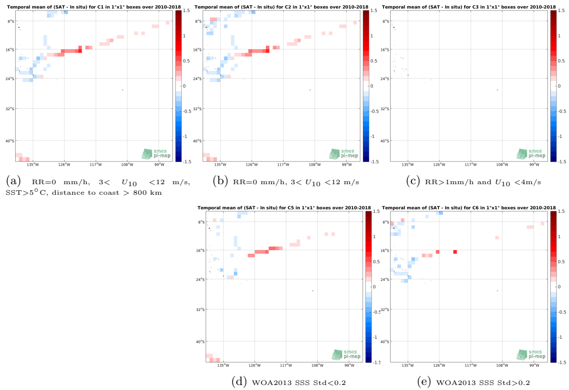
Figure 12: Temporal mean gridded over spatial boxes of size 1^\circ \times 1^\circ of \Delta\text{SSS} (SMOS SSS L3 v317 - Monthly - 25 km (CATDS-CPDC) - TSG (GOSUD-Research-vessel)) for 5 different subdatasets corresponding to: \text{RR}=0 \text{ mm/h} , 3 < U_{10} < 12 \text{ m/s} , \text{SST} > 5^\circ\text{C} , distance to coast > 800 \text{ km} (a), \text{RR}=0 \text{ mm/h} , 3 < U_{10} < 12 \text{ m/s} (b), \text{RR} > 1\text{mm/h} and U_{10} < 4\text{m/s} (c), WOA2013 SSS Std < 0.2 (d), WOA2013 SSS Std > 0.2 (e).
