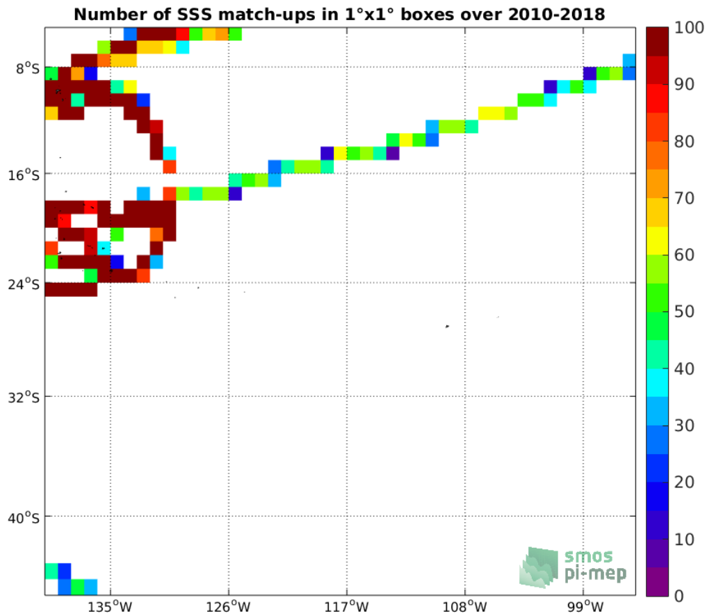
Figure 4: Number of SSS match-ups between TSG (GOSUD-Research-vessel) SSS and the SMOS SSS L3 v317 - Monthly - 25 km (CATDS-CPDC) SSS product for the OTT zone Pi-MEP region over 1°x1° boxes and for the full satellite product period.
