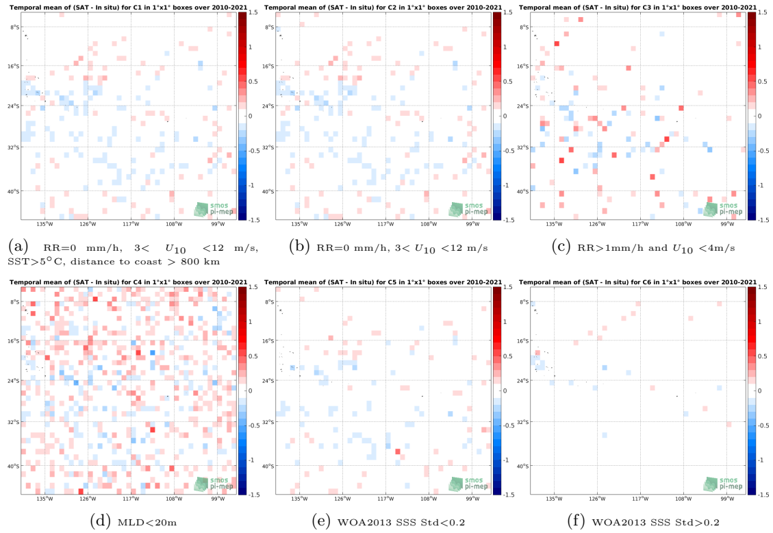
Figure 12: Temporal mean gridded over spatial boxes of size 1^\circ \times 1^\circ of \Delta SSS (SMOS SSS L3 v317 - Monthly - 25 km (CATDS-CPDC) - Argo) for 6 different subdatasets corresponding to:RR=0 mm/h, 3 < U_{10} < 12 m/s, SST >5^\circ C, distance to coast > 800 km (a), RR=0 mm/h, 3 < U_{10} < 12 m/s (b), RR >1 mm/h and U_{10} < 4 m/s (c),MLD <20 m (d),WOA2013 SSS Std <0.2 (e),WOA2013 SSS Std >0.2 (f).
