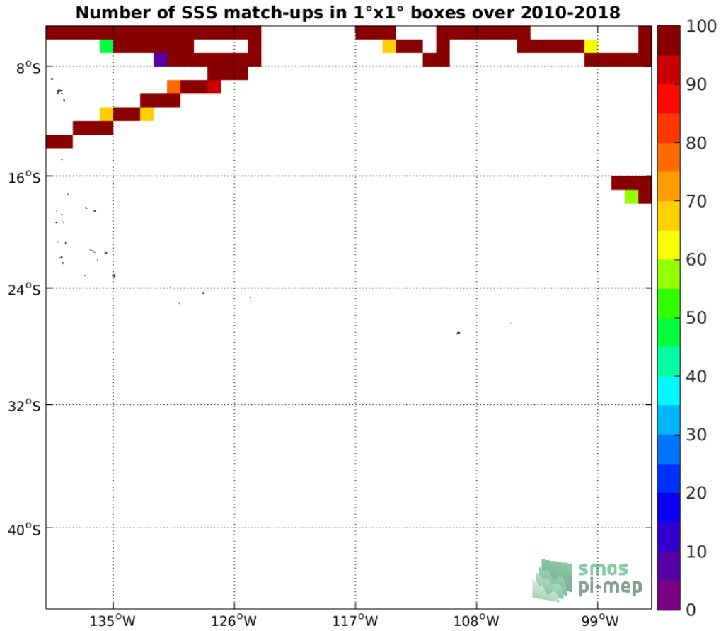
Figure 4: Number of SSS match-ups between TSG (SAMOS) SSS and the SMOS SSS L3 v317 - 10 Days - 25 km (CATDS-CPDC) SSS product for the OTT zone Pi-MEP region over 1^\circ \times 1^\circ boxes and for the full satellite product period.
