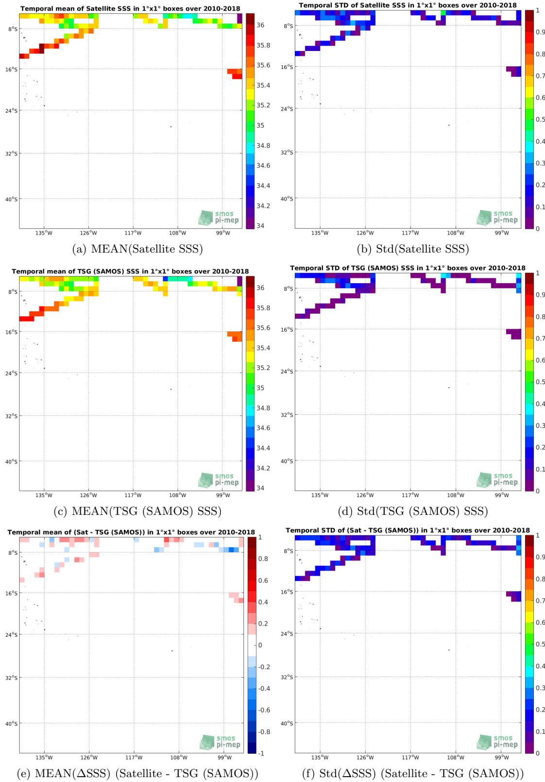
Figure 6: Temporal mean (left) and Std (right) of SSS from SMOS SSS L3 v317 - 10 Days - 25 km (CATDS-CPDC) (top), TSG (SAMOS) (middle), and of \Delta SSS (Satellite - TSG (SAMOS)). Only match-up pairs are used to generate these maps.
