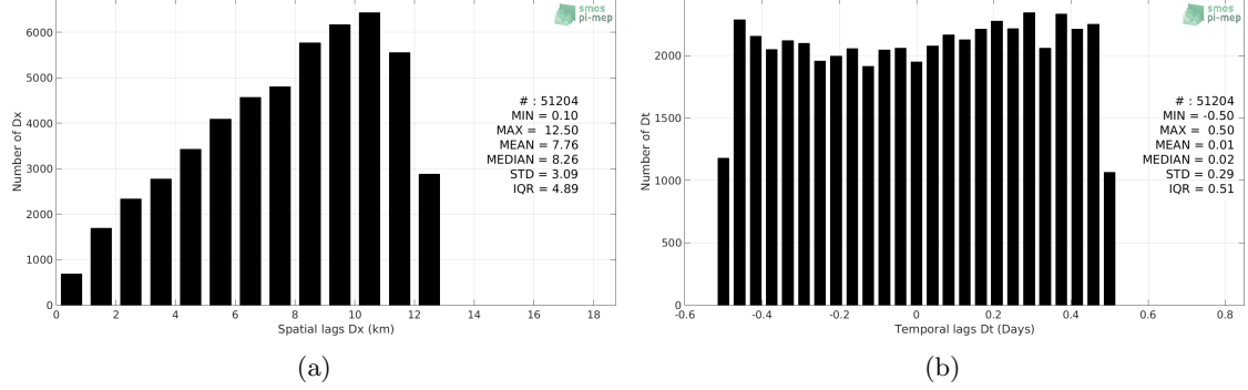
Figure 5: Histograms of the spatial (a) and temporal (b) lags between the time of the TSG (SAMOS) measurements and the date of the corresponding SMOS SSS L3 v317 - 10 Days - 25 km (CATDS-CPDC) SSS product.
