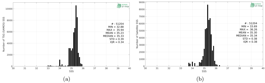
Figure 2: Histograms of SSS from TSG (SAMOS) (a) and SMOS SSS L3 v317 - 10 Days - 25 km (CATDS-CPDC) (b) considering all match-up pairs per bins of 0.1 over the OTT zone Pi-MEP region and for the full satellite product period.
