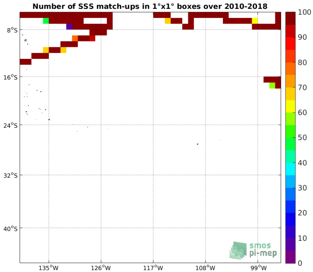
Figure 4: Number of SSS match-ups between TSG (SAMOS) SSS and the SMOS SSS L3 v317 - 10 Days - 25 km (CATDS-CPDC) SSS product for the OTT zone Pi-MEP region over 1°x1° boxes and for the full satellite product period.
