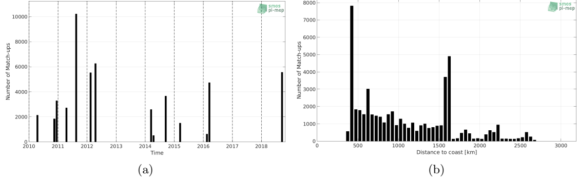
Figure 1: Number of match-ups between TSG (SAMOS) and SMOS SSS L3 v317 - 10 Days - 25 km (CATDS-CPDC) SSS as a function of time (a) and as function of the distance to coast (b) over the OTT zone Pi-MEP region and for the full satellite product period.
