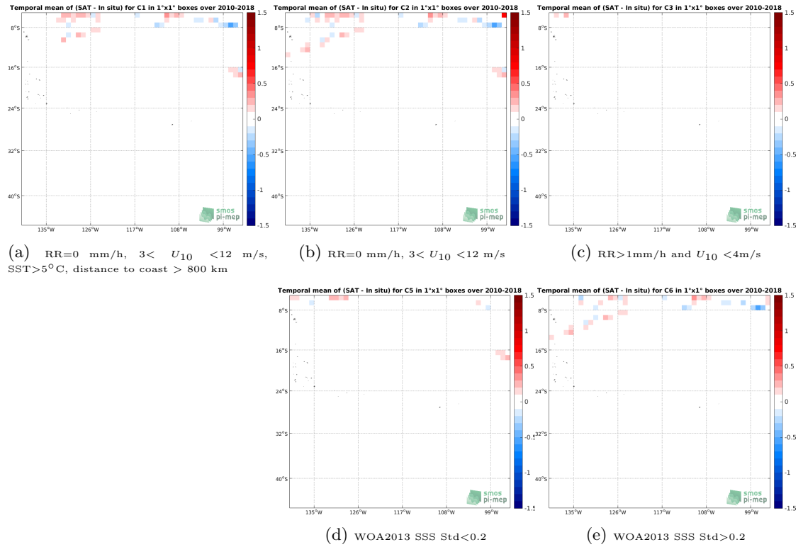
Figure 12: Temporal mean gridded over spatial boxes of size 1^\circ \times 1^\circ of \Delta SSS (SMOS SSS L3 v317 - 10 Days - 25 km (CATDS-CPDC) - TSG (SAMOS)) for 5 different subdatasets corresponding to: RR=0 mm/h, 3 < U_{10} < 12 m/s, SST > 5^\circ C , distance to coast > 800 km (a), RR=0 mm/h, 3 < U_{10} < 12 m/s (b), RR > 1 mm/h and U_{10} < 4 m/s (c), WOA2013 SSS Std < 0.2 (d), WOA2013 SSS Std > 0.2 (e).
