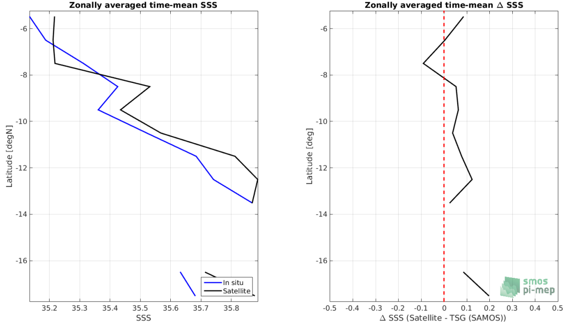
Figure 8: Left panel: Zonal mean SSS from SMOS SSS L3 v317 - 10 Days - 25 km (CATDS-CPDC) satellite product (black) and from TSG (SAMOS) (blue). Right panel: Zonal mean of \Delta\text{SSS} (Satellite - TSG (SAMOS)) for all the collected Pi-MEP match-up pairs estimated over the full satellite product period.
