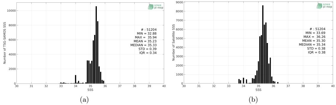
Figure 2: Histograms of SSS from TSG-SAMOS (a) and SMOS L3 v317 - 10 Days - 25 km (CATDS-CPDC) (b) considering all match-up pairs per bins of 0.1 over the OTT zone Pi-MEP region and for the full satellite product period.
