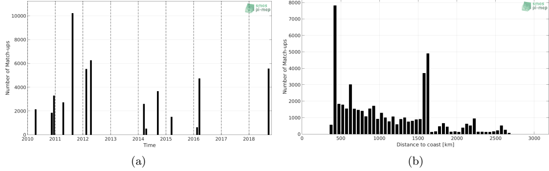
Figure 1: Number of match-ups between TSG-SAMOS and SMOS L3 v317 - 10 Days - 25 km (CATDS-CPDC) SSS as a function of time (a) and as function of the distance to coast (b) over the OTT zone Pi-MEP region and for the full satellite product period.
