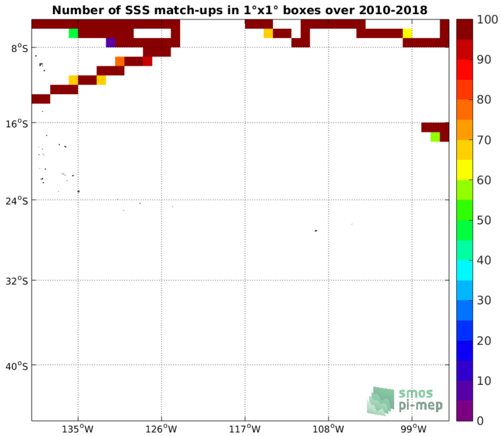
Figure 4: Number of SSS match-ups between TSG-SAMOS SSS and the SMOS L3 v317 - 10 Days - 25 km (CATDS-CPDC) SSS product for the OTT zone Pi-MEP region over 1°x1° boxes and for the full satellite product period.
