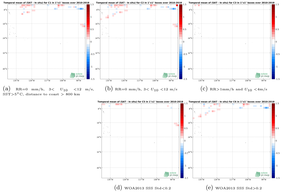
Figure 12: Temporal mean gridded over spatial boxes of size 1^\circ \times 1^\circ of \Delta SSS (SMOS L3 v317 - 10 Days - 25 km (CATDS-CPDC) - TSG-SAMOS) for 5 different subdatasets corresponding to:RR=0 mm/h, 3 < U_{10} < 12 m/s, SST >5^\circ C, distance to coast > 800 km (a), RR=0 mm/h, 3 < U_{10} < 12 m/s (b), RR >1 mm/h and U_{10} < 4 m/s (c), WOA2013 SSS Std <0.2 (d), WOA2013 SSS Std >0.2 (e).
