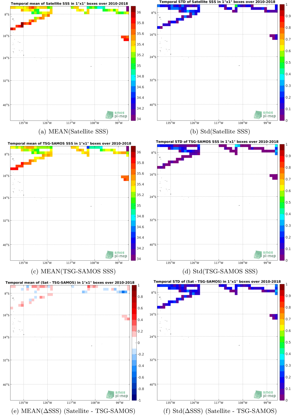
Figure 6: Temporal mean (left) and Std (right) of SSS from SMOS L3 v317 - 10 Days - 25 km (CATDS-CPDC) (top), TSG-SAMOS (middle), and of \Delta SSS (Satellite - TSG-SAMOS). Only match-up pairs are used to generate these maps.
