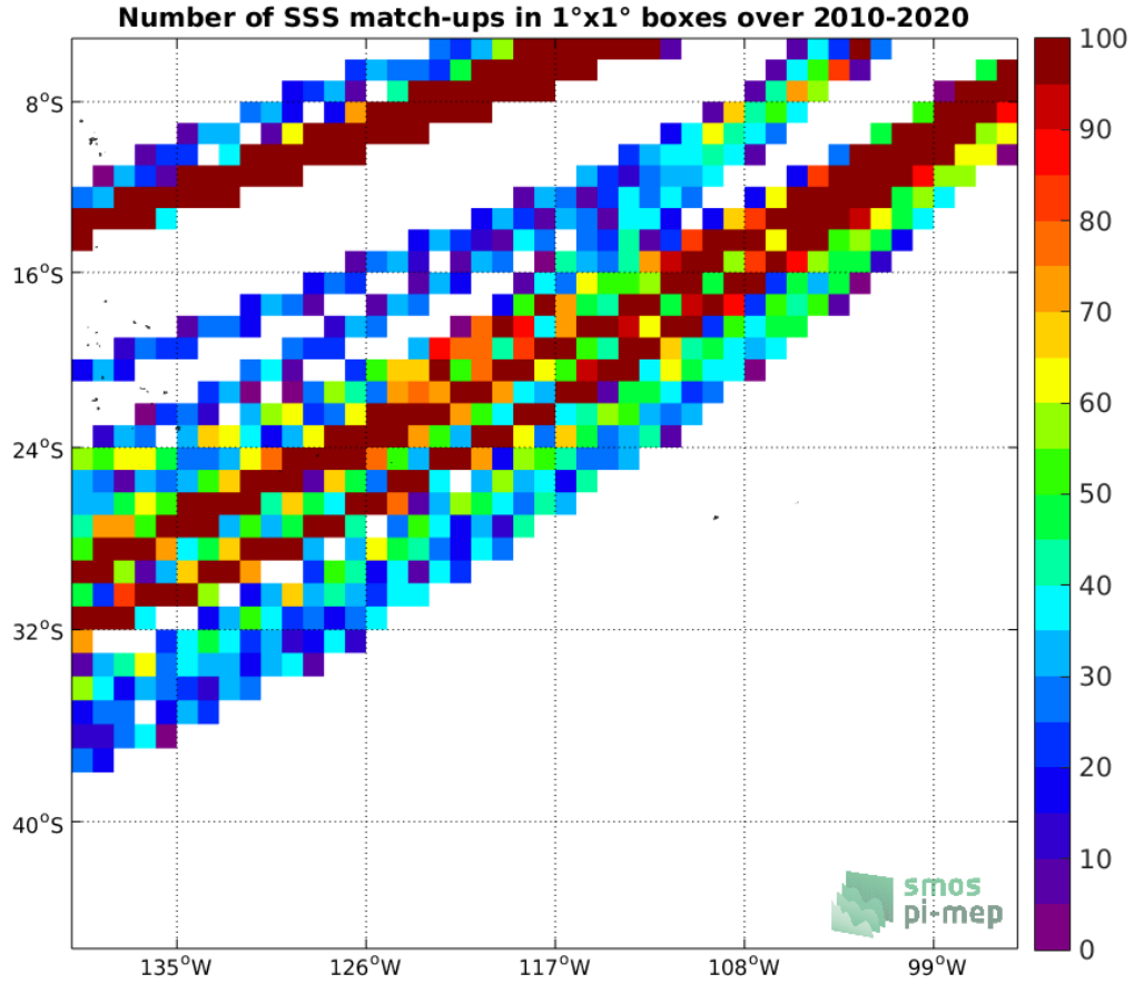
Figure 4: Number of SSS match-ups between TSG (LEGOS-DM) SSS and the SMOS SSS L3 v317 - 10 Days - 25 km (CATDS-CPDC) SSS product for the OTT zone Pi-MEP region over 1^\circ \times 1^\circ boxes and for the full satellite product period.
