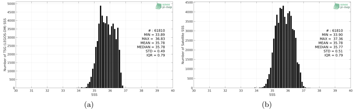
Figure 2: Histograms of SSS from TSG (LEGOS-DM) (a) and SMOS SSS L3 v317 - 10 Days - 25 km (CATDS-CPDC) (b) considering all match-up pairs per bins of 0.1 over the OTT zone Pi-MEP region and for the full satellite product period.
