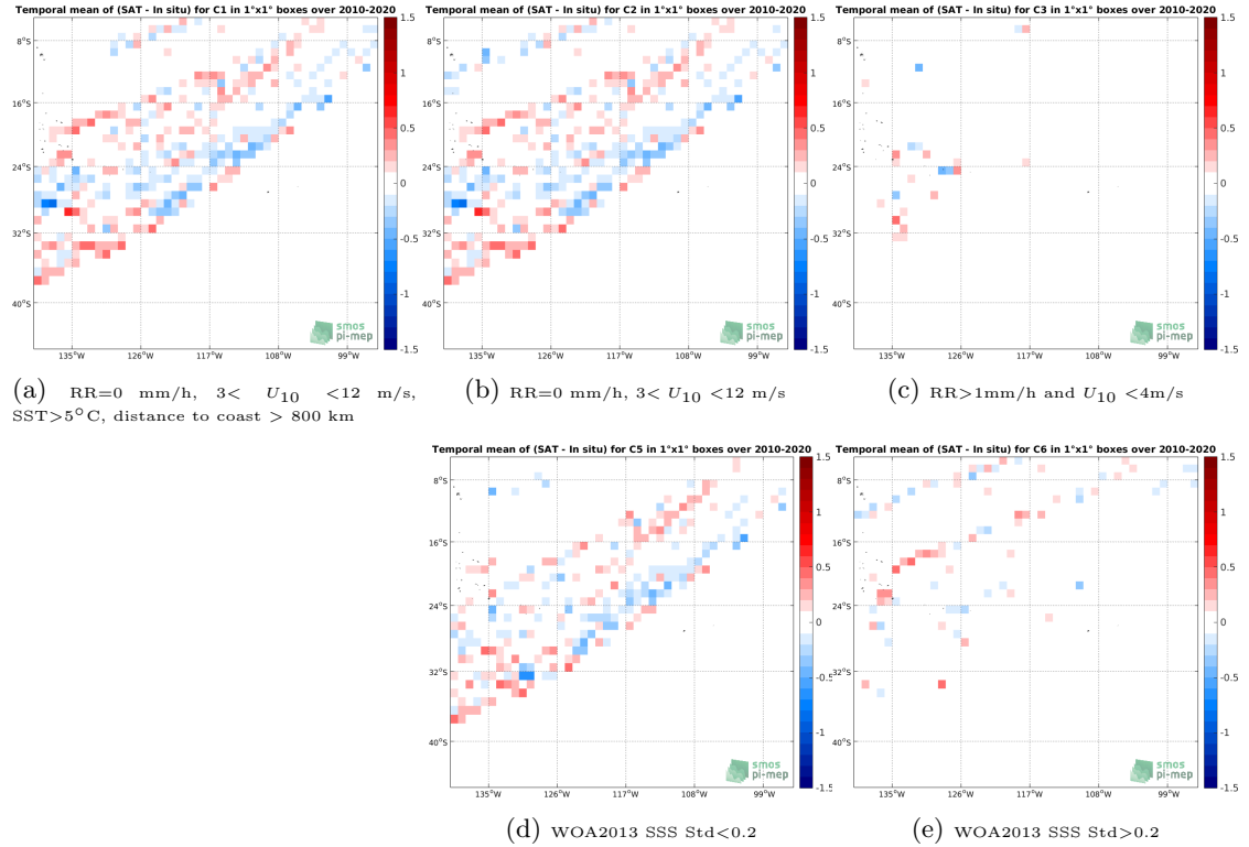
Figure 12: Temporal mean gridded over spatial boxes of size 1^{\circ}\times 1^{\circ} of \Delta\text{SSS} (SMOS SSS L3 v317 - 10 Days - 25 km (CATDS-CPDC) - TSG (LEGOS-DM)) for 5 different subdatasets corresponding to: RR=0 mm/h, 3 < U_{10} < 12 m/s, SST >5^{\circ}\text{C} , distance to coast > 800 km (a), RR=0 mm/h, 3 < U_{10} < 12 m/s (b), RR >1 mm/h and U_{10} < 4 m/s (c), WOA2013 SSS Std <0.2 (d), WOA2013 SSS Std >0.2 (e).
