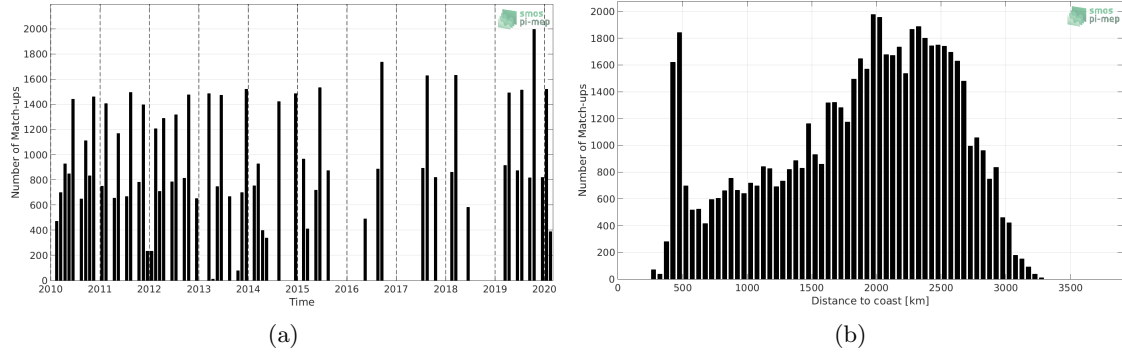
Figure 1: Number of match-ups between TSG (LEGOS-DM) and SMOS SSS L3 v317 - 10 Days - 25 km (CATDS-CPDC) SSS as a function of time (a) and as function of the distance to coast (b) over the OTT zone Pi-MEP region and for the full satellite product period.
