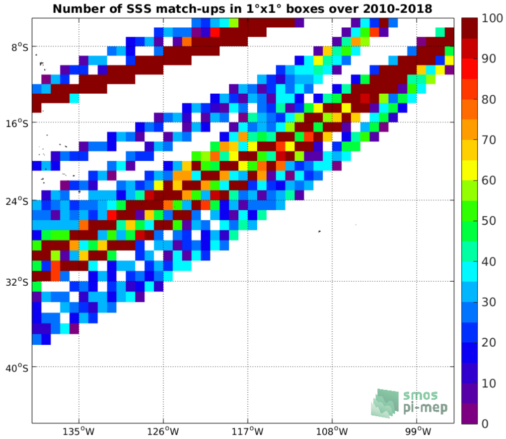
Figure 4: Number of SSS match-ups between TSG (LEGOS-DM) SSS and the SMOS SSS L3 v317 - 10 Days - 25 km (CATDS-CPDC) SSS product for the OTT zone Pi-MEP region over 1°x1° boxes and for the full satellite product period.
