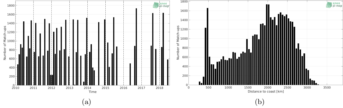
Figure 1: Number of match-ups between TSG-LEGOS-DM and SMOS L3 v317 - 10 Days - 25 km (CATDS-CPDC) SSS as a function of time (a) and as function of the distance to coast (b) over the OTT zone Pi-MEP region and for the full satellite product period.
