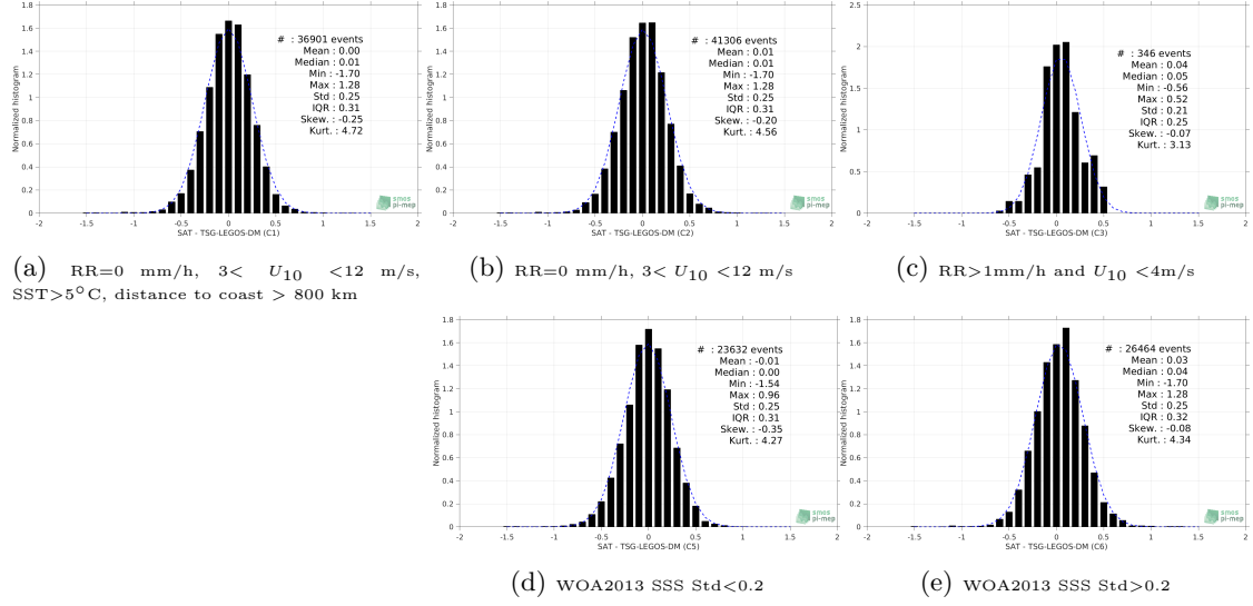
Figure 13: Normalized histogram of \Delta\text{SSS} (SMOS L3 v317 - 10 Days - 25 km (CATDS-CPDC) - TSG-LEGOS-DM) for 5 different subdatasets corresponding to: RR=0 mm/h, 3 < U_{10} < 12 m/s, SST >5^{\circ}\text{C} , distance to coast > 800 km (a), RR=0 mm/h, 3 < U_{10} < 12 m/s (b), RR>1\text{mm/h} and U_{10} < 4\text{m/s} (c), WOA2013 SSS Std <0.2 (d), WOA2013 SSS Std >0.2 (e).
