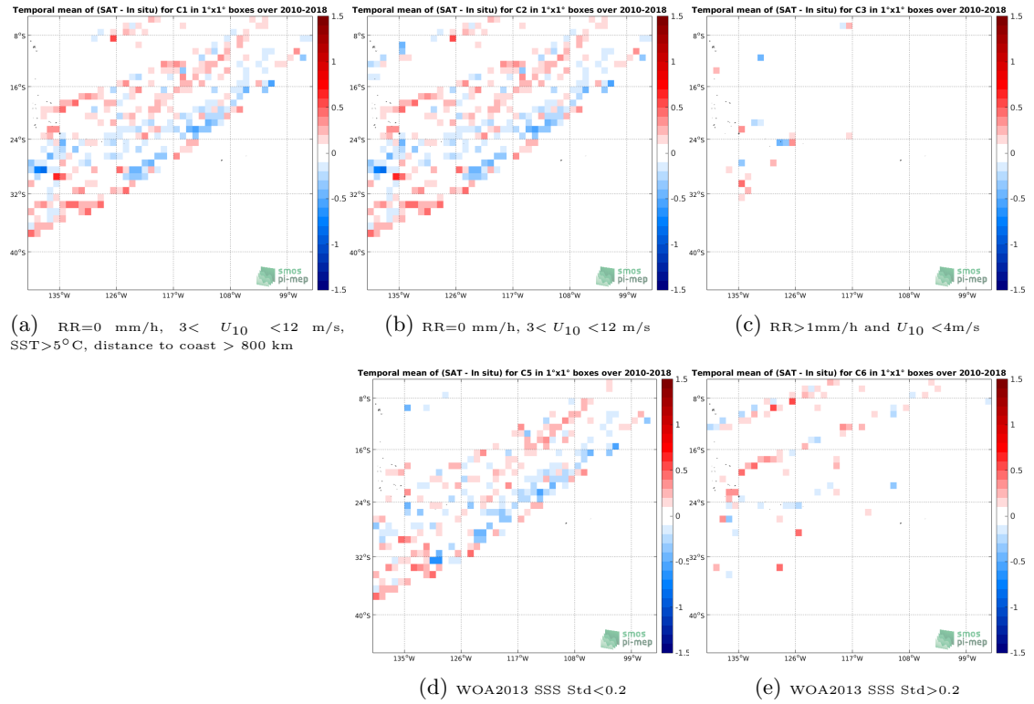
Figure 12: Temporal mean gridded over spatial boxes of size 1^\circ \times 1^\circ of \Delta SSS (SMOS L3 v317 - 10 Days - 25 km (CATDS-CPDC) - TSG-LEGOS-DM) for 5 different subdatasets corresponding to:RR=0 mm/h, 3 < U_{10} < 12 m/s, SST >5^\circ\text{C} , distance to coast > 800 km (a), RR=0 mm/h, 3 < U_{10} < 12 m/s (b), RR >1 mm/h and U_{10} < 4 m/s (c), WOA2013 SSS Std <0.2 (d), WOA2013 SSS Std >0.2 (e).
