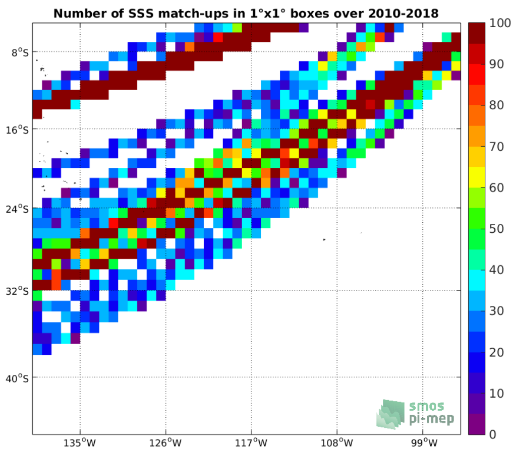
Figure 4: Number of SSS match-ups between TSG-LEGOS-DM SSS and the SMOS L3 v317 - 10 Days - 25 km (CATDS-CPDC) SSS product for the OTT zone Pi-MEP region over 1°x1° boxes and for the full satellite product period.
