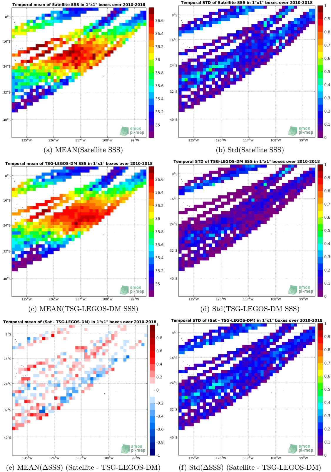
Figure 6: Temporal mean (left) and Std (right) of SSS from SMOS-L3-CATDS-CPDC-V317-10DAYS-25KM (top), TSG-LEGOS-DM (middle), and of \Delta SSS (Satellite - TSG-LEGOS-DM). Only match-up pairs are used to generate these maps.
