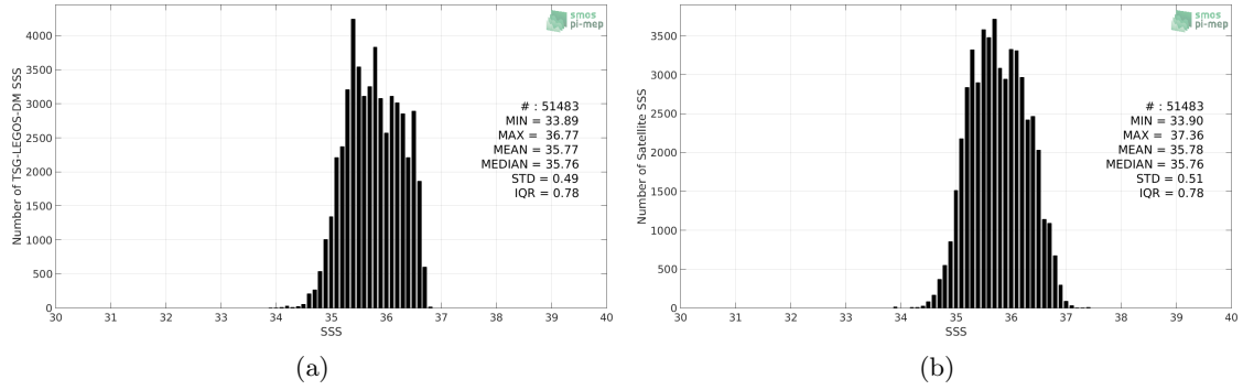
Figure 2: Histograms of SSS from TSG-LEGOS-DM (a) and SMOS-L3-CATDS-CPDC-V317-10DAYS-25KM (b) considering all match-up pairs per bins of 0.1 over the OTT zone Pi-MEP region and for the full satellite product period.
