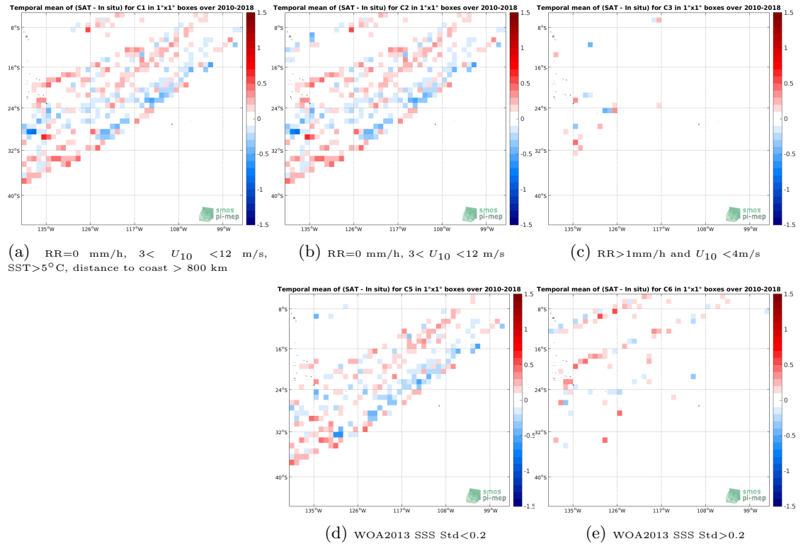
Figure 12: Temporal mean gridded over spatial boxes of size 1^\circ \times 1^\circ of \Delta SSS (SMOS-L3-CATDS-CPDC-V317-10DAYS-25KM - TSG-LEGOS-DM) for 5 different subdatasets corresponding to:RR=0 mm/h, 3 < U_{10} < 12 m/s, SST >5^\circ C, distance to coast > 800 km (a), RR=0 mm/h, 3 < U_{10} < 12 m/s (b), RR >1 mm/h and U_{10} < 4 m/s (c), WOA2013 SSS Std <0.2 (d), WOA2013 SSS Std >0.2 (e).
