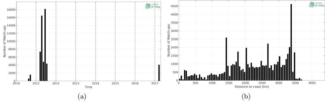
Figure 1: Number of match-ups between TSG (GOSUD-Sailing-ship) and SMOS SSS L3 v317 - 10 Days - 25 km (CATDS-CPDC) SSS as a function of time (a) and as function of the distance to coast (b) over the OTT zone Pi-MEP region and for the full satellite product period.
