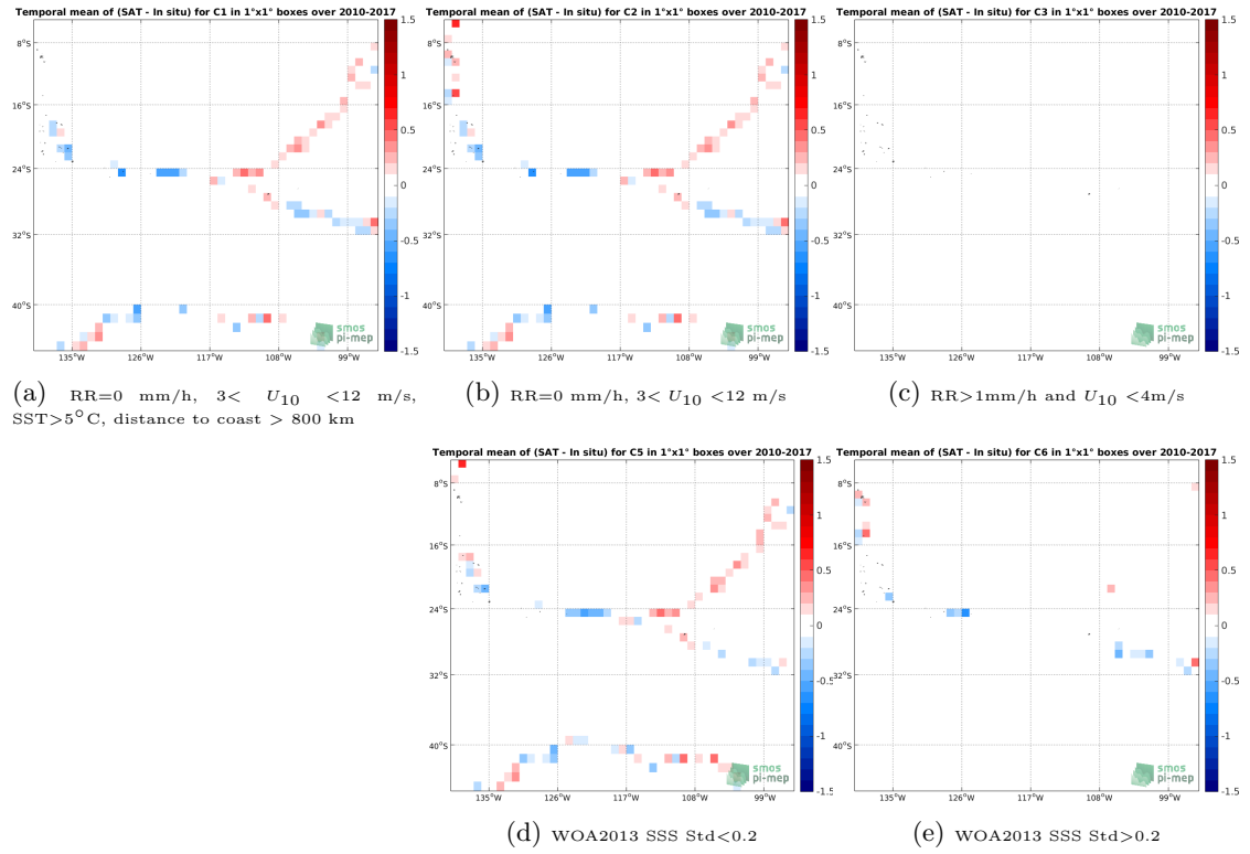
Figure 12: Temporal mean gridded over spatial boxes of size 1^\circ \times 1^\circ of \Delta SSS (SMOS SSS L3 v317 - 10 Days - 25 km (CATDS-CPDC) - TSG (GOSUD-Sailing-ship)) for 5 different subdatasets corresponding to: RR=0 mm/h, 3 < U_{10} < 12 m/s, SST > 5^\circ C , distance to coast > 800 km (a), RR=0 mm/h, 3 < U_{10} < 12 m/s (b), RR > 1 mm/h and U_{10} < 4 m/s (c), WOA2013 SSS Std < 0.2 (d), WOA2013 SSS Std > 0.2 (e).
