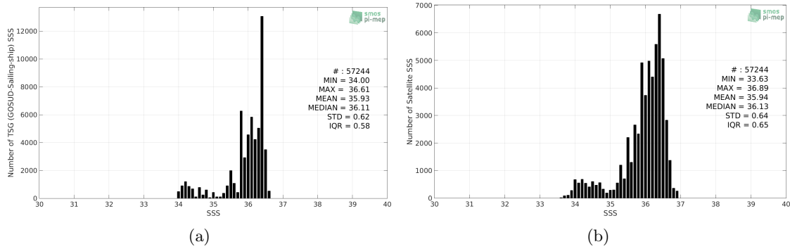
Figure 2: Histograms of SSS from TSG (GOSUD-Sailing-ship) (a) and SMOS SSS L3 v317 - 10 Days - 25 km (CATDS-CPDC) (b) considering all match-up pairs per bins of 0.1 over the OTT zone Pi-MEP region and for the full satellite product period.
