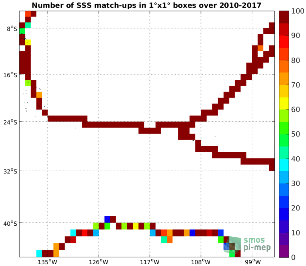
Figure 4: Number of SSS match-ups between TSG (GOSUD-Sailing-ship) SSS and the SMOS SSS L3 v317 - 10 Days - 25 km (CATDS-CPDC) SSS product for the OTT zone Pi-MEP region over 1°x1° boxes and for the full satellite product period.
