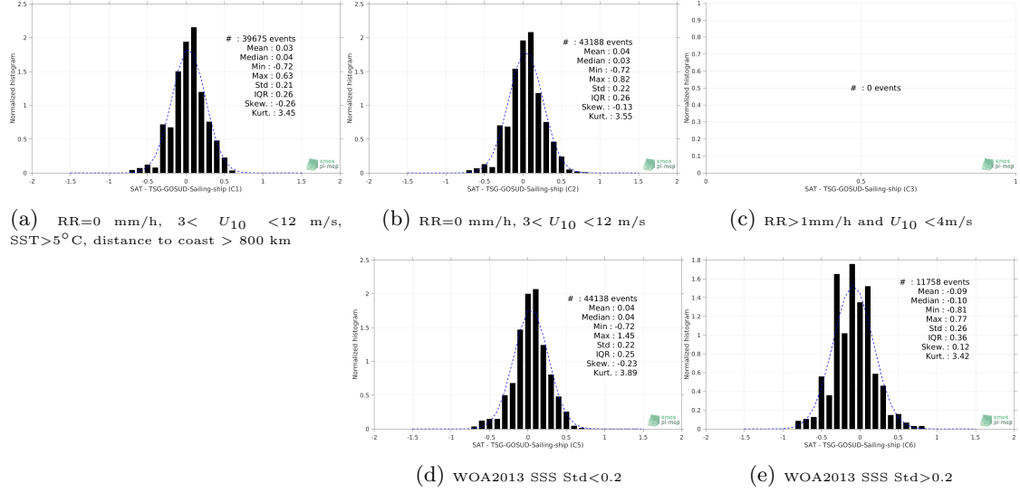
Figure 13: Normalized histogram of \Delta\text{SSS} (SMOS L3 v317 - 10 Days - 25 km (CATDS-CPDC) - TSG-GOSUD-Sailing-ship) for 5 different subdatasets corresponding to: RR=0 mm/h, 3 < U_{10} < 12 m/s, SST > 5^\circ\text{C} , distance to coast > 800 km (a), RR=0 mm/h, 3 < U_{10} < 12 m/s (b), RR > 1\text{mm/h} and U_{10} < 4\text{m/s} (c), WOA2013 SSS Std < 0.2 (d), WOA2013 SSS Std > 0.2 (e).
