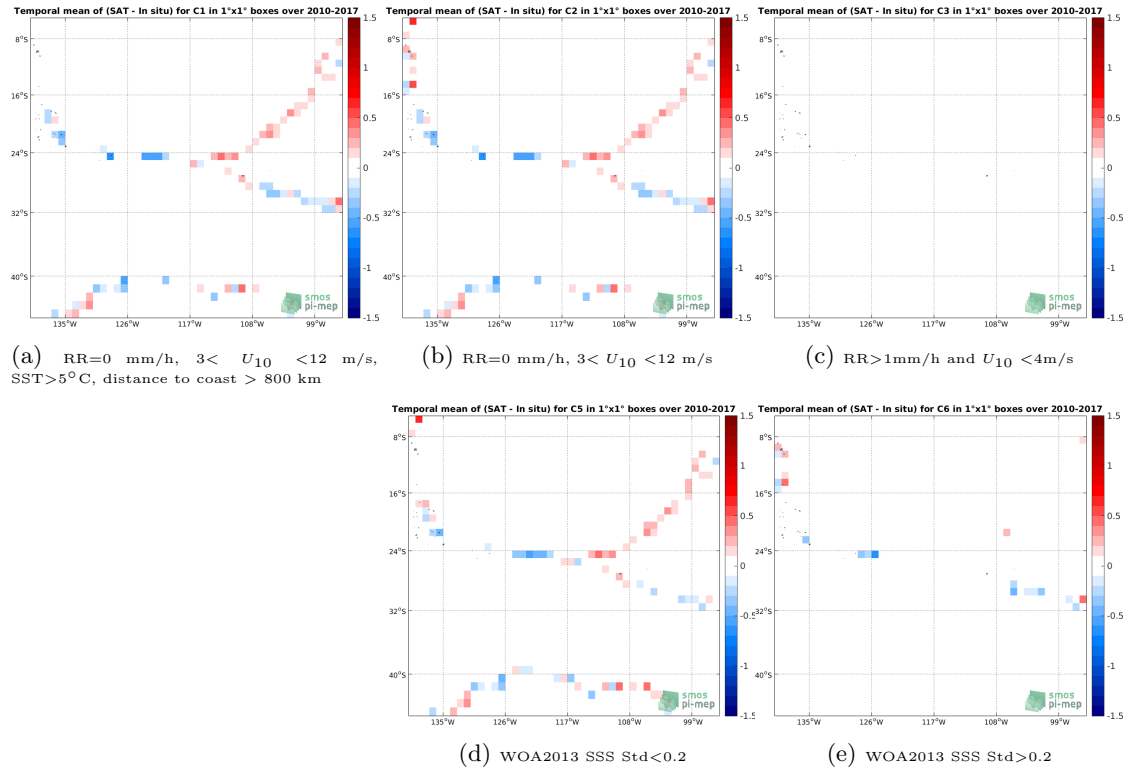
Figure 12: Temporal mean gridded over spatial boxes of size 1^\circ \times 1^\circ of \Delta SSS (SMOS L3 v317 - 10 Days - 25 km (CATDS-CPDC) - TSG-GOSUD-Sailing-ship) for 5 different subdatasets corresponding to: RR=0 mm/h, 3 < U_{10} < 12 m/s, SST >5^\circ\text{C} , distance to coast > 800 km (a), RR=0 mm/h, 3 < U_{10} < 12 m/s (b), RR >1 mm/h and U_{10} < 4 m/s (c), WOA2013 SSS Std <0.2 (d), WOA2013 SSS Std >0.2 (e).
