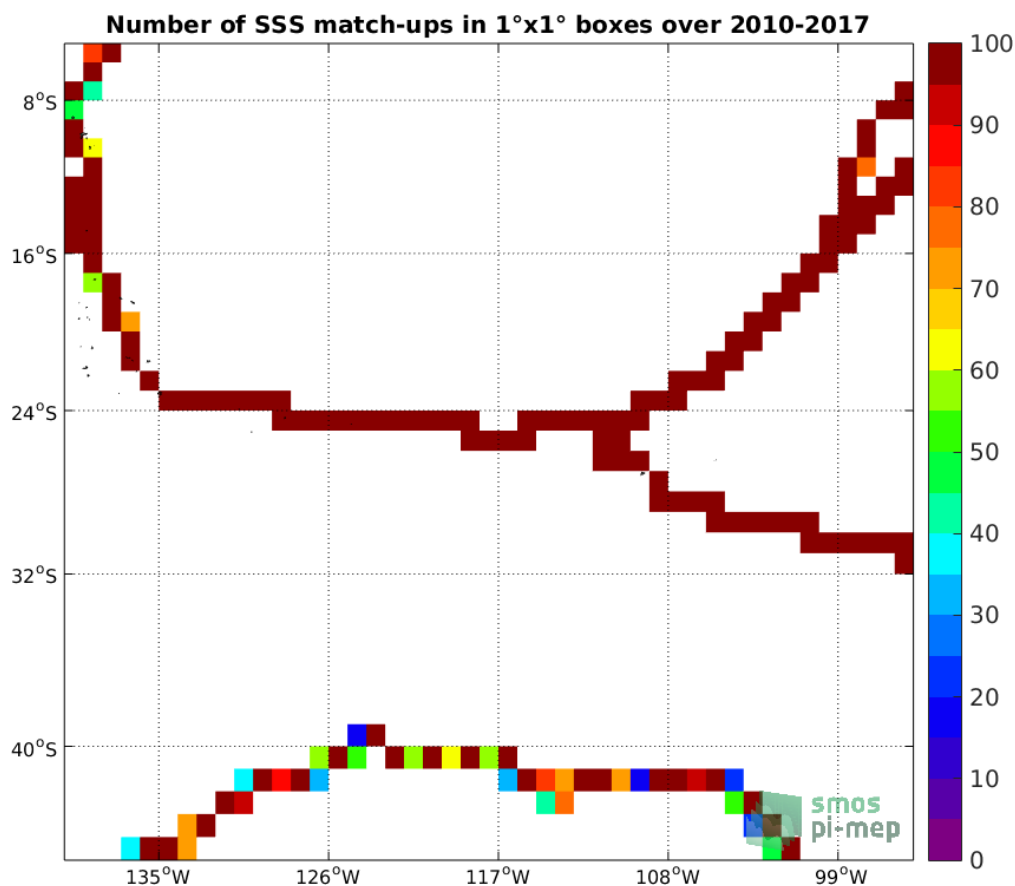
Figure 4: Number of SSS match-ups between TSG-GOSUD-Sailing-ship SSS and the SMOS L3 v317 - 10 Days - 25 km (CATDS-CPDC) SSS product for the OTT zone Pi-MEP region over 1°x1° boxes and for the full satellite product period.
