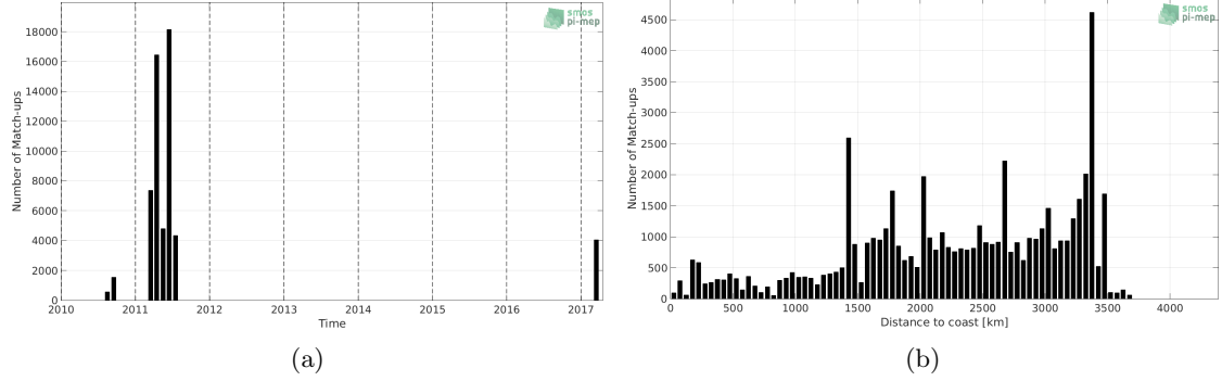
Figure 1: Number of match-ups between TSG-GOSUD-Sailing-ship and SMOS L3 v317 - 10 Days - 25 km (CATDS-CPDC) SSS as a function of time (a) and as function of the distance to coast (b) over the OTT zone Pi-MEP region and for the full satellite product period.
