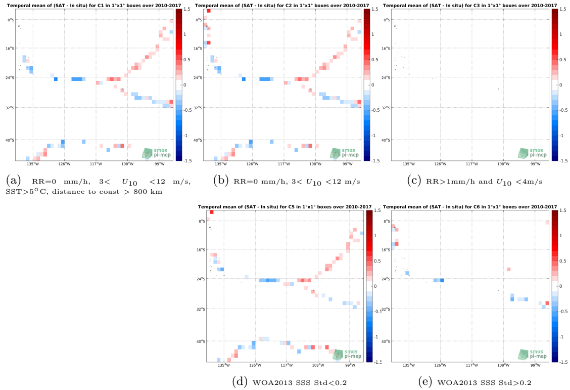
Figure 12: Temporal mean gridded over spatial boxes of size 1^\circ \times 1^\circ of \Delta SSS (SMOS-L3-CATDS-CPDC-V317-10DAYS-25KM - TSG-GOSUD-Sailing-ship) for 5 different subdatasets corresponding to: RR=0 mm/h, 3 < U_{10} < 12 m/s, SST >5^\circ\text{C} , distance to coast > 800 km (a), RR=0 mm/h, 3 < U_{10} < 12 m/s (b), RR >1 mm/h and U_{10} < 4 m/s (c), WOA2013 SSS Std <0.2 (d), WOA2013 SSS Std >0.2 (e).
