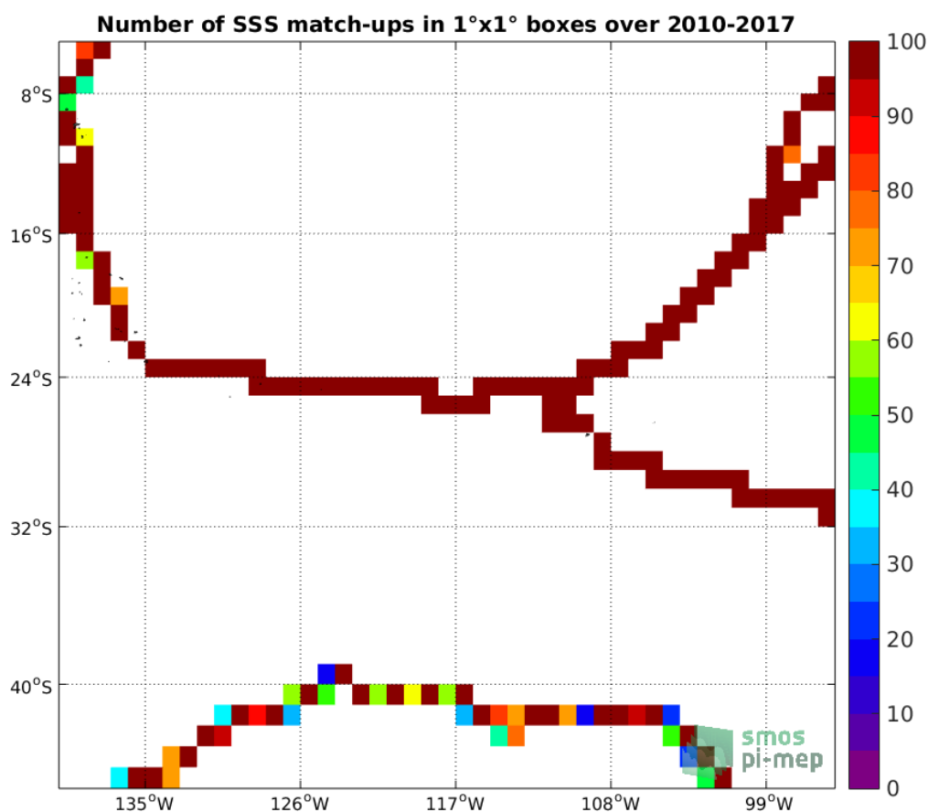
Figure 4: Number of SSS match-ups between TSG-GOSUD-Sailing-ship SSS and the SMOS-L3-CATDS-CPDC-V317-10DAYS-25KM SSS product for the OTT zone Pi-MEP region over 1°x1° boxes and for the full satellite product period.
