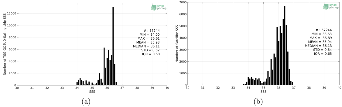
Figure 2: Histograms of SSS from TSG-GOSUD-Sailing-ship (a) and SMOS-L3-CATDS-CPDC-V317-10DAYS-25KM (b) considering all match-up pairs per bins of 0.1 over the OTT zone Pi-MEP region and for the full satellite product period.
