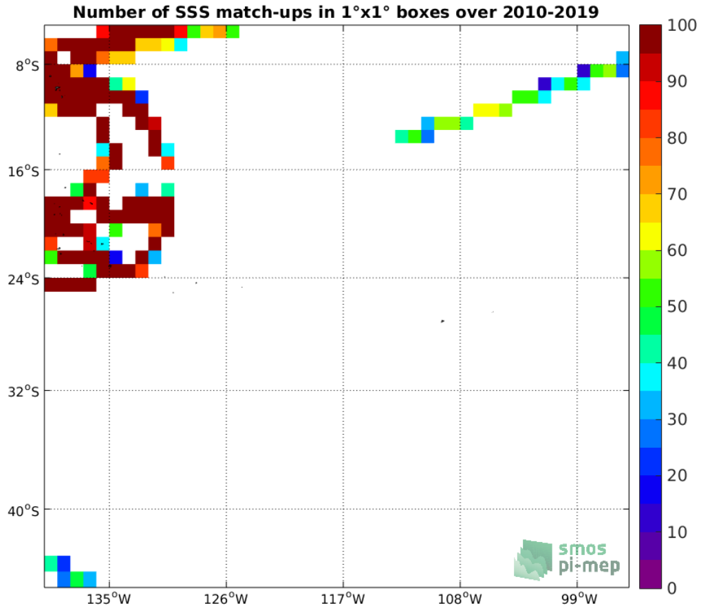
Figure 4: Number of SSS match-ups between TSG (GOSUD-Research-vessel) SSS and the SMOS SSS L3 v317 - 10 Days - 25 km (CATDS-CPDC) SSS product for the OTT zone Pi-MEP region over 1^\circ \times 1^\circ boxes and for the full satellite product period.
