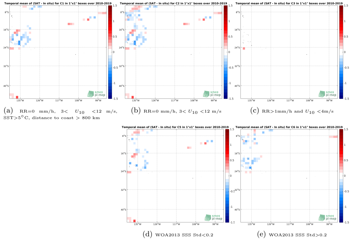
Figure 12: Temporal mean gridded over spatial boxes of size 1^\circ \times 1^\circ of \Delta SSS (SMOS SSS L3 v317 - 10 Days - 25 km (CATDS-CPDC) - TSG (GOSUD-Research-vessel)) for 5 different subdatasets corresponding to: RR=0 mm/h, 3 < U_{10} < 12 m/s, SST > 5^\circ C , distance to coast > 800 km (a), RR=0 mm/h, 3 < U_{10} < 12 m/s (b), RR > 1 mm/h and U_{10} < 4 m/s (c), WOA2013 SSS Std < 0.2 (d), WOA2013 SSS Std > 0.2 (e).
