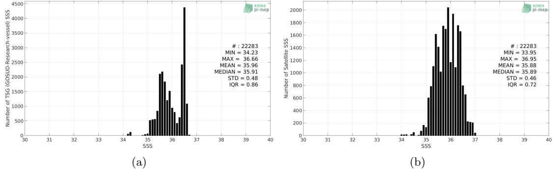
Figure 2: Histograms of SSS from TSG (GOSUD-Research-vessel) (a) and SMOS SSS L3 v317 - 10 Days - 25 km (CATDS-CPDC) (b) considering all match-up pairs per bins of 0.1 over the OTT zone Pi-MEP region and for the full satellite product period.
