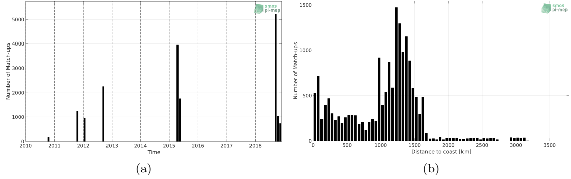
Figure 1: Number of match-ups between TSG-GOSUD-Research-vessel and SMOS L3 v317 - 10 Days - 25 km (CATDS-CPDC) SSS as a function of time (a) and as function of the distance to coast (b) over the OTT zone Pi-MEP region and for the full satellite product period.
