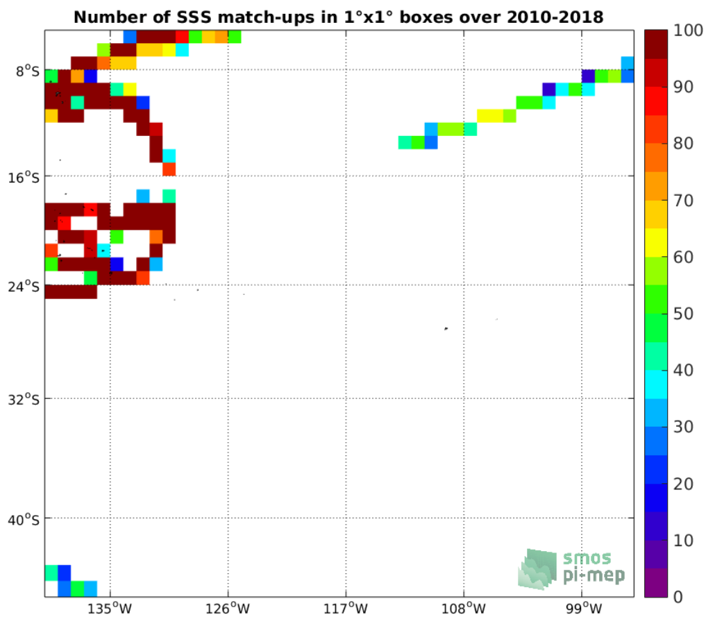
Figure 4: Number of SSS match-ups between TSG-GOSUD-Research-vessel SSS and the SMOS L3 v317 - 10 Days - 25 km (CATDS-CPDC) SSS product for the OTT zone Pi-MEP region over 1°x1° boxes and for the full satellite product period.
