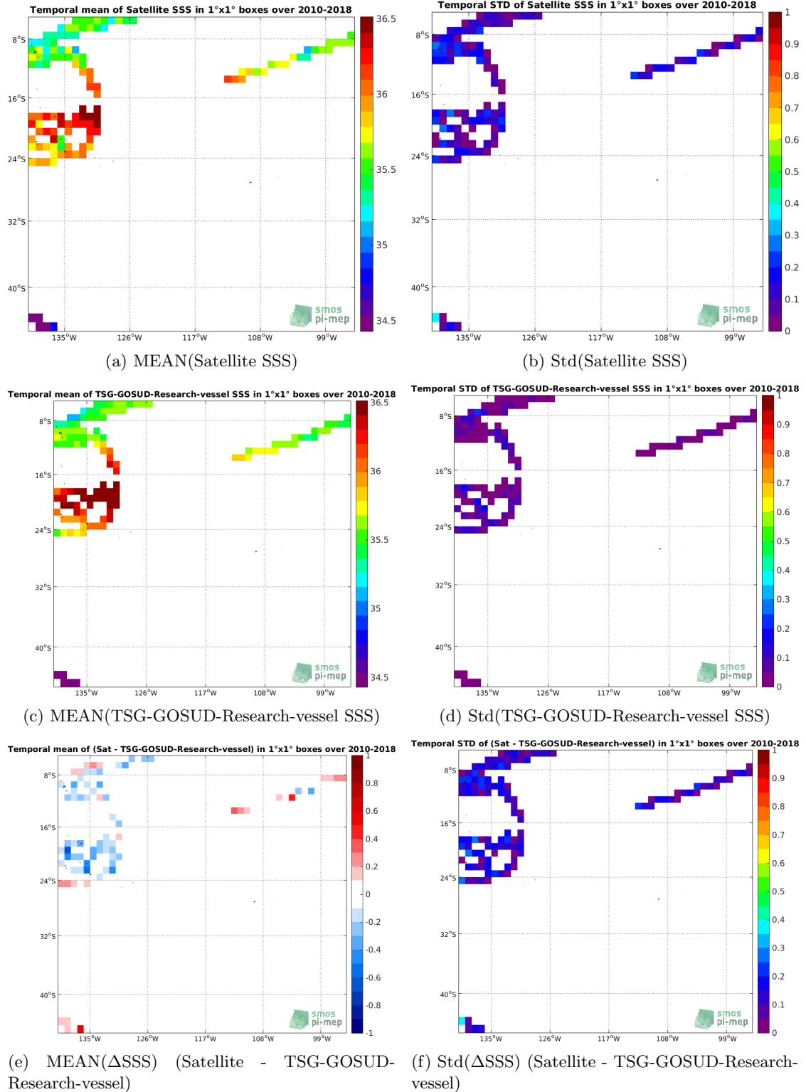
Figure 6: Temporal mean (left) and Std (right) of SSS from SMOS L3 v317 - 10 Days - 25 km (CATDS-CPDC) (top), TSG-GOSUD-Research-vessel (middle), and of \Delta SSS (Satellite - TSG-GOSUD-Research-vessel). Only match-up pairs are used to generate these maps.
