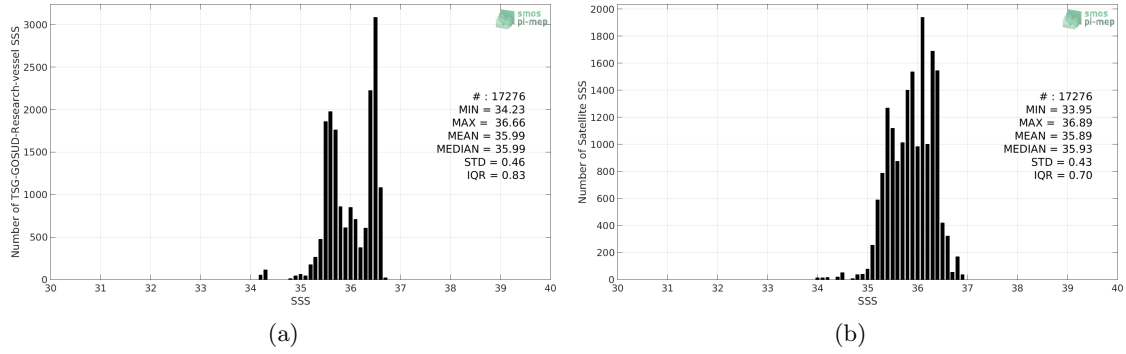
Figure 2: Histograms of SSS from TSG-GOSUD-Research-vessel (a) and SMOS L3 v317 - 10 Days - 25 km (CATDS-CPDC) (b) considering all match-up pairs per bins of 0.1 over the OTT zone Pi-MEP region and for the full satellite product period.
