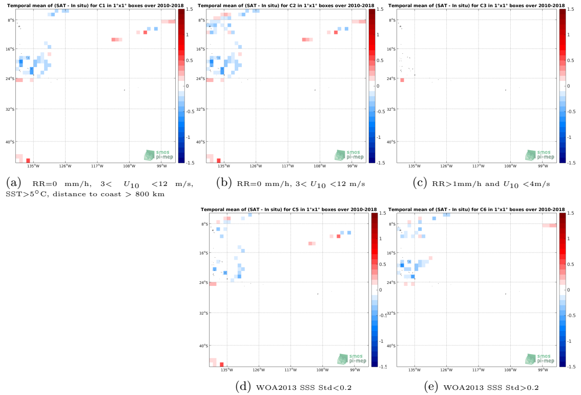
Figure 12: Temporal mean gridded over spatial boxes of size 1^\circ \times 1^\circ of \Delta SSS (SMOS L3 v317 - 10 Days - 25 km (CATDS-CPDC) - TSG-GOSUD-Research-vessel) for 5 different subdatasets corresponding to:RR=0 mm/h, 3 < U_{10} < 12 m/s, SST >5^\circ\text{C} , distance to coast > 800 km (a), RR=0 mm/h, 3 < U_{10} < 12 m/s (b), RR >1 mm/h and U_{10} < 4 m/s (c), WOA2013 SSS Std <0.2 (d), WOA2013 SSS Std >0.2 (e).
