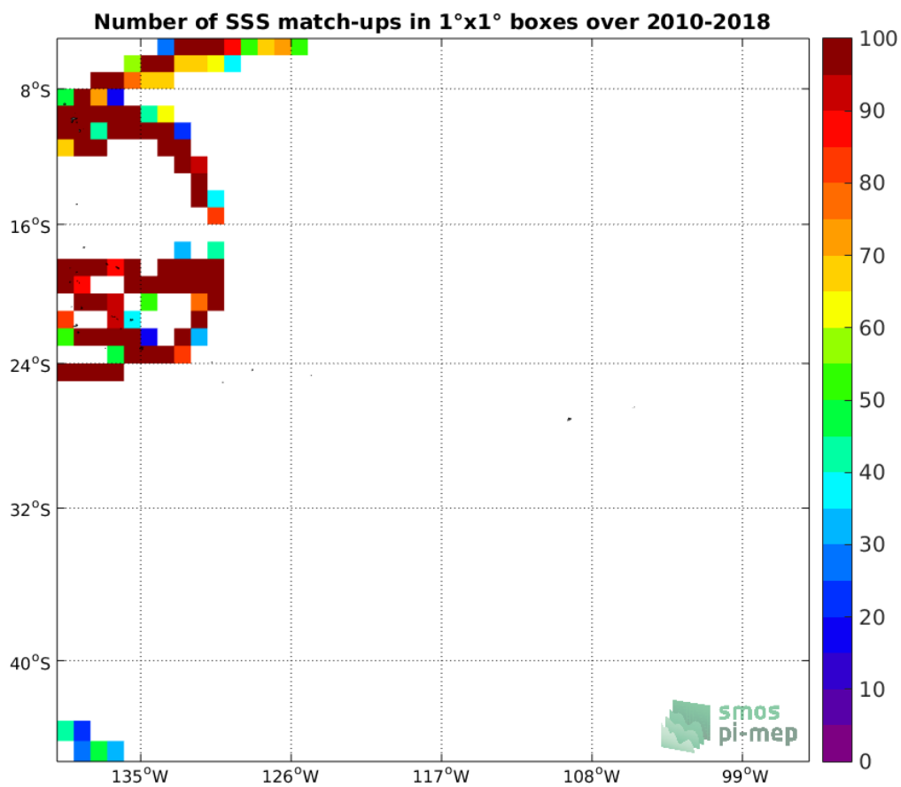
Figure 4: Number of SSS match-ups between TSG-GOSUD-Research-vessel SSS and the SMOS-L3-CATDS-CPDC-V317-10DAYS-25KM SSS product for the OTT zone Pi-MEP region over 1°x1° boxes and for the full satellite product period.
