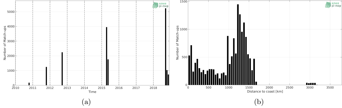
Figure 1: Number of match-ups between TSG-GOSUD-Research-vessel and SMOS-L3-CATDS-CPDC-V317-10DAYS-25KM SSS as a function of time (a) and as function of the distance to coast (b) over the OTT zone Pi-MEP region and for the full satellite product period.
