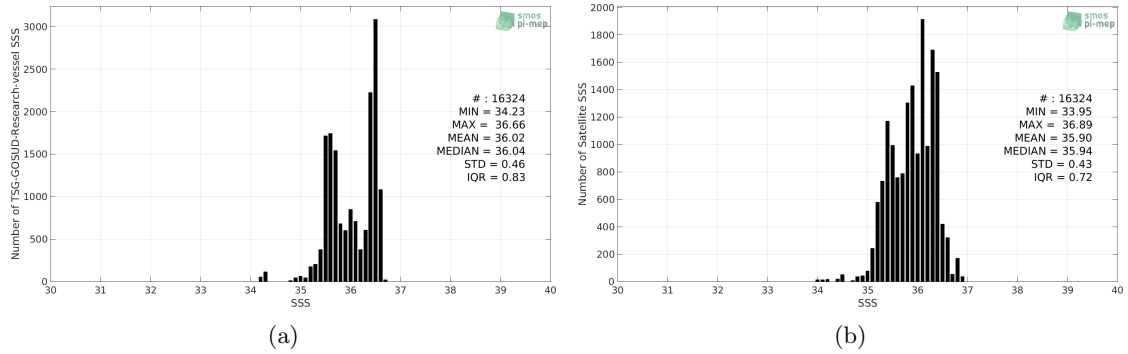
Figure 2: Histograms of SSS from TSG-GOSUD-Research-vessel (a) and SMOS-L3-CATDS-CPDC-V317-10DAYS-25KM (b) considering all match-up pairs per bins of 0.1 over the OTT zone Pi-MEP region and for the full satellite product period.
