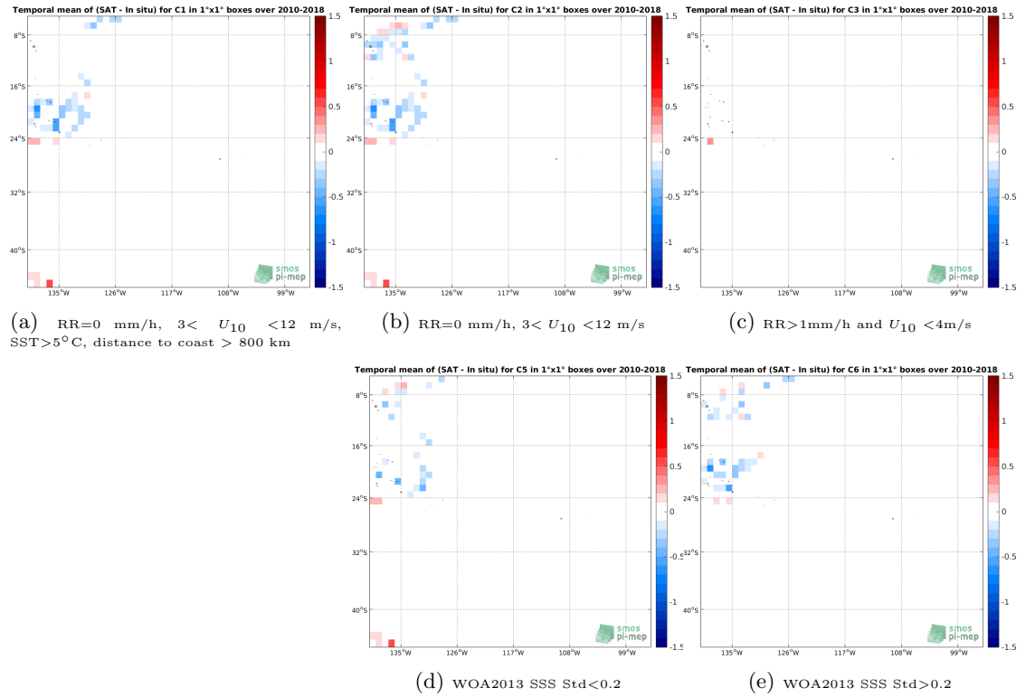
Figure 12: Temporal mean gridded over spatial boxes of size 1^\circ \times 1^\circ of \Delta SSS (SMOS-L3-CATDS-CPDC-V317-10DAYS-25KM - TSG-GOSUD-Research-vessel) for 5 different subdatasets corresponding to:RR=0 mm/h, 3 < U_{10} < 12 m/s, SST >5^\circ\text{C} , distance to coast > 800 km (a), RR=0 mm/h, 3 < U_{10} < 12 m/s (b), RR >1 mm/h and U_{10} < 4 m/s (c), WOA2013 SSS Std <0.2 (d), WOA2013 SSS Std >0.2 (e).
