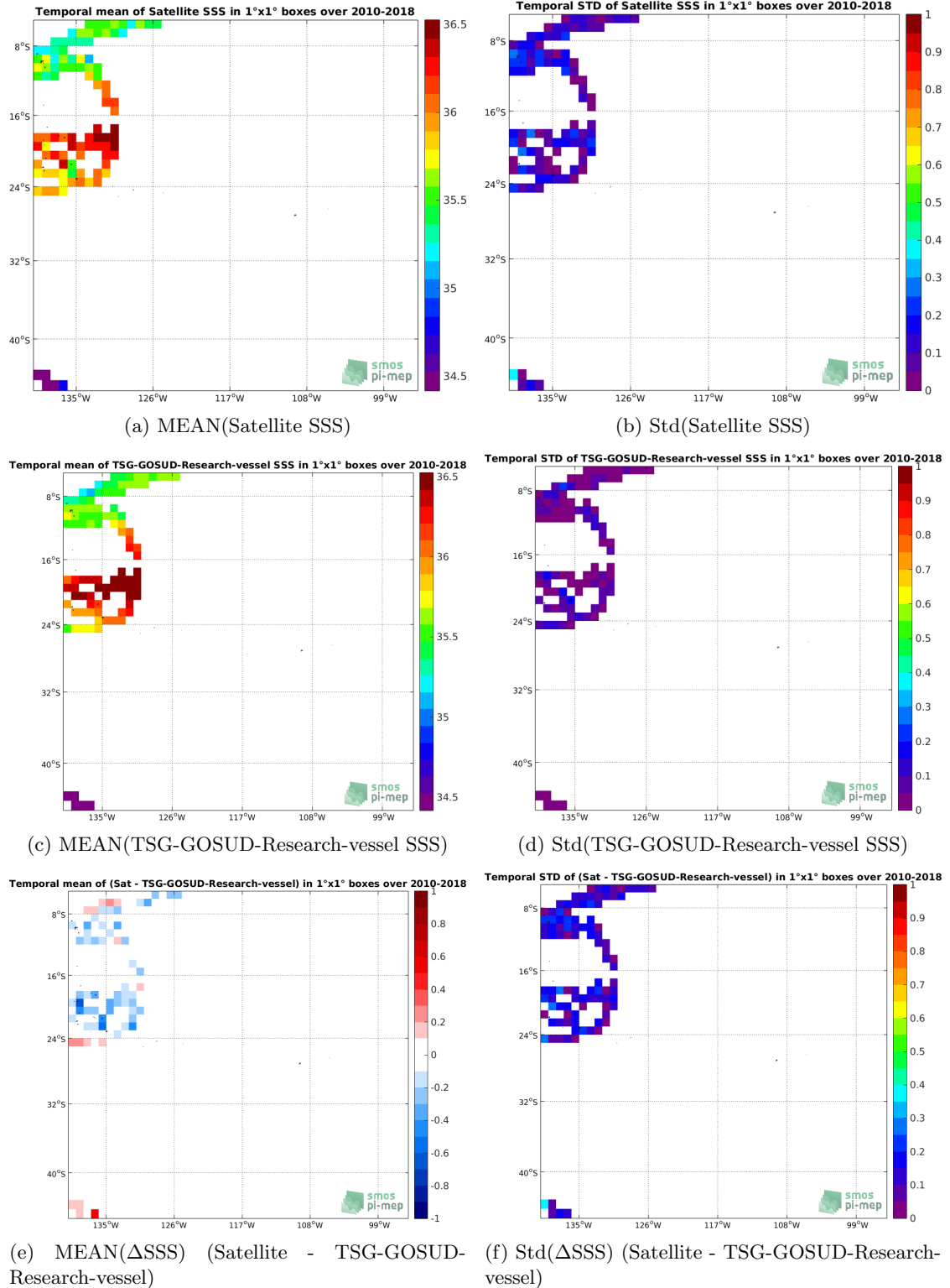
Figure 6: Temporal mean (left) and Std (right) of SSS from SMOS-L3-CATDS-CPDC-V317-10DAYS-25KM (top), TSG-GOSUD-Research-vessel (middle), and of \Delta SSS (Satellite - TSG-GOSUD-Research-vessel). Only match-up pairs are used to generate these maps.
