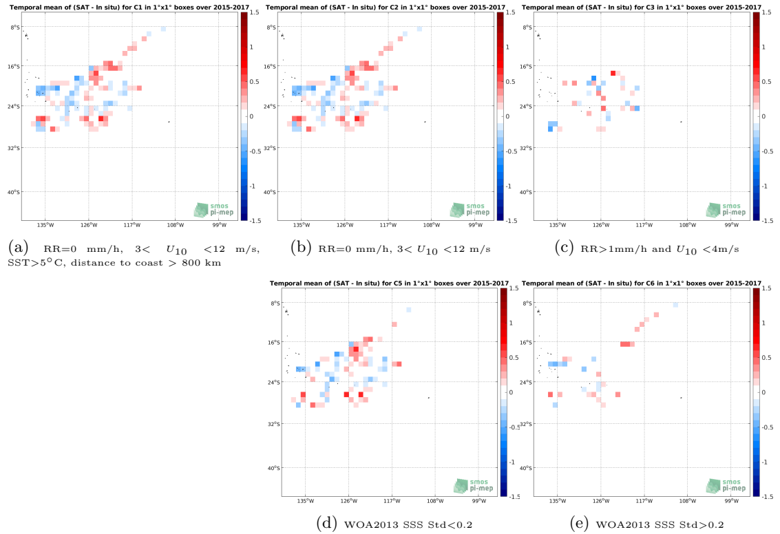
Figure 11: Temporal mean gridded over spatial boxes of size 1^\circ \times 1^\circ of \Delta SSS (SMOS SSS L3 v317 - 10 Days - 25 km (CATDS-CPDC) - Surface drifters) for 5 different subdatasets corresponding to: RR=0 mm/h, 3 < U_{10} < 12 m/s, SST > 5^\circ C , distance to coast > 800 km (a), RR=0 mm/h, 3 < U_{10} < 12 m/s (b), RR > 1 mm/h and U_{10} < 4 m/s (c), WOA2013 SSS Std < 0.2 (d), WOA2013 SSS Std > 0.2 (e).
