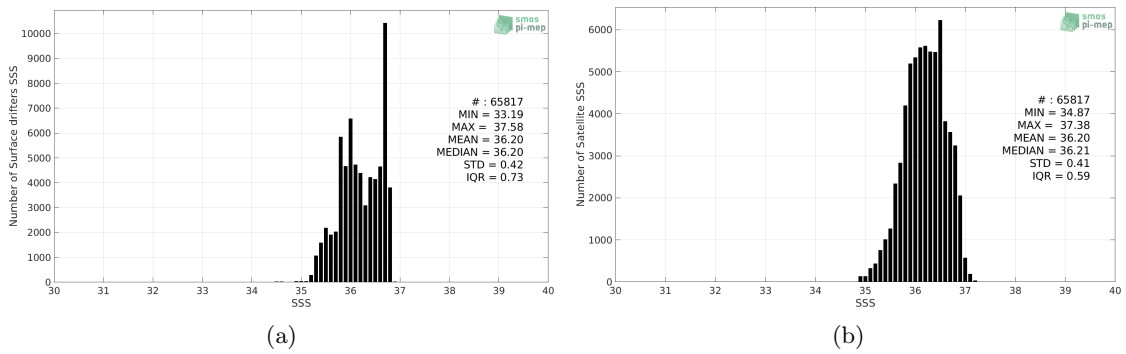
Figure 2: Histograms of SSS from Surface drifters (a) and SMOS SSS L3 v317 - 10 Days - 25 km (CATDS-CPDC) (b) considering all match-up pairs per bins of 0.1 over the OTT zone Pi-MEP region and for the full satellite product period.
