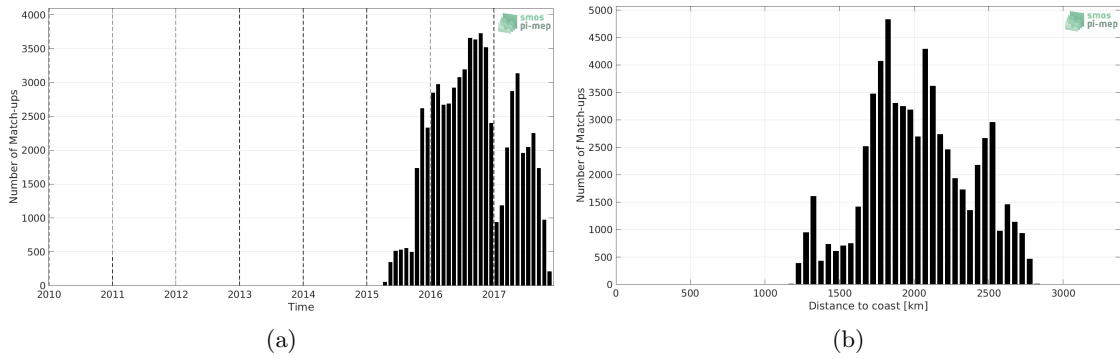
Figure 1: Number of match-ups between Surface drifters and SMOS SSS L3 v317 - 10 Days - 25 km (CATDS-CPDC) SSS as a function of time (a) and as function of the distance to coast (b) over the OTT zone Pi-MEP region and for the full satellite product period.
