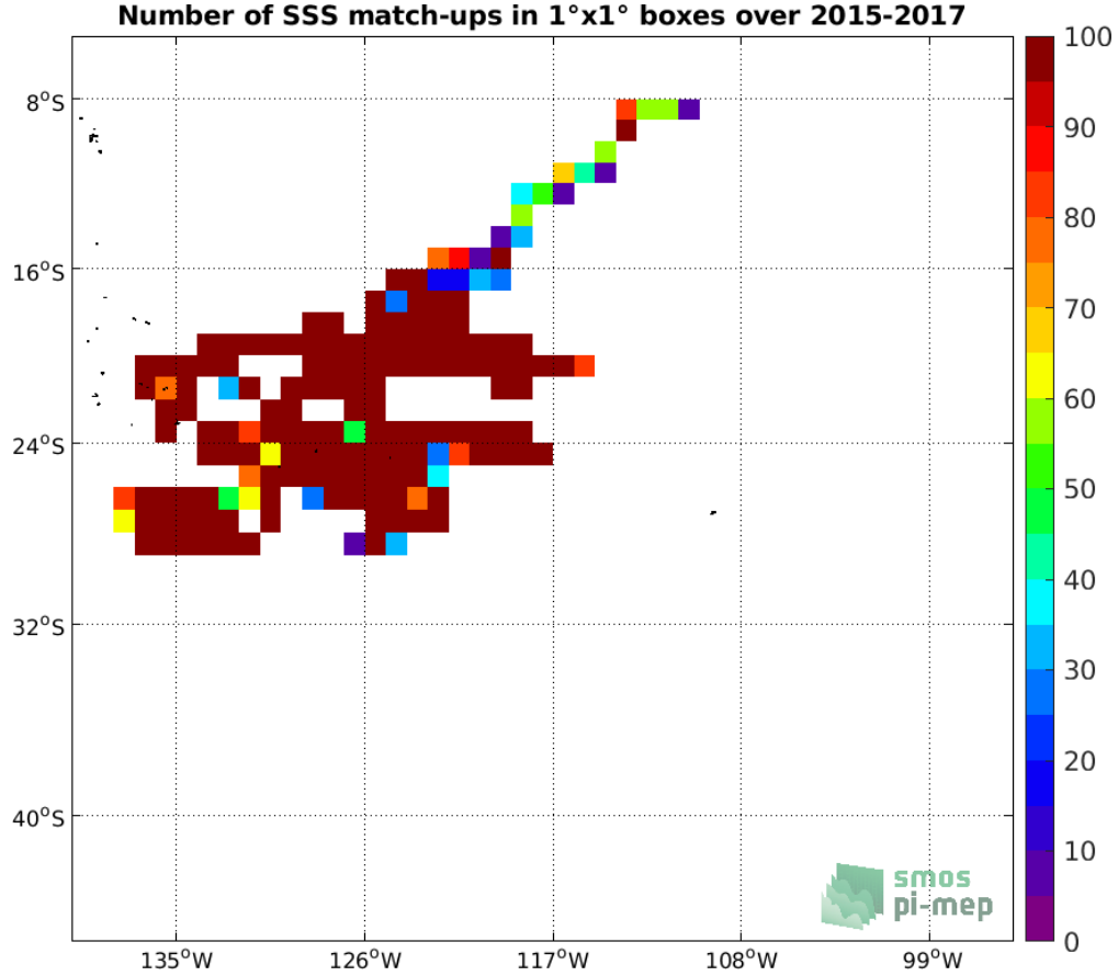
Figure 3: Number of SSS match-ups between Surface drifters SSS and the SMOS SSS L3 v317 - 10 Days - 25 km (CATDS-CPDC) SSS product for the OTT zone Pi-MEP region over 1^\circ \times 1^\circ boxes and for the full satellite product period.
