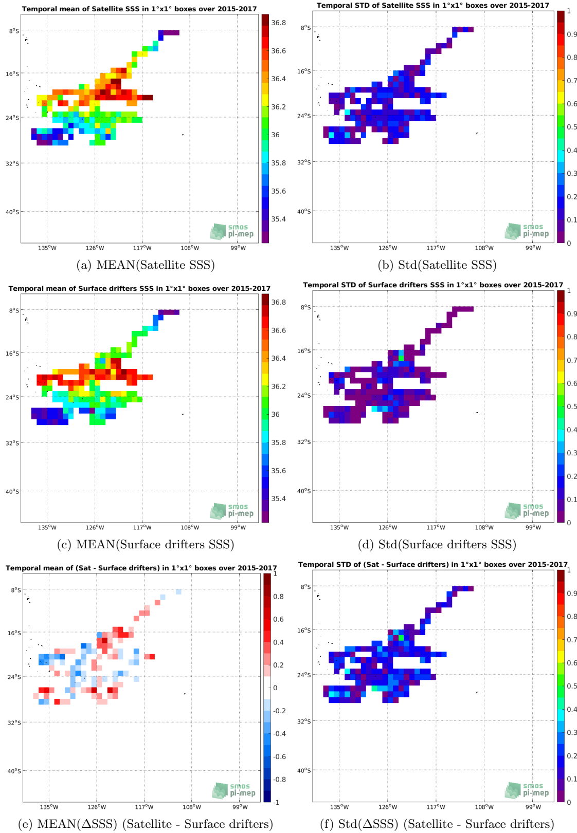
Figure 5: Temporal mean (left) and Std (right) of SSS from SMOS SSS L3 v317 - 10 Days - 25 km (CATDS-CPDC) (top), Surface drifters (middle), and of \Delta SSS (Satellite - Surface drifters). Only match-up pairs are used to generate these maps.
