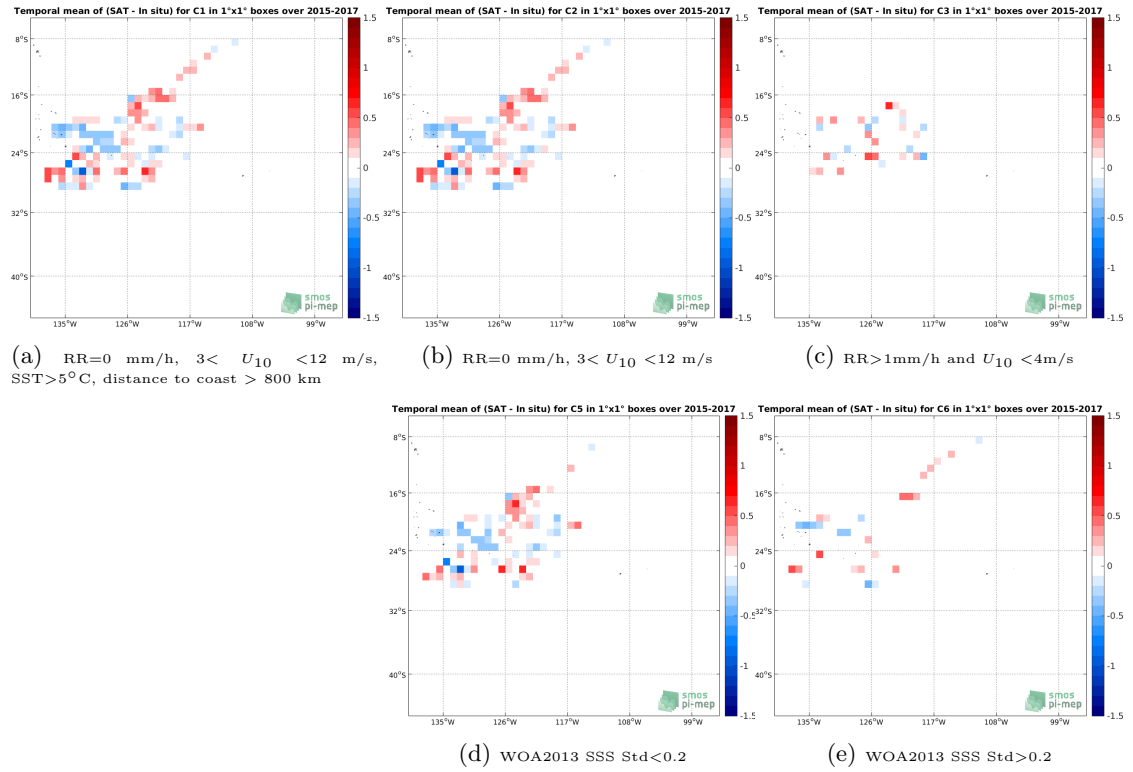
Figure 11: Temporal mean gridded over spatial boxes of size 1^\circ \times 1^\circ of \Delta SSS (SMOS-L3-CATDS-CPDC-V317-10DAYS-25KM - Surface drifters) for 5 different subdatasets corresponding to:RR=0 mm/h, 3 < U_{10} < 12 m/s, SST >5^\circ C, distance to coast > 800 km (a), RR=0 mm/h, 3 < U_{10} < 12 m/s (b), RR >1 mm/h and U_{10} < 4 m/s (c), WOA2013 SSS Std <0.2 (d), WOA2013 SSS Std >0.2 (e).
