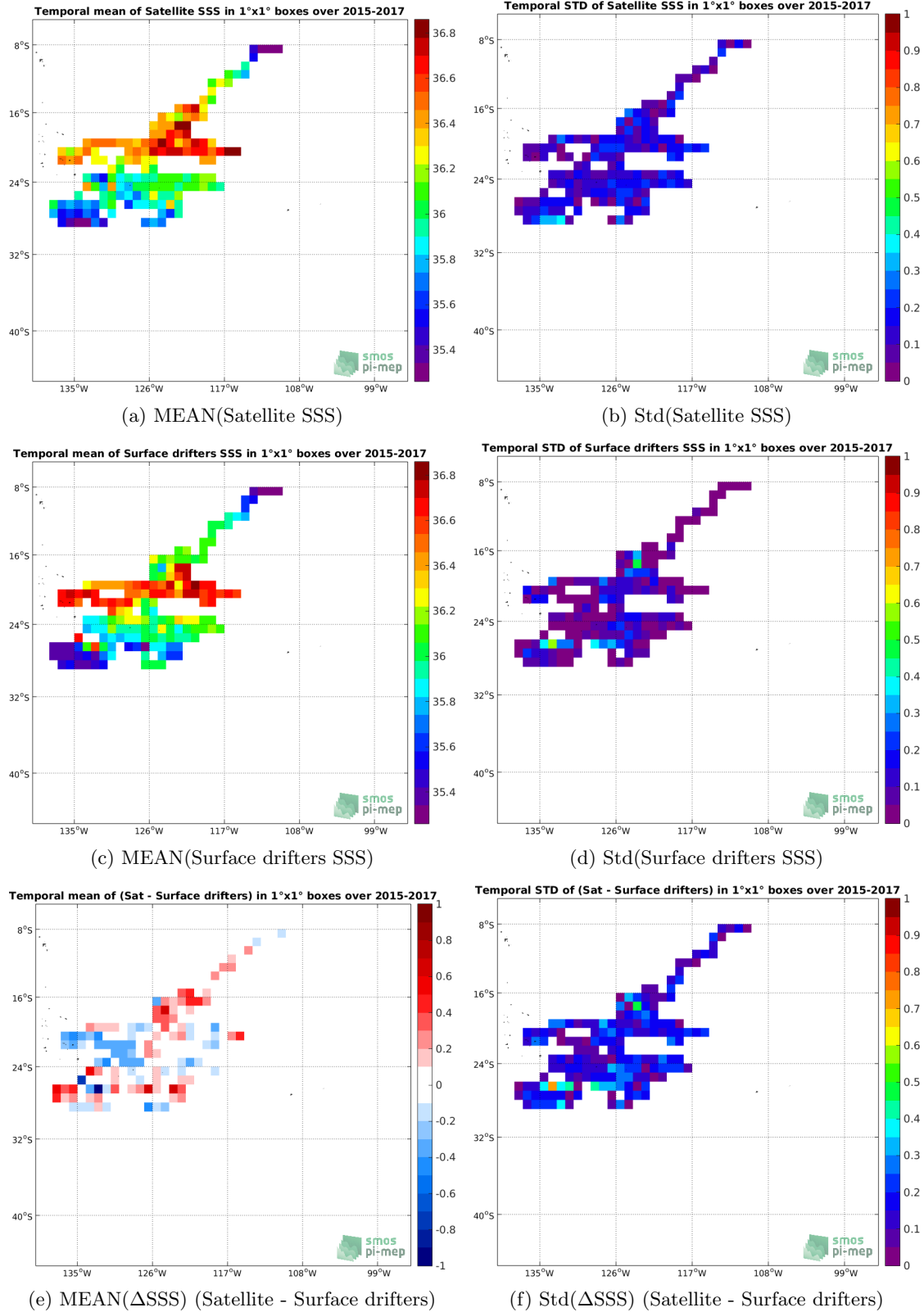
Figure 5: Temporal mean (left) and Std (right) of SSS from SMOS-L3-CATDS-CPDC-V317-10DAYS-25KM (top), Surface drifters (middle), and of \Delta SSS (Satellite - Surface drifters). Only match-up pairs are used to generate these maps.
