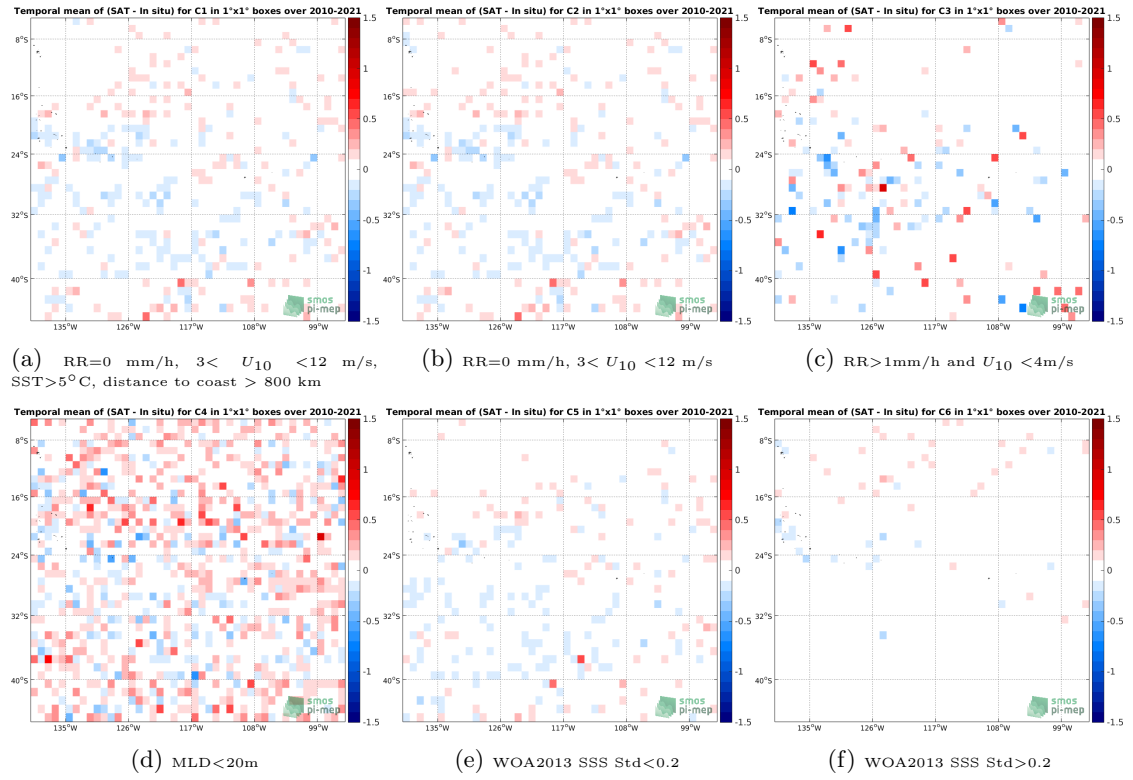
Figure 12: Temporal mean gridded over spatial boxes of size 1^\circ \times 1^\circ of \Delta SSS (SMOS SSS L3 v317 - 10 Days - 25 km (CATDS-CPDC) - Argo) for 6 different subdatasets corresponding to: RR=0 mm/h, 3 < U_{10} < 12 m/s, SST > 5^\circ C , distance to coast > 800 km (a), RR=0 mm/h, 3 < U_{10} < 12 m/s (b), RR > 1 mm/h and U_{10} < 4 m/s (c), MLD < 20 m (d), WOA2013 SSS Std < 0.2 (e), WOA2013 SSS Std > 0.2 (f).
