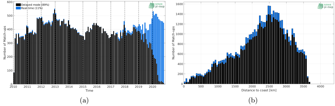
Figure 1: Number of match-ups between Argo and SMOS SSS L3 v317 - 10 Days - 25 km (CATDS-CPDC) SSS as a function of time (a) and as function of the distance to coast (b) over the OTT zone Pi-MEP region and for the full satellite product period.
