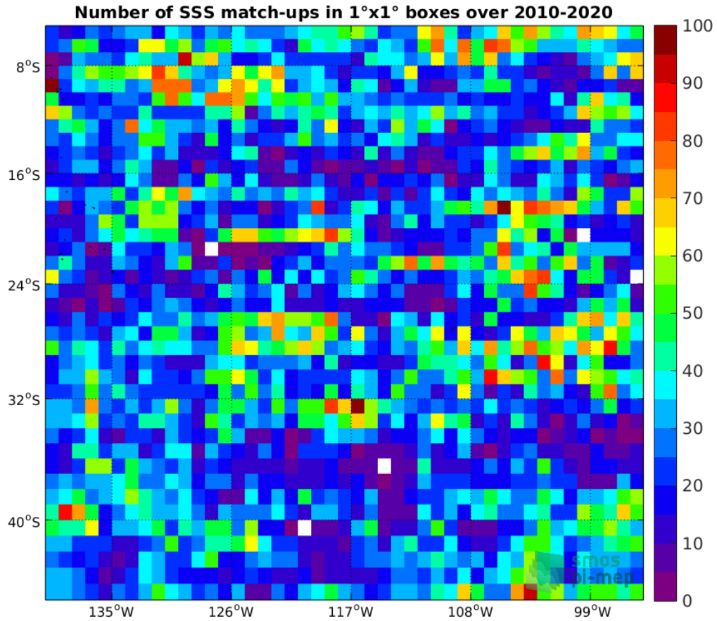
Figure 4: Number of SSS match-ups between Argo SSS and the SMOS SSS L3 v317 - 10 Days - 25 km (CATDS-CPDC) SSS product for the OTT zone Pi-MEP region over 1°x1° boxes and for the full satellite product period.
