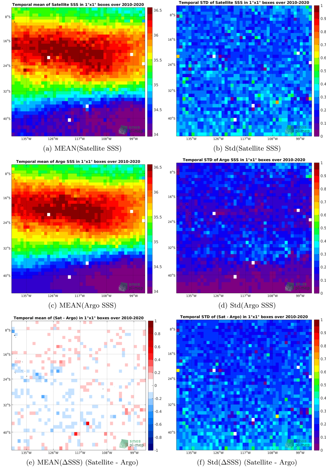
Figure 6: Temporal mean (left) and Std (right) of SSS from SMOS SSS L3 v317 - 10 Days - 25 km (CATDS-CPDC) (top), Argo (middle), and of \Delta SSS (Satellite - Argo). Only match-up pairs are used to generate these maps.
