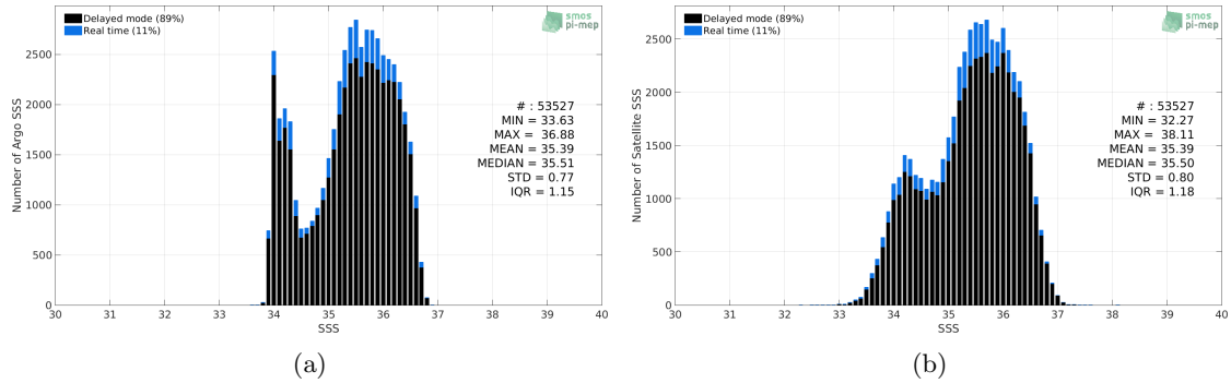
Figure 2: Histograms of SSS from Argo (a) and SMOS SSS L3 v317 - 10 Days - 25 km (CATDS-CPDC) (b) considering all match-up pairs per bins of 0.1 over the OTT zone Pi-MEP region and for the full satellite product period.
