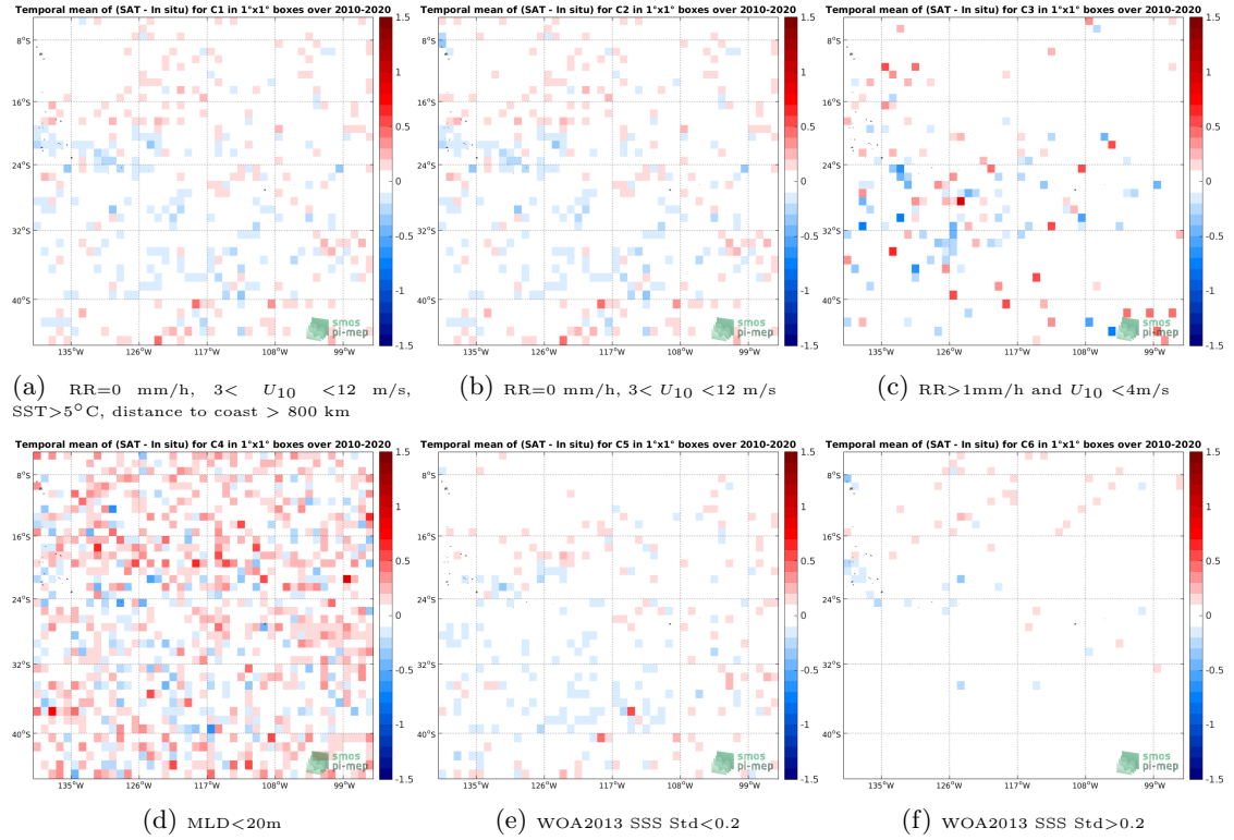
Figure 12: Temporal mean gridded over spatial boxes of size 1^\circ \times 1^\circ of \Delta SSS (SMOS SSS L3 v317 - 10 Days - 25 km (CATDS-CPDC) - Argo) for 6 different subdatasets corresponding to: RR=0 mm/h, 3 < U_{10} < 12 m/s, SST > 5^\circ C , distance to coast > 800 km (a), RR=0 mm/h, 3 < U_{10} < 12 m/s (b), RR > 1 mm/h and U_{10} < 4 m/s (c), MLD < 20 m (d), WOA2013 SSS Std < 0.2 (e), WOA2013 SSS Std > 0.2 (f).
