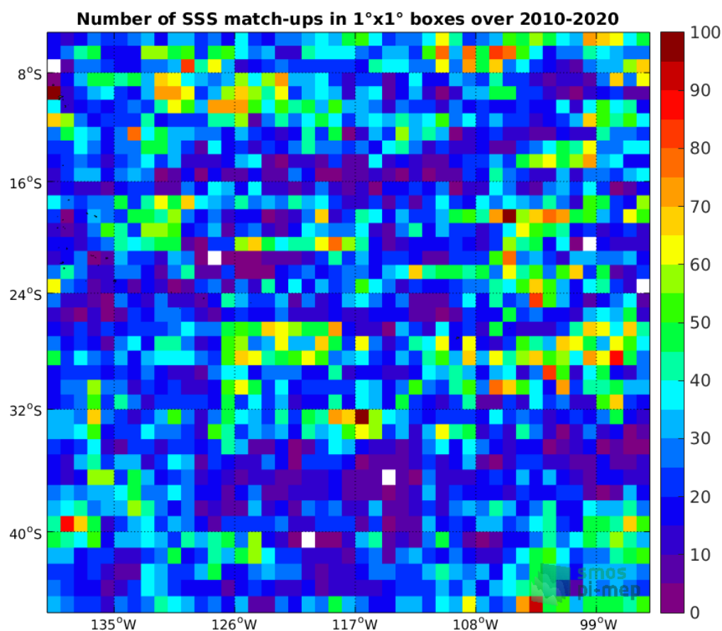
Figure 4: Number of SSS match-ups between Argo SSS and the SMOS L3 v317 - 10 Days - 25 km (CATDS-CPDC) SSS product for the OTT zone Pi-MEP region over 1°x1° boxes and for the full satellite product period.
