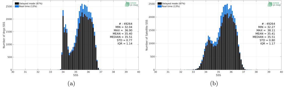
Figure 2: Histograms of SSS from Argo (a) and SMOS L3 v317 - 10 Days - 25 km (CATDS-CPDC) (b) considering all match-up pairs per bins of 0.1 over the OTT zone Pi-MEP region and for the full satellite product period.
