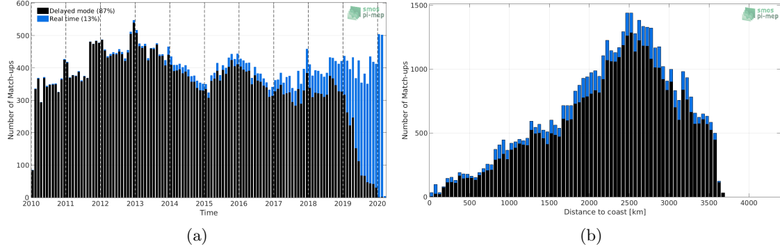
Figure 1: Number of match-ups between Argo and SMOS L3 v317 - 10 Days - 25 km (CATDS-CPDC) SSS as a function of time (a) and as function of the distance to coast (b) over the OTT zone Pi-MEP region and for the full satellite product period.
