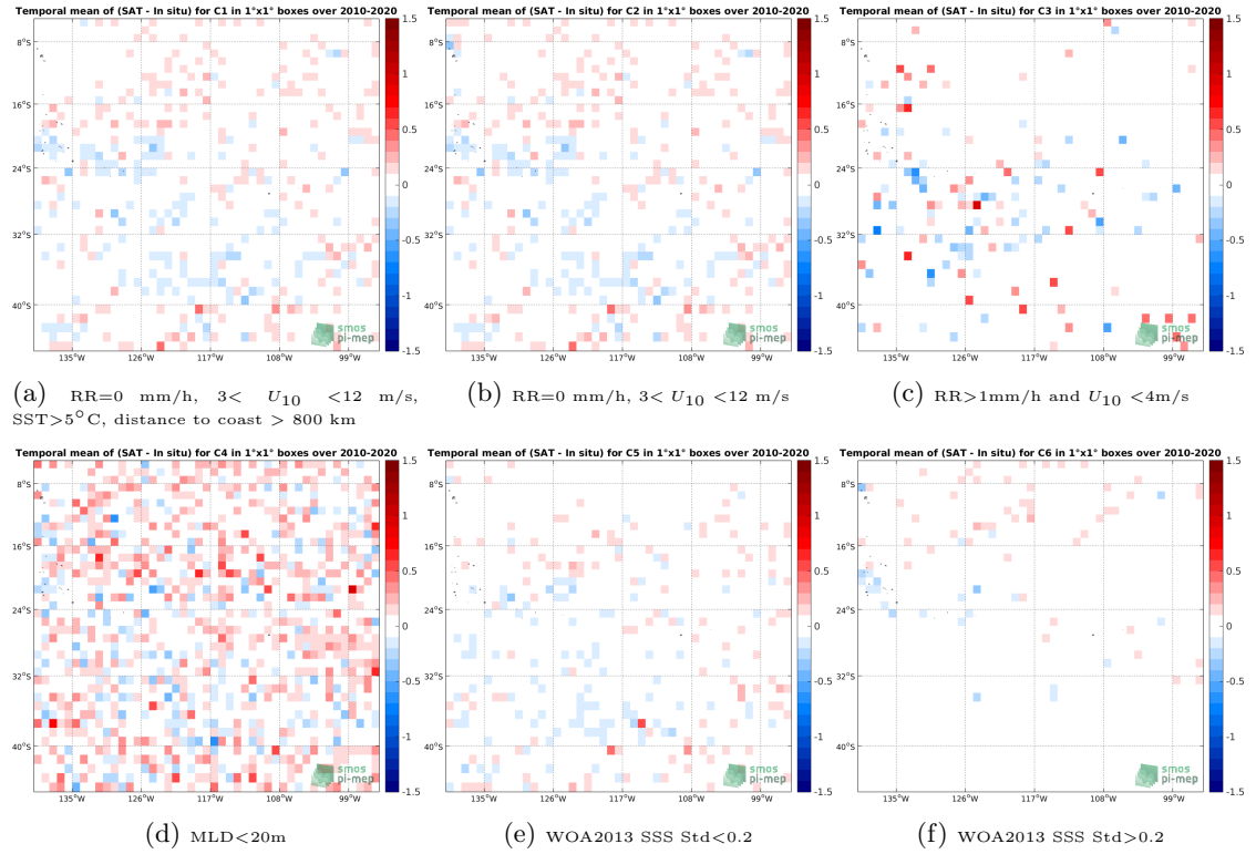
Figure 12: Temporal mean gridded over spatial boxes of size 1^\circ \times 1^\circ of \Delta SSS (SMOS L3 v317 - 10 Days - 25 km (CATDS-CPDC) - Argo) for 6 different subdatasets corresponding to: RR=0 mm/h, 3 < U_{10} < 12 m/s, SST >5^\circ C, distance to coast > 800 km (a), RR=0 mm/h, 3 < U_{10} < 12 m/s (b), RR >1 mm/h and U_{10} < 4 m/s (c),MLD <20 m (d),WOA2013 SSS Std <0.2 (e),WOA2013 SSS Std >0.2 (f).
