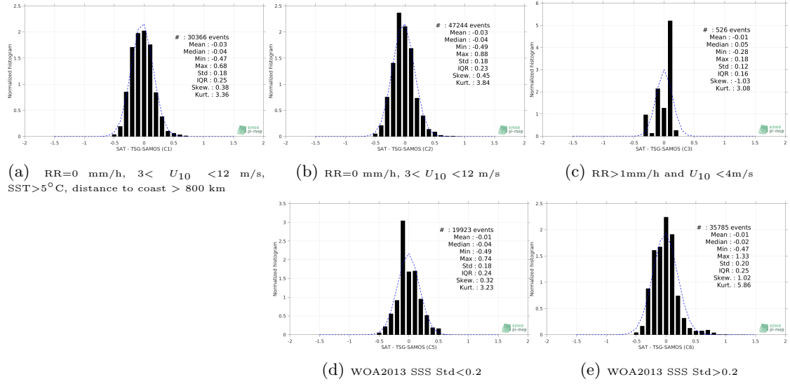
Figure 13: Normalized histogram of \Delta SSS (SMOS-L3-CATDS-CPDC-V3-MONTHLY-25KM - TSG-SAMOS) for 5 different subdatasets corresponding to: RR=0 mm/h, 3 < U_{10} < 12 m/s, SST>5°C, distance to coast > 800 km (a), RR=0 mm/h, 3 < U_{10} < 12 m/s (b), RR>1mm/h and U_{10} < 4 m/s (c), WOA2013 SSS Std<0.2 (d), WOA2013 SSS Std>0.2 (e).
