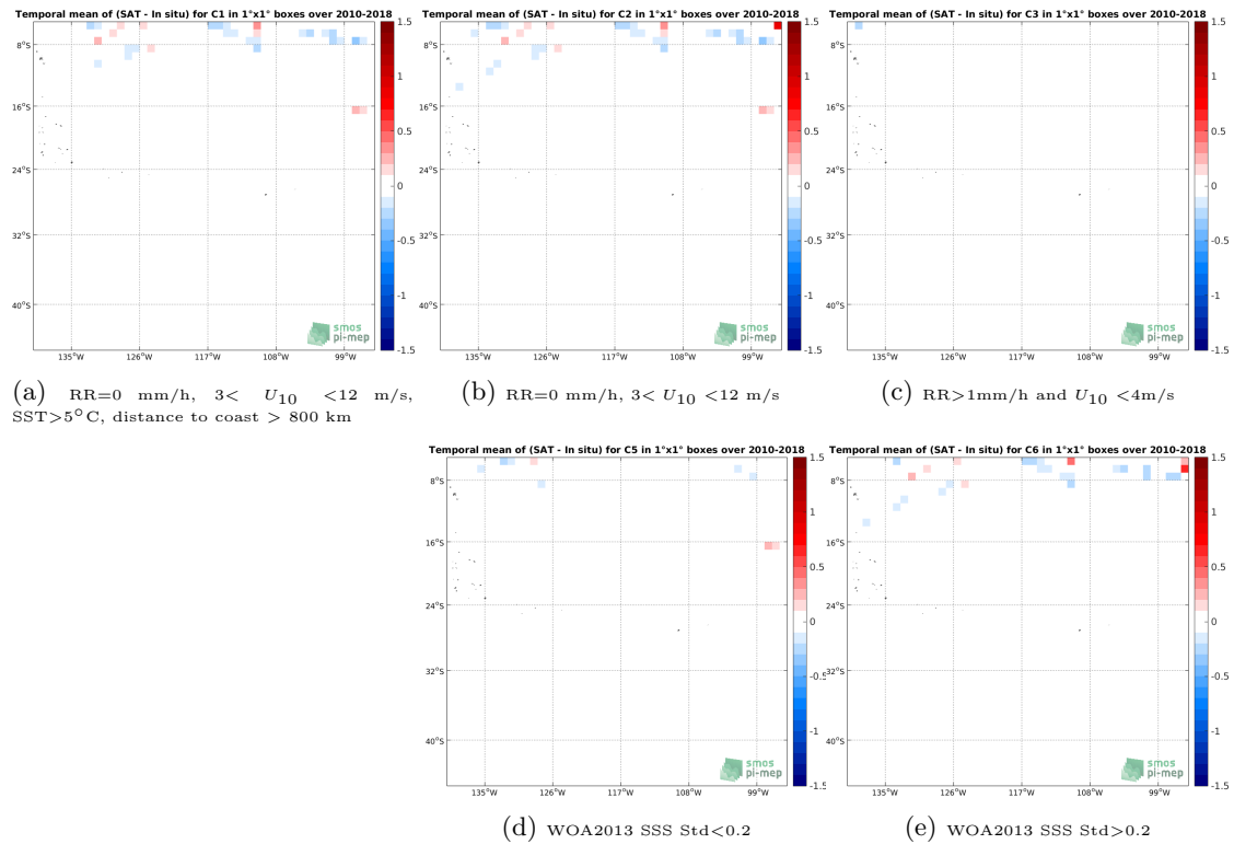
Figure 12: Temporal mean gridded over spatial boxes of size 1^\circ \times 1^\circ of \Delta SSS (SMOS-L3-CATDS-CPDC-V3-MONTHLY-25KM - TSG-SAMOS) for 5 different subdatasets corresponding to:RR=0 mm/h, 3 < U_{10} < 12 m/s, SST >5^\circ C, distance to coast > 800 km (a), RR=0 mm/h, 3 < U_{10} < 12 m/s (b), RR >1 mm/h and U_{10} < 4 m/s (c), WOA2013 SSS Std <0.2 (d), WOA2013 SSS Std >0.2 (e).
