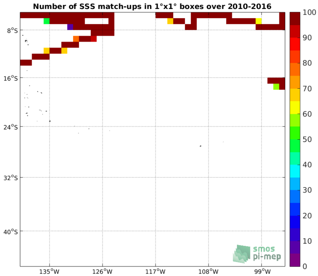
Figure 4: Number of SSS match-ups between TSG-SAMOS SSS and the SMOS-L3-CATDS-CPDC-V3-MONTHLY-25KM SSS product for the OTT zone Pi-MEP region over 1°x1° boxes and for the full satellite product period.
