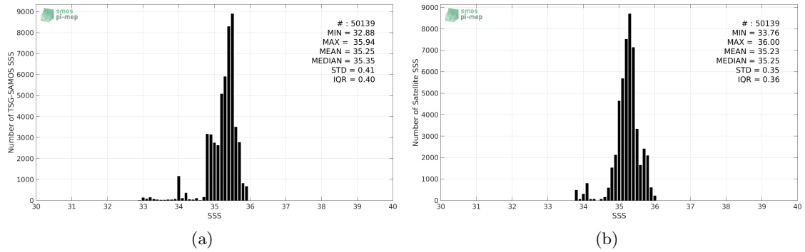
Figure 2: Histograms of SSS from TSG-SAMOS (a) and SMOS-L3-CATDS-CPDC-V3-MONTHLY-25KM (b) considering all match-up pairs per bins of 0.1 over the OTT zone Pi-MEP region and for the full satellite product period.
