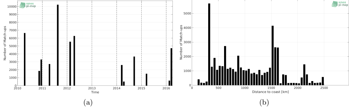
Figure 1: Number of match-ups between TSG-SAMOS and SMOS-L3-CATDS-CPDC-V3-MONTHLY-25KM SSS as a function of time (a) and as function of the distance to coast (b) over the OTT zone Pi-MEP region and for the full satellite product period.
