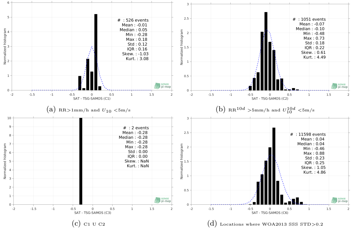
Figure 13: Normalized histogram of \Delta\text{SSS} (SMOS-L3-CATDS-CPDC-V3-MONTHLY-25KM - TSG-SAMOS) for 6 different subdatasets corresponding to: RR > 1mm/h and U_{10} < 5\text{m/s} (a), RR^{10d} > 5\text{mm/h} and U_{10}^{10d} < 5\text{m/s} (b), C1 U C2 (c), Locations where WOA2013 SSS STD > 0.2 (d).
