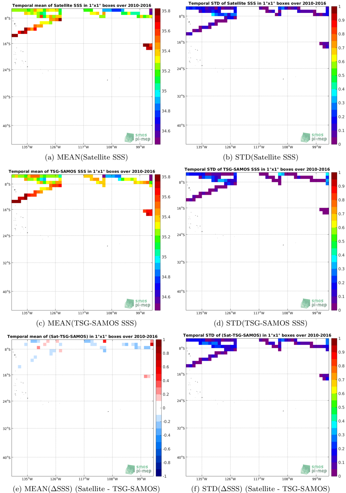
Figure 6: Temporal mean (left) and STD (right) of SSS from SMOS-L3-CATDS-CPDC-V3-MONTHLY-25KM (top), TSG-SAMOS (middle), and of \Delta SSS (Satellite - TSG-SAMOS). Only match-up pairs are used to generate these maps.
