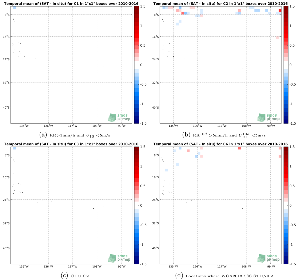
Figure 12: Temporal mean gridded over spatial boxes of size 1^\circ \times 1^\circ of \Delta SSS (SMOS-L3-CATDS-CPDC-V3-MONTHLY-25KM - TSG-SAMOS) for 4 different subdatasets corresponding to: RR > 1mm/h and U_{10} < 5\text{m/s} (a), RR^{10d} > 5\text{mm/h} and U_{10}^{10d} < 5\text{m/s} (b), C1 U C2 (c), Locations where WOA2013 SSS STD > 0.2 (d).
