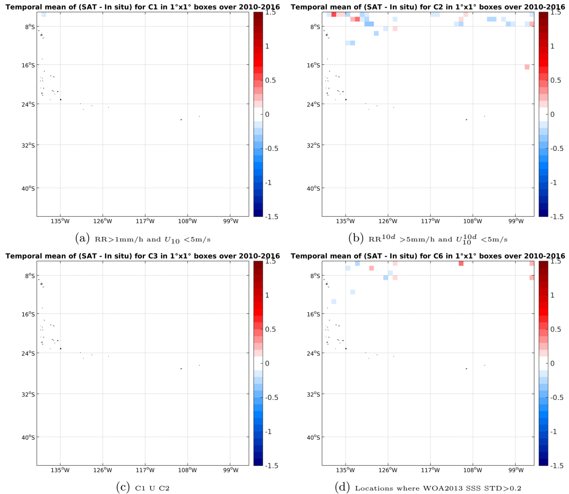
Figure 12: Temporal mean gridded over spatial boxes of size 1^\circ \times 1^\circ of \Delta SSS (SMOS-L3-CATDS-CPDC-V3-MONTHLY-25KM - TSG-SAMOS) for 4 different subdatasets corresponding to: RR > 1 mm/h and U_{10} < 5 m/s (a), RR 10d > 5 mm/h and U_{10}^{10d} < 5 m/s (b), C1 U C2 (c), Locations where WOA2013 SSS STD > 0.2 (d).
