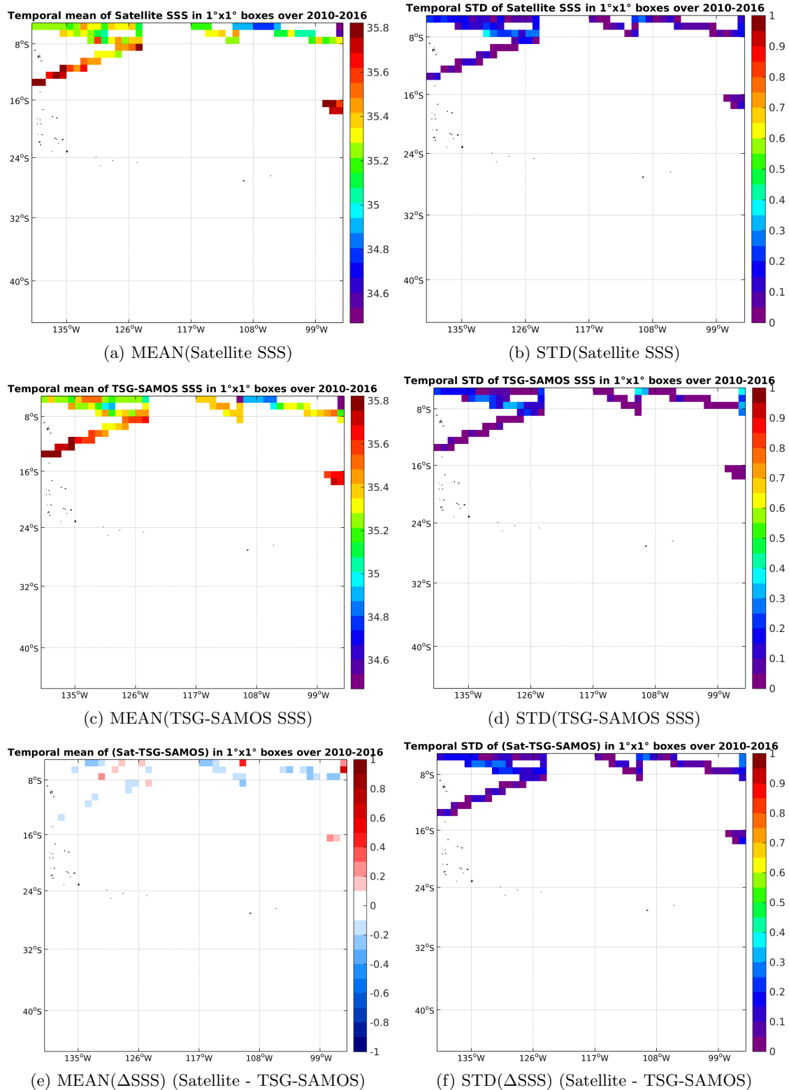
Figure 6: Temporal mean (left) and STD (right) of SSS from SMOS-L3-CATDS-CPDC-V3-MONTHLY-25KM (top), TSG-SAMOS (middle), and of \Delta SSS (Satellite - TSG-SAMOS). Only match-up pairs are used to generate these maps.
