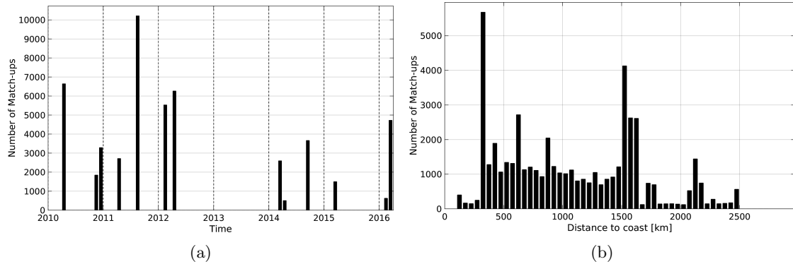
Figure 1: Number of match-ups between TSG-SAMOS and SMOS-L3-CATDS-CPDC-V3-MONTHLY-25KM SSS as a function of time (a) and as function of the distance to coast (b) over the OTT zone Pi-MEP region and for the full satellite product period.
