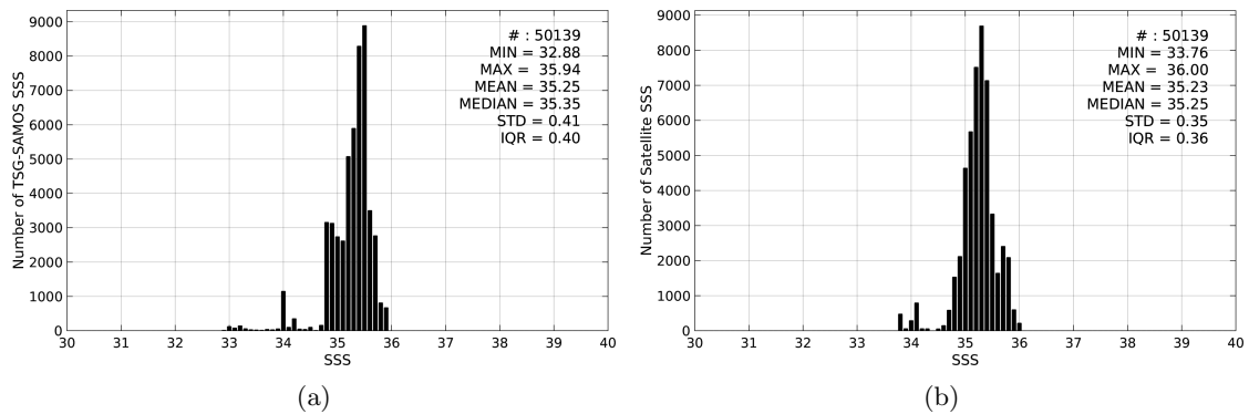
Figure 2: Histograms of SSS from TSG-SAMOS (a) and SMOS-L3-CATDS-CPDC-V3-MONTHLY-25KM (b) considering all match-up pairs per bins of 0.1 over the OTT zone Pi-MEP region and for the full satellite product period.
