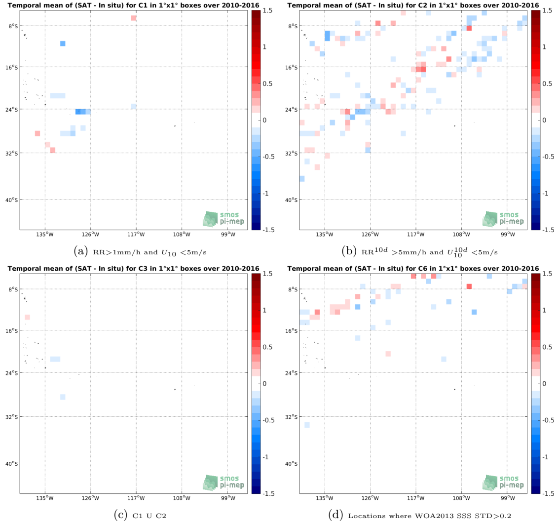
Figure 12: Temporal mean gridded over spatial boxes of size 1^\circ \times 1^\circ of \Delta SSS (SMOS-L3-CATDS-CPDC-V3-MONTHLY-25KM - TSG-LEGOS-DM) for 4 different subdatasets corresponding to: RR > 1\text{mm/h} and U_{10} < 5\text{m/s} (a), RR^{10d} > 5\text{mm/h} and U_{10}^{10d} < 5\text{m/s} (b), C1 U C2 (c), Locations where WOA2013 SSS STD > 0.2 (d).
