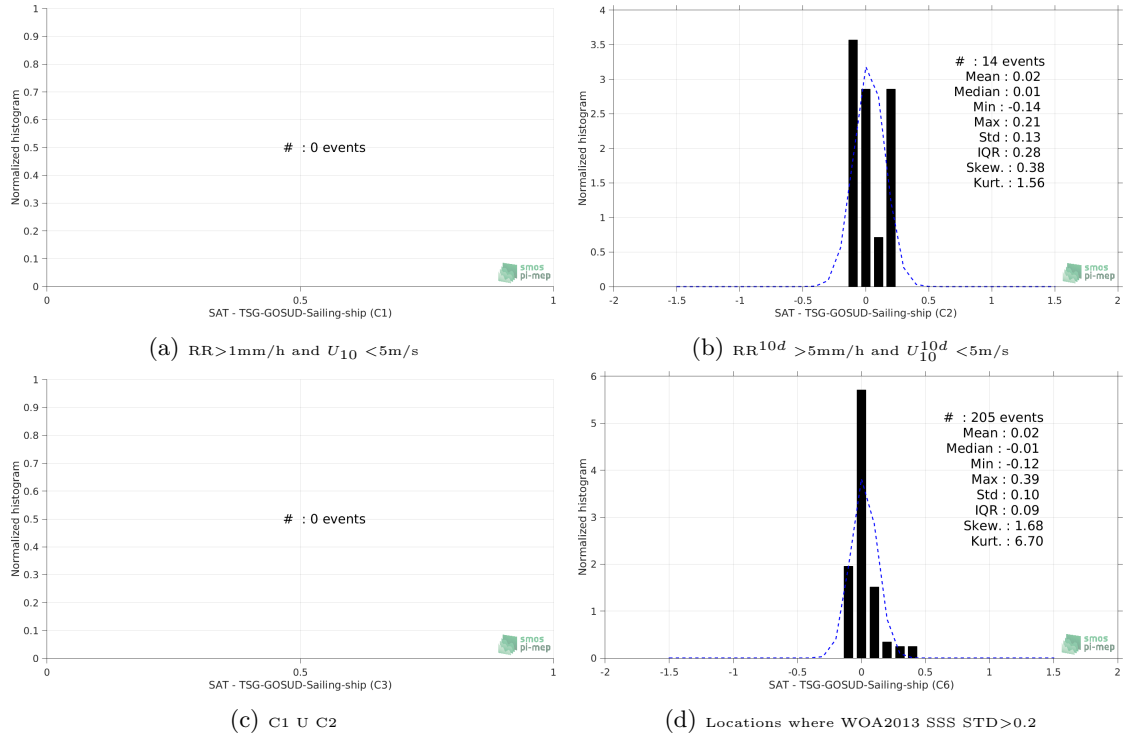
Figure 13: Normalized histogram of \Delta\text{SSS} (SMOS-L3-CATDS-CPDC-V3-MONTHLY-25KM - TSG-GOSUD-Sailing-ship) for 6 different subdatasets corresponding to: RR > 1\text{mm/h} and U_{10} < 5\text{m/s} (a), RR^{10d} > 5\text{mm/h} and U_{10}^{10d} < 5\text{m/s} (b), C1 U C2 (c), Locations where WOA2013 SSS STD > 0.2 (d).
