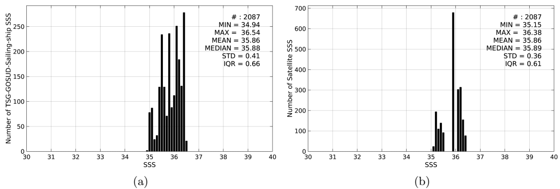
Figure 2: Histograms of SSS from TSG-GOSUD-Sailing-ship (a) and SMOS-L3-CATDS-CPDC-V3-MONTHLY-25KM (b) considering all match-up pairs per bins of 0.1 over the OTT zone Pi-MEP region and for the full satellite product period.
