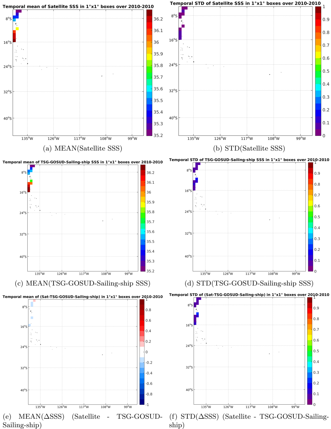
Figure 6: Temporal mean (left) and STD (right) of SSS from SMOS-L3-CATDS-CPDC-V3-MONTHLY-25KM (top), TSG-GOSUD-Sailing-ship (middle), and of \Delta SSS (Satellite - TSG-GOSUD-Sailing-ship). Only match-up pairs are used to generate these maps.
