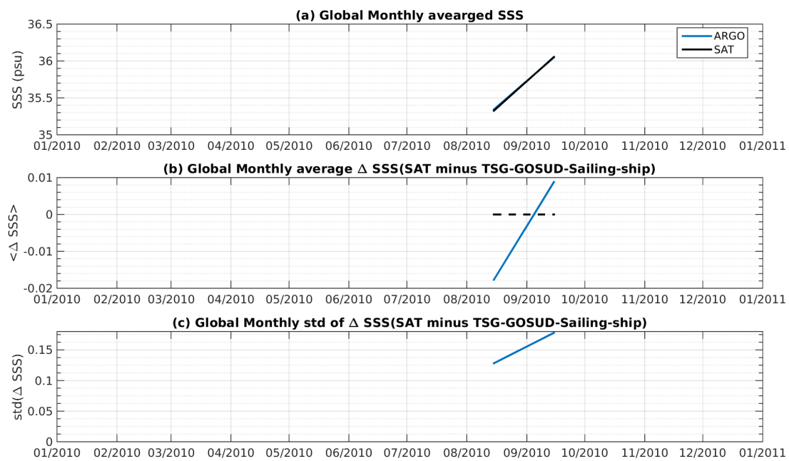
Figure 7: Time series of the monthly averaged mean SSS (top), mean \Delta SSS (Satellite - TSG-GOSUD-Sailing-ship) and STD of \Delta SSS (Satellite - TSG-GOSUD-Sailing-ship) over the OTT zone Pi-MEP region considering all match-ups collected by the Pi-MEP platform.
