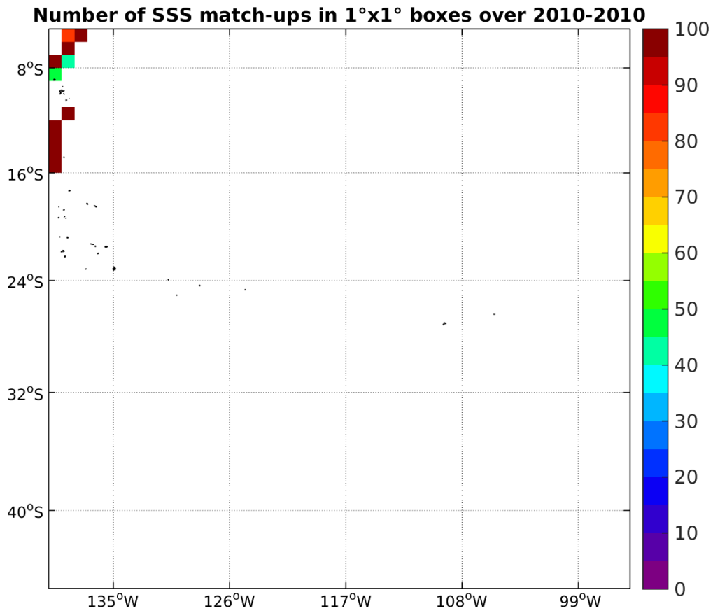
Figure 4: Number of SSS match-ups between TSG-GOSUD-Sailing-ship SSS and the SMOS-L3-CATDS-CPDC-V3-MONTHLY-25KM SSS product for the OTT zone Pi-MEP region over 1°x1° boxes and for the full satellite product period.
