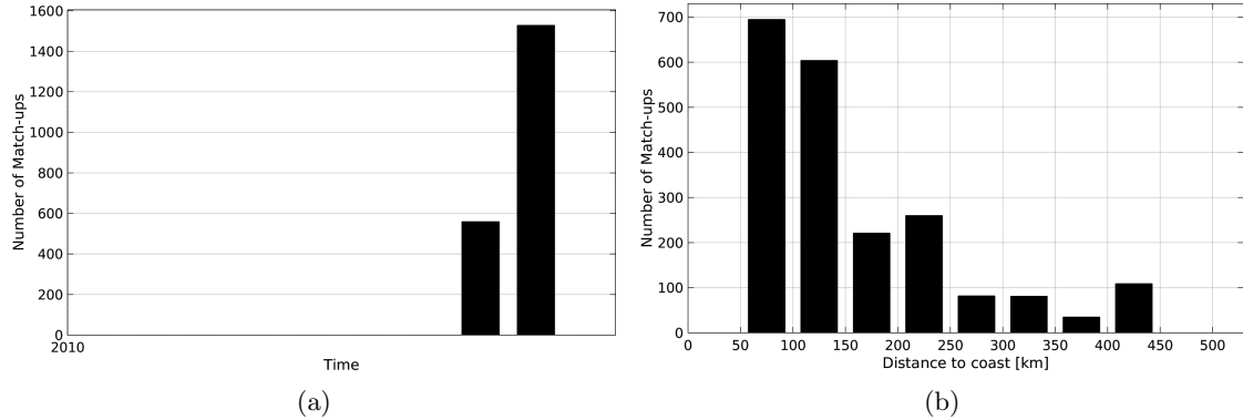
Figure 1: Number of match-ups between TSG-GOSUD-Sailing-ship and SMOS-L3-CATDS-CPDC-V3-MONTHLY-25KM SSS as a function of time (a) and as function of the distance to coast (b) over the OTT zone Pi-MEP region and for the full satellite product period.
