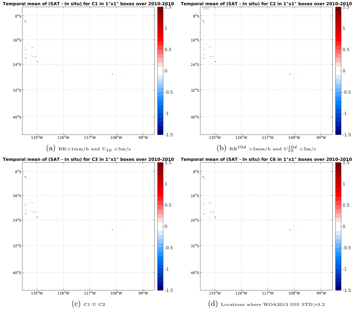
Figure 12: Temporal mean gridded over spatial boxes of size 1^\circ \times 1^\circ of \Delta SSS (SMOS-L3-CATDS-CPDC-V3-MONTHLY-25KM - TSG-GOSUD-Sailing-ship) for 4 different subdatasets corresponding to: RR > 1mm/h and U_{10} < 5 m/s (a), RR^{10d} > 5 mm/h and U_{10}^{10d} < 5 m/s (b), C1 U C2 (c), Locations where WOA2013 SSS STD > 0.2 (d).
