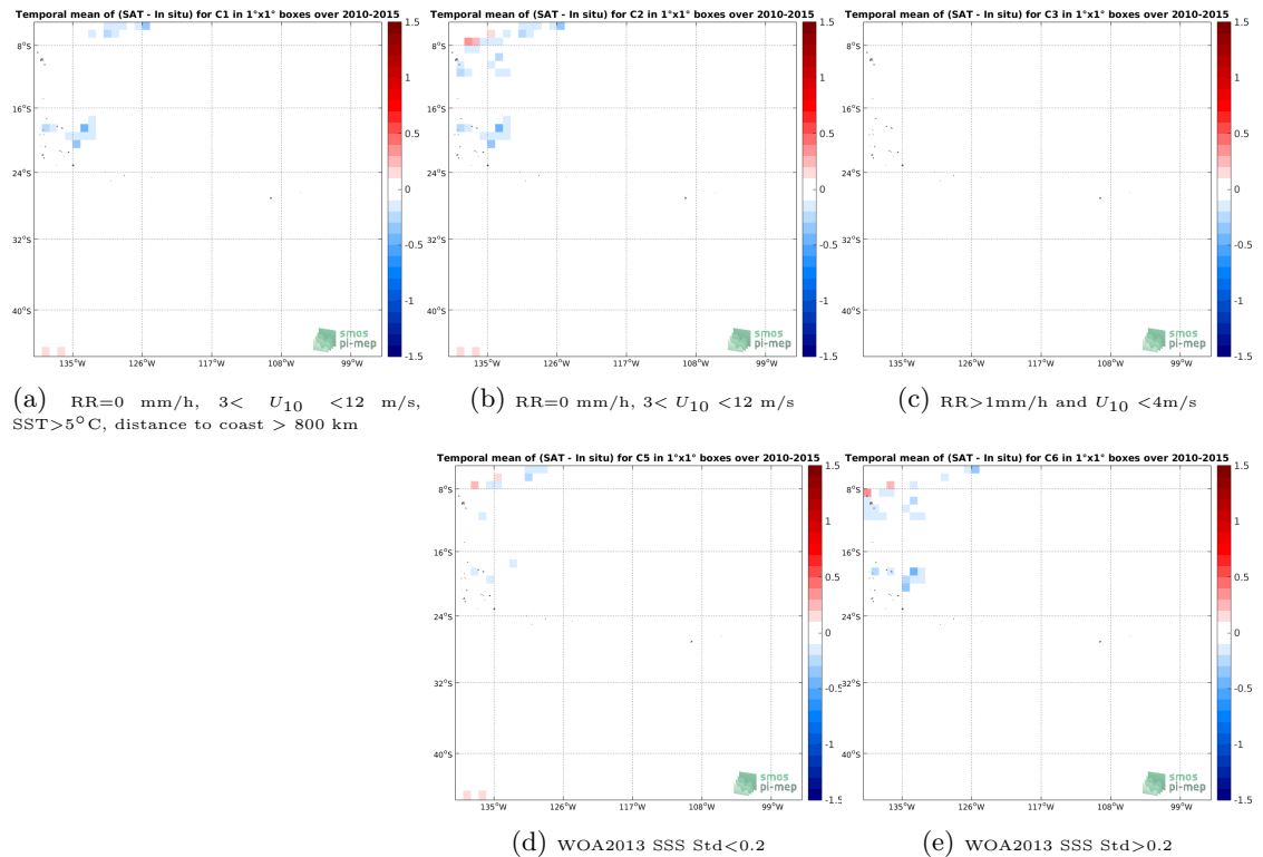
Figure 12: Temporal mean gridded over spatial boxes of size 1^\circ \times 1^\circ of \Delta SSS (SMOS-L3-CATDS-CPDC-V3-MONTHLY-25KM - TSG-GOSUD-Research-vessel) for 5 different subdatasets corresponding to:RR=0 mm/h, 3 < U_{10} < 12 m/s, SST >5^\circ C, distance to coast > 800 km (a), RR=0 mm/h, 3 < U_{10} < 12 m/s (b), RR >1 mm/h and U_{10} < 4 m/s (c), WOA2013 SSS Std <0.2 (d), WOA2013 SSS Std >0.2 (e).
