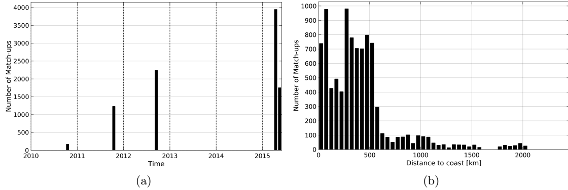
Figure 1: Number of match-ups between TSG-GOSUD-Research-vessel and SMOS-L3-CATDS-CPDC-V3-MONTHLY-25KM SSS as a function of time (a) and as function of the distance to coast (b) over the OTT zone Pi-MEP region and for the full satellite product period.
