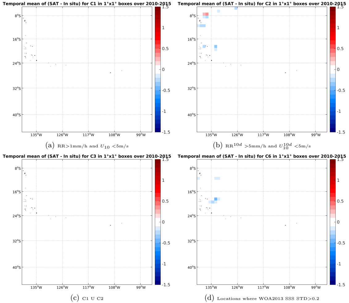
Figure 12: Temporal mean gridded over spatial boxes of size 1°x1° of \Delta SSS (SMOS-L3-CATDS-CPDC-V3-MONTHLY-25KM - TSG-GOSUD-Research-vessel) for 4 different subdatasets corresponding to: RR > 1\text{mm/h} and U_{10} < 5\text{m/s} (a), RR^{10d} > 5\text{mm/h} and U_{10}^{10d} < 5\text{m/s} (b), C1 U C2 (c), Locations where WOA2013 SSS STD > 0.2 (d).
