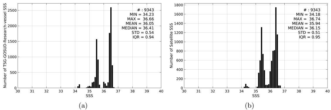
Figure 2: Histograms of SSS from TSG-GOSUD-Research-vessel (a) and SMOS-L3-CATDS-CPDC-V3-MONTHLY-25KM (b) considering all match-up pairs per bins of 0.1 over the OTT zone Pi-MEP region and for the full satellite product period.
