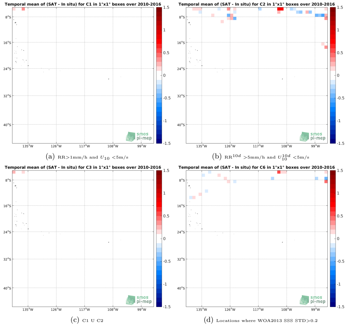
Figure 12: Temporal mean gridded over spatial boxes of size 1^\circ \times 1^\circ of \Delta SSS (SMOS-L3-CATDS-CPDC-V3-10DAYS-25KM - TSG-SAMOS) for 4 different subdatasets corresponding to: RR > 1mm/h and U_{10} < 5\text{m/s} (a), RR^{10d} > 5\text{mm/h} and U_{10}^{10d} < 5\text{m/s} (b), C1 U C2 (c), Locations where WOA2013 SSS STD > 0.2 (d).
