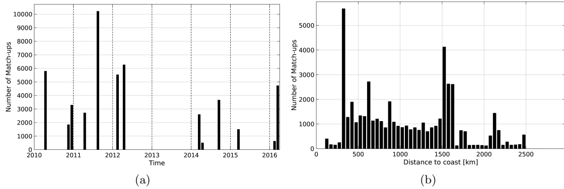
Figure 1: Number of match-ups between TSG-SAMOS and SMOS-L3-CATDS-CPDC-V3-10DAYS-25KM SSS as a function of time (a) and as function of the distance to coast (b) over the OTT zone Pi-MEP region and for the full satellite product period.
