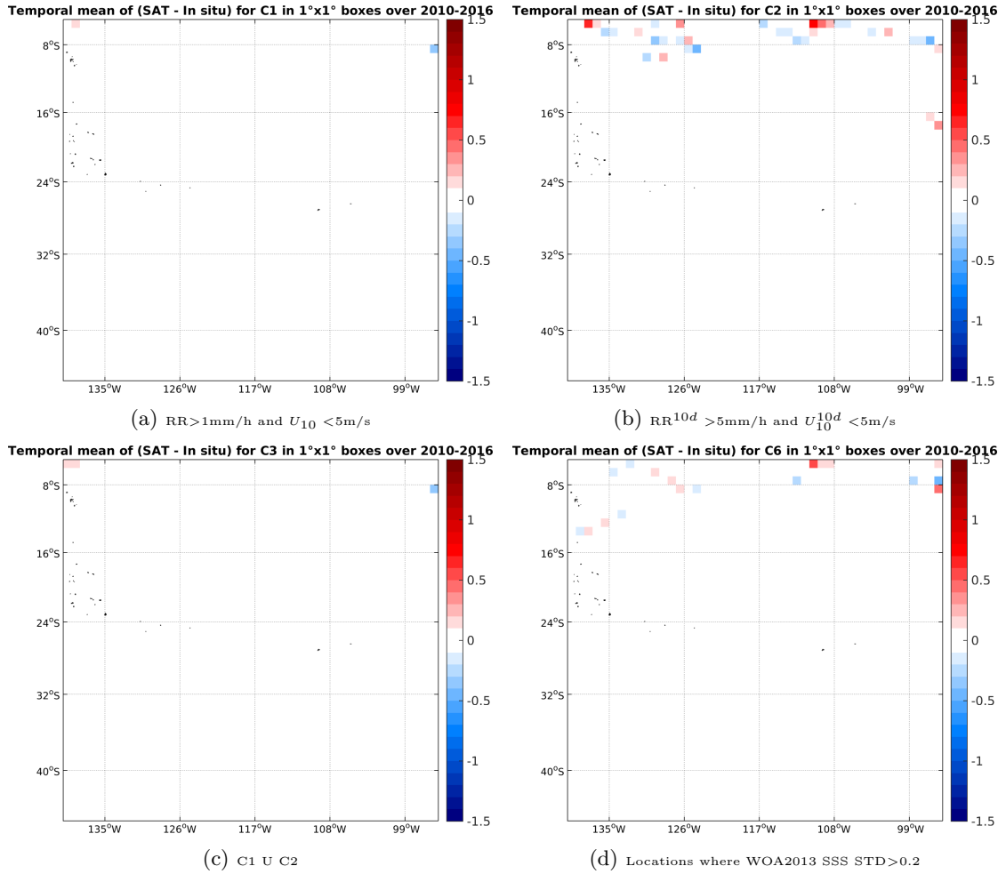
Figure 12: Temporal mean gridded over spatial boxes of size 1^\circ \times 1^\circ of \Delta SSS (SMOS-L3-CATDS-CPDC-V3-10DAYS-25KM - TSG-SAMOS) for 4 different subdatasets corresponding to: RR > 1mm/h and U_{10} < 5\text{m/s} (a), RR^{10d} > 5\text{mm/h} and U_{10}^{10d} < 5\text{m/s} (b), C1 U C2 (c), Locations where WOA2013 SSS STD > 0.2 (d).
