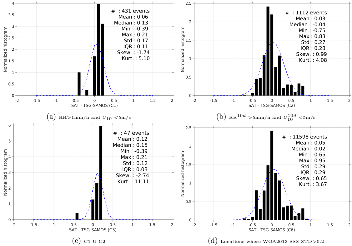
Figure 13: Normalized histogram of \Delta\text{SSS} (SMOS-L3-CATDS-CPDC-V3-10DAYS-25KM - TSG-SAMOS) for 6 different subdatasets corresponding to: RR>1mm/h and U_{10} < 5\text{m/s} (a), \text{RR}^{10d} > 5\text{mm/h} and U_{10}^{10d} < 5\text{m/s} (b), C1 U C2 (c), Locations where WOA2013 SSS STD>0.2 (d).
