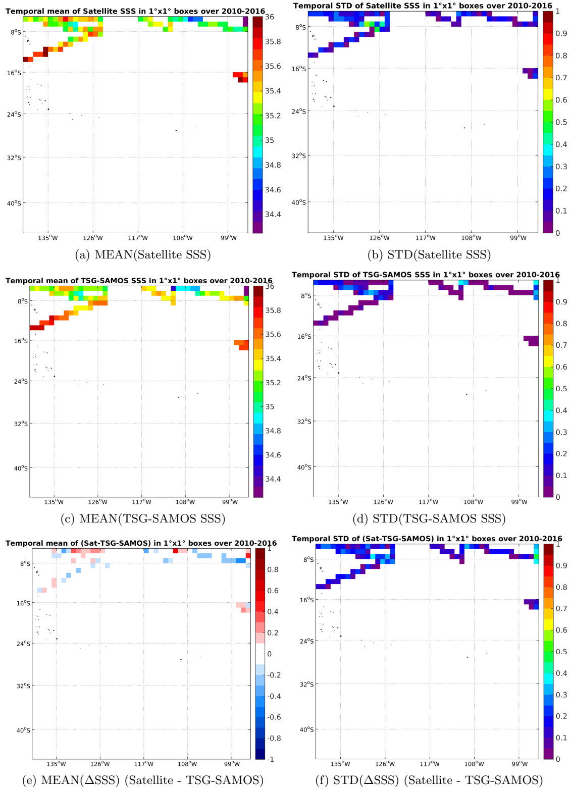
Figure 6: Temporal mean (left) and STD (right) of SSS from SMOS-L3-CATDS-CPDC-V3-10DAYS-25KM (top), TSG-SAMOS (middle), and of \Delta SSS (Satellite - TSG-SAMOS). Only match-up pairs are used to generate these maps.
