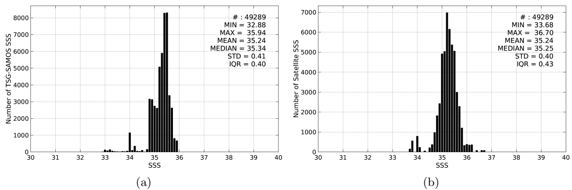
Figure 2: Histograms of SSS from TSG-SAMOS (a) and SMOS-L3-CATDS-CPDC-V3-10DAYS-25KM (b) considering all match-up pairs per bins of 0.1 over the OTT zone Pi-MEP region and for the full satellite product period.
