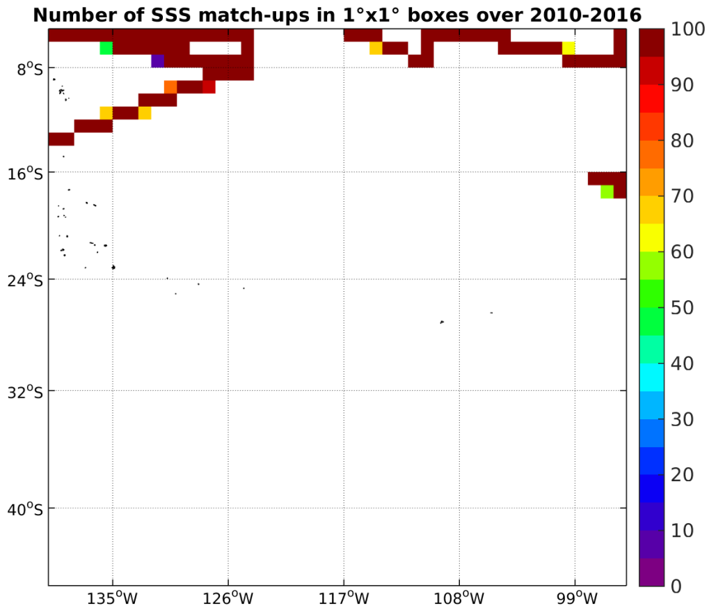
Figure 4: Number of SSS match-ups between TSG-SAMOS SSS and the SMOS-L3-CATDS-CPDC-V3-10DAYS-25KM SSS product for the OTT zone Pi-MEP region over 1°x1° boxes and for the full satellite product period.
