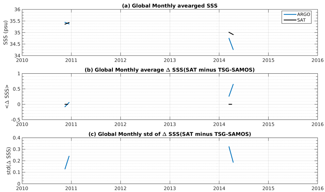
Figure 7: Time series of the monthly averaged mean SSS (top), mean \Delta SSS (Satellite - TSG-SAMOS) and STD of \Delta SSS (Satellite - TSG-SAMOS) over the OTT zone Pi-MEP region considering all match-ups collected by the Pi-MEP platform.
