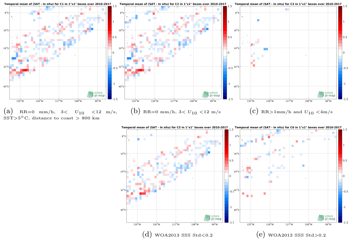
Figure 12: Temporal mean gridded over spatial boxes of size 1^\circ \times 1^\circ of \Delta SSS (SMOS-L3-CATDS-CPDC-V3-10DAYS-25KM - TSG-LEGOS-DM) for 5 different subdatasets corresponding to:RR=0 mm/h, 3 < U_{10} < 12 m/s, SST >5^\circ C, distance to coast > 800 km (a), RR=0 mm/h, 3 < U_{10} < 12 m/s (b), RR >1 mm/h and U_{10} < 4 m/s (c), WOA2013 SSS Std <0.2 (d), WOA2013 SSS Std >0.2 (e).
