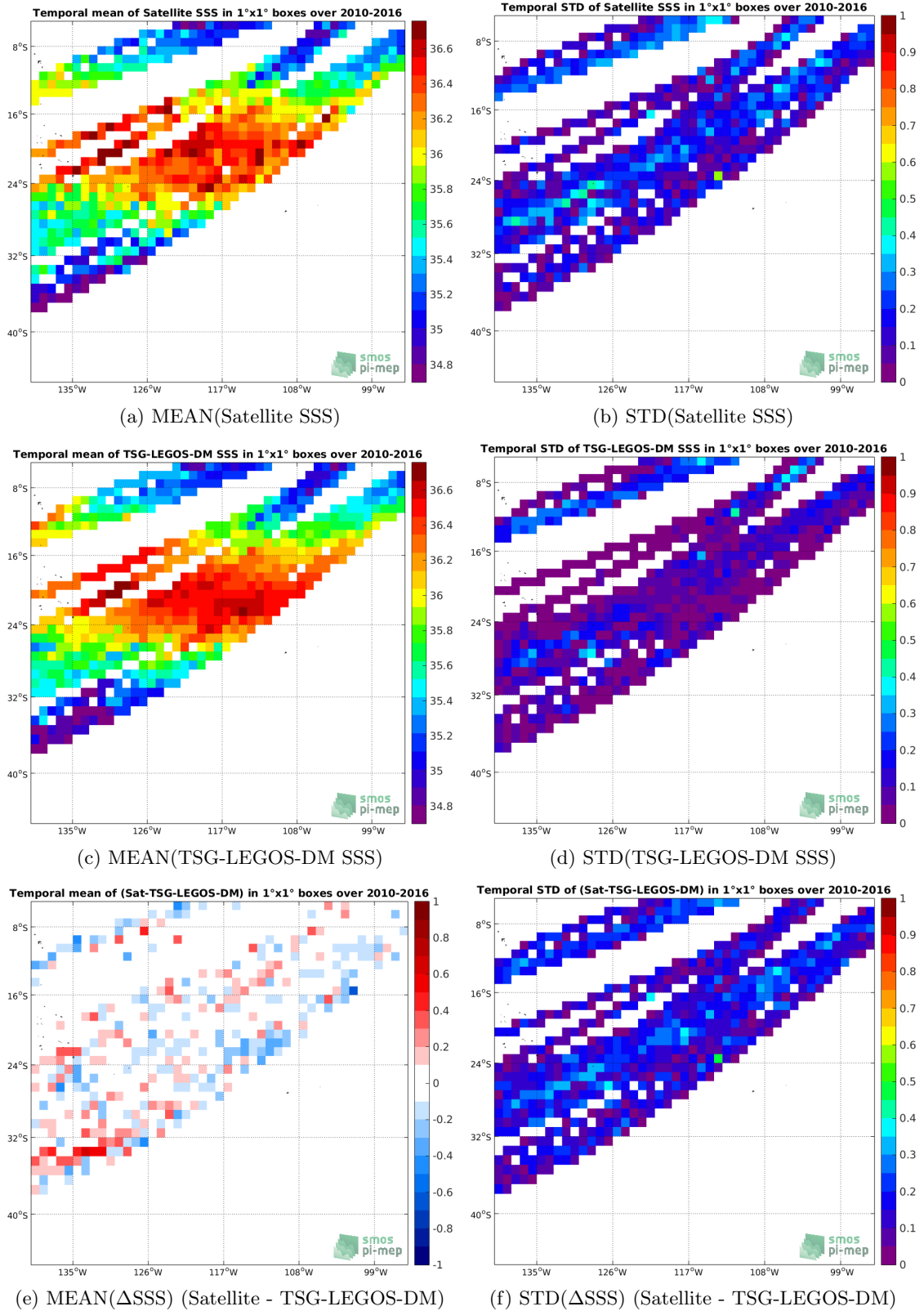
Figure 6: Temporal mean (left) and STD (right) of SSS from SMOS-L3-CATDS-CPDC-V3-10DAYS-25KM (top), TSG-LEGOS-DM (middle), and of \Delta SSS (Satellite - TSG-LEGOS-DM). Only match-up pairs are used to generate these maps.
