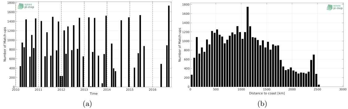
Figure 1: Number of match-ups between TSG-LEGOS-DM and SMOS-L3-CATDS-CPDC-V3-10DAYS-25KM SSS as a function of time (a) and as function of the distance to coast (b) over the OTT zone Pi-MEP region and for the full satellite product period.
