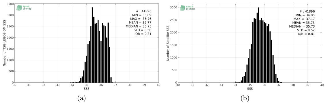
Figure 2: Histograms of SSS from TSG-LEGOS-DM (a) and SMOS-L3-CATDS-CPDC-V3-10DAYS-25KM (b) considering all match-up pairs per bins of 0.1 over the OTT zone Pi-MEP region and for the full satellite product period.
