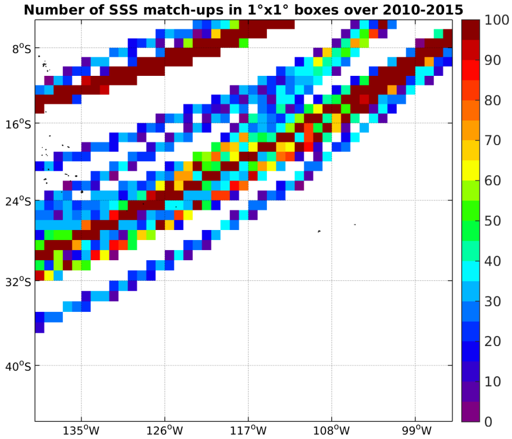
Figure 4: Number of SSS match-ups between TSG-LEGOS-DM SSS and the SMOS-L3-CATDS-CPDC-V3-10DAYS-25KM SSS product for the OTT zone Pi-MEP region over 1°x1° boxes and for the full satellite product period.
