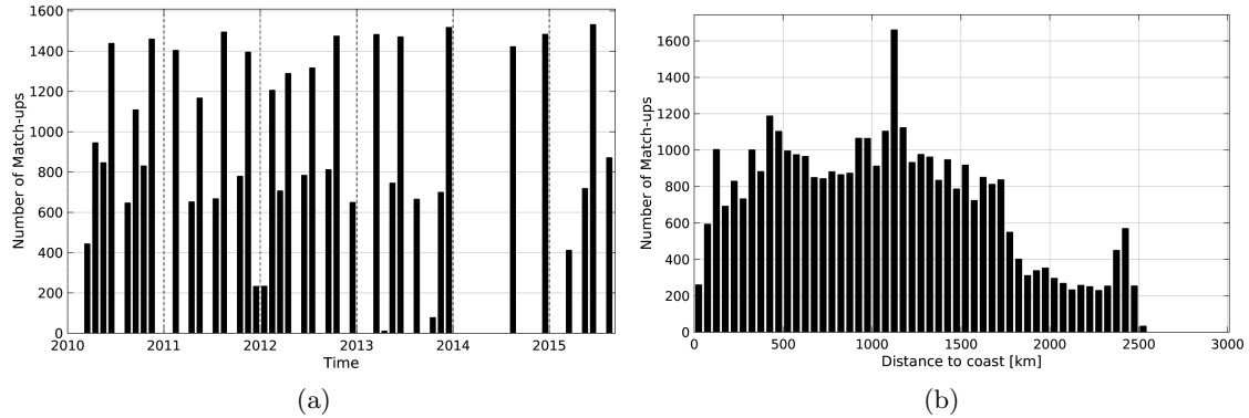
Figure 1: Number of match-ups between TSG-LEGOS-DM and SMOS-L3-CATDS-CPDC-V3-10DAYS-25KM SSS as a function of time (a) and as function of the distance to coast (b) over the OTT zone Pi-MEP region and for the full satellite product period.
