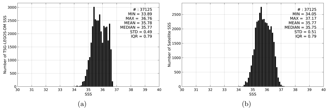
Figure 2: Histograms of SSS from TSG-LEGOS-DM (a) and SMOS-L3-CATDS-CPDC-V3-10DAYS-25KM (b) considering all match-up pairs per bins of 0.1 over the OTT zone Pi-MEP region and for the full satellite product period.
