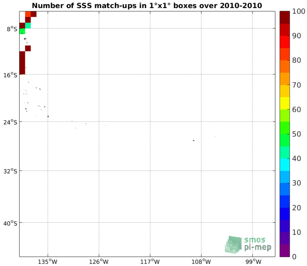
Figure 4: Number of SSS match-ups between TSG-GOSUD-Sailing-ship SSS and the SMOS-L3-CATDS-CPDC-V3-10DAYS-25KM SSS product for the OTT zone Pi-MEP region over 1°x1° boxes and for the full satellite product period.
