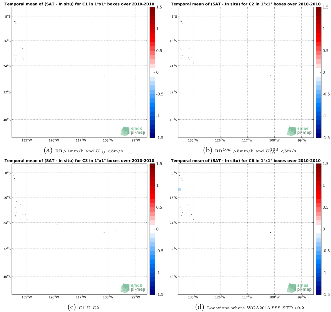
Figure 12: Temporal mean gridded over spatial boxes of size 1^\circ \times 1^\circ of \Delta SSS (SMOS-L3-CATDS-CPDC-V3-10DAYS-25KM - TSG-GOSUD-Sailing-ship) for 4 different subdatasets corresponding to: RR > 1 mm/h and U_{10} < 5 m/s (a), RR 10d > 5 mm/h and U_{10}^{10d} < 5 m/s (b), C1 U C2 (c), Locations where WOA2013 SSS STD > 0.2 (d).
