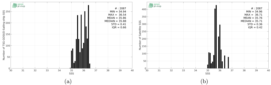
Figure 2: Histograms of SSS from TSG-GOSUD-Sailing-ship (a) and SMOS-L3-CATDS-CPDC-V3-10DAYS-25KM (b) considering all match-up pairs per bins of 0.1 over the OTT zone Pi-MEP region and for the full satellite product period.
