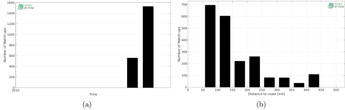
Figure 1: Number of match-ups between TSG-GOSUD-Sailing-ship and SMOS-L3-CATDS-CPDC-V3-10DAYS-25KM SSS as a function of time (a) and as function of the distance to coast (b) over the OTT zone Pi-MEP region and for the full satellite product period.
