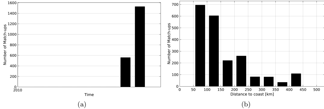
Figure 1: Number of match-ups between TSG-GOSUD-Sailing-ship and SMOS-L3-CATDS-CPDC-V3-10DAYS-25KM SSS as a function of time (a) and as function of the distance to coast (b) over the OTT zone Pi-MEP region and for the full satellite product period.
