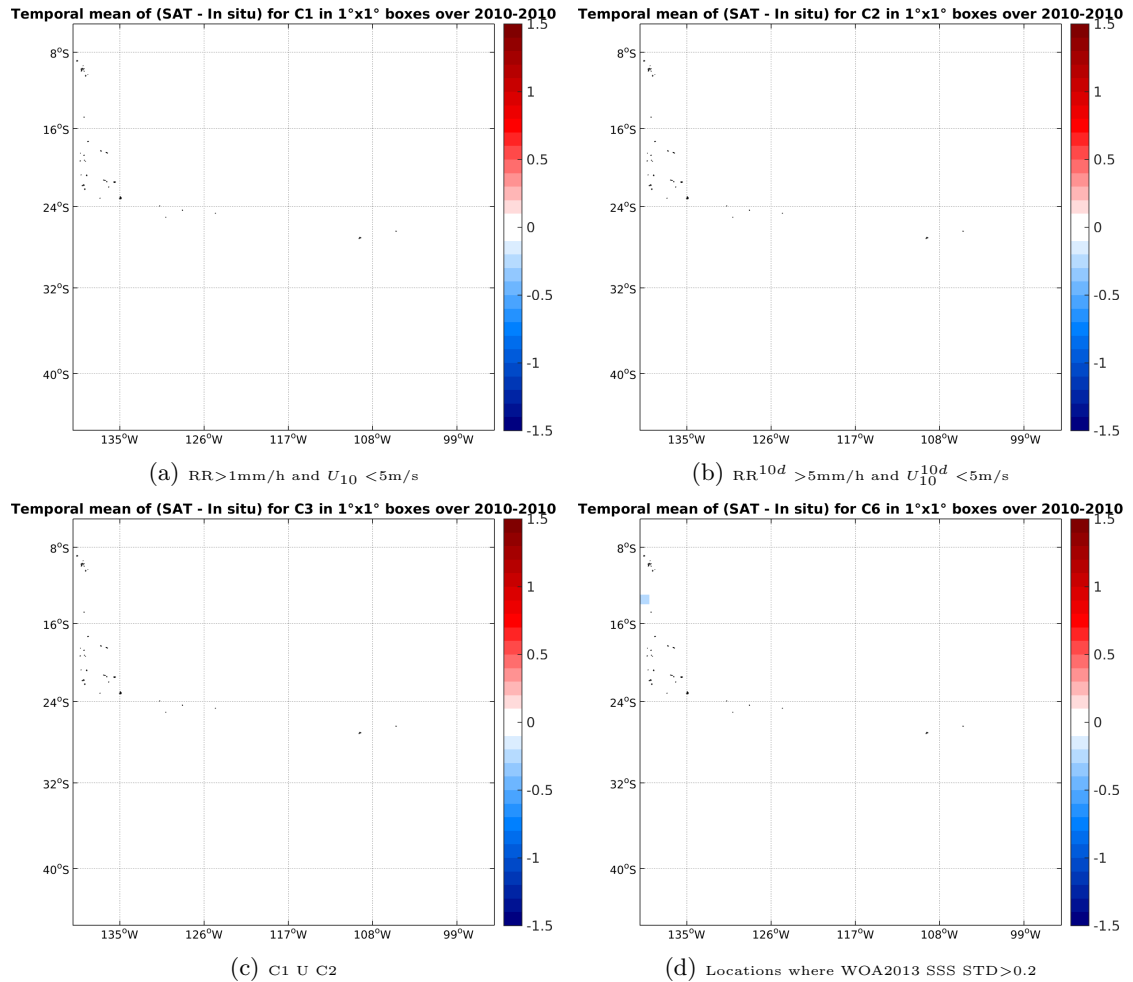
Figure 12: Temporal mean gridded over spatial boxes of size 1^\circ \times 1^\circ of \Delta SSS (SMOS-L3-CATDS-CPDC-V3-10DAYS-25KM - TSG-GOSUD-Sailing-ship) for 4 different subdatasets corresponding to: RR > 1\text{mm/h} and U_{10} < 5\text{m/s} (a), RR^{10d} > 5\text{mm/h} and U_{10}^{10d} < 5\text{m/s} (b), C1 U C2 (c), Locations where WOA2013 SSS STD > 0.2 (d).
