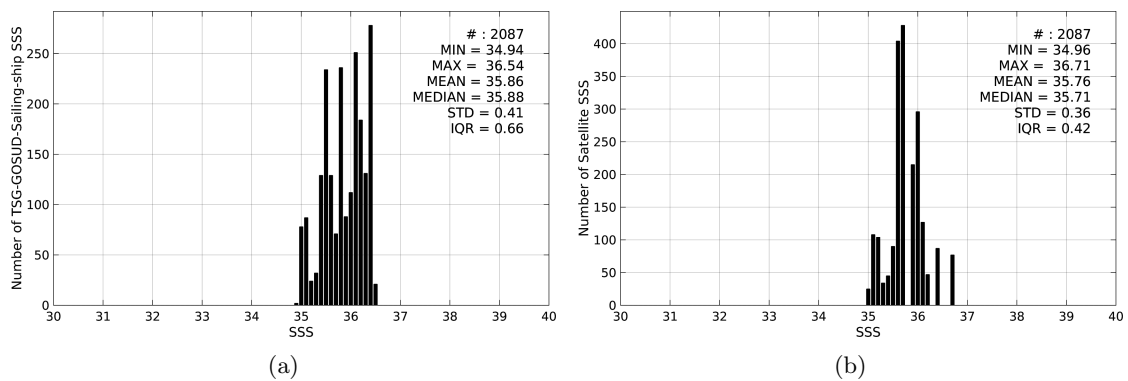
Figure 2: Histograms of SSS from TSG-GOSUD-Sailing-ship (a) and SMOS-L3-CATDS-CPDC-V3-10DAYS-25KM (b) considering all match-up pairs per bins of 0.1 over the OTT zone Pi-MEP region and for the full satellite product period.
