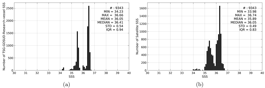
Figure 2: Histograms of SSS from TSG-GOSUD-Research-vessel (a) and SMOS-L3-CATDS-CPDC-V3-10DAYS-25KM (b) considering all match-up pairs per bins of 0.1 over the OTT zone Pi-MEP region and for the full satellite product period.
