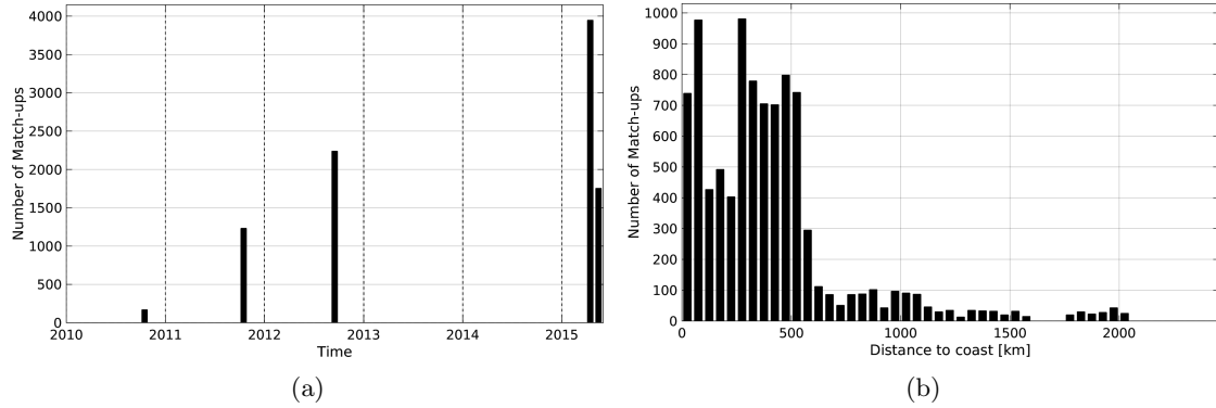
Figure 1: Number of match-ups between TSG-GOSUD-Research-vessel and SMOS-L3-CATDS-CPDC-V3-10DAYS-25KM SSS as a function of time (a) and as function of the distance to coast (b) over the OTT zone Pi-MEP region and for the full satellite product period.
