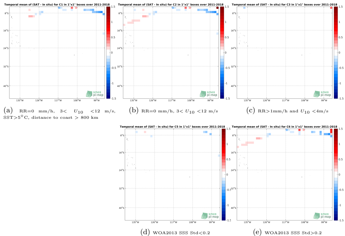
Figure 12: Temporal mean gridded over spatial boxes of size 1^\circ \times 1^\circ of \Delta SSS (SMOS SSS L3 v2 - 9-Days (BEC) - TSG (SAMOS)) for 5 different subdatasets corresponding to:RR=0 mm/h, 3 < U_{10} < 12 m/s, SST >5^\circ C, distance to coast > 800 km (a), RR=0 mm/h, 3 < U_{10} < 12 m/s (b), RR >1 mm/h and U_{10} < 4 m/s (c), WOA2013 SSS Std <0.2 (d), WOA2013 SSS Std >0.2 (e).
