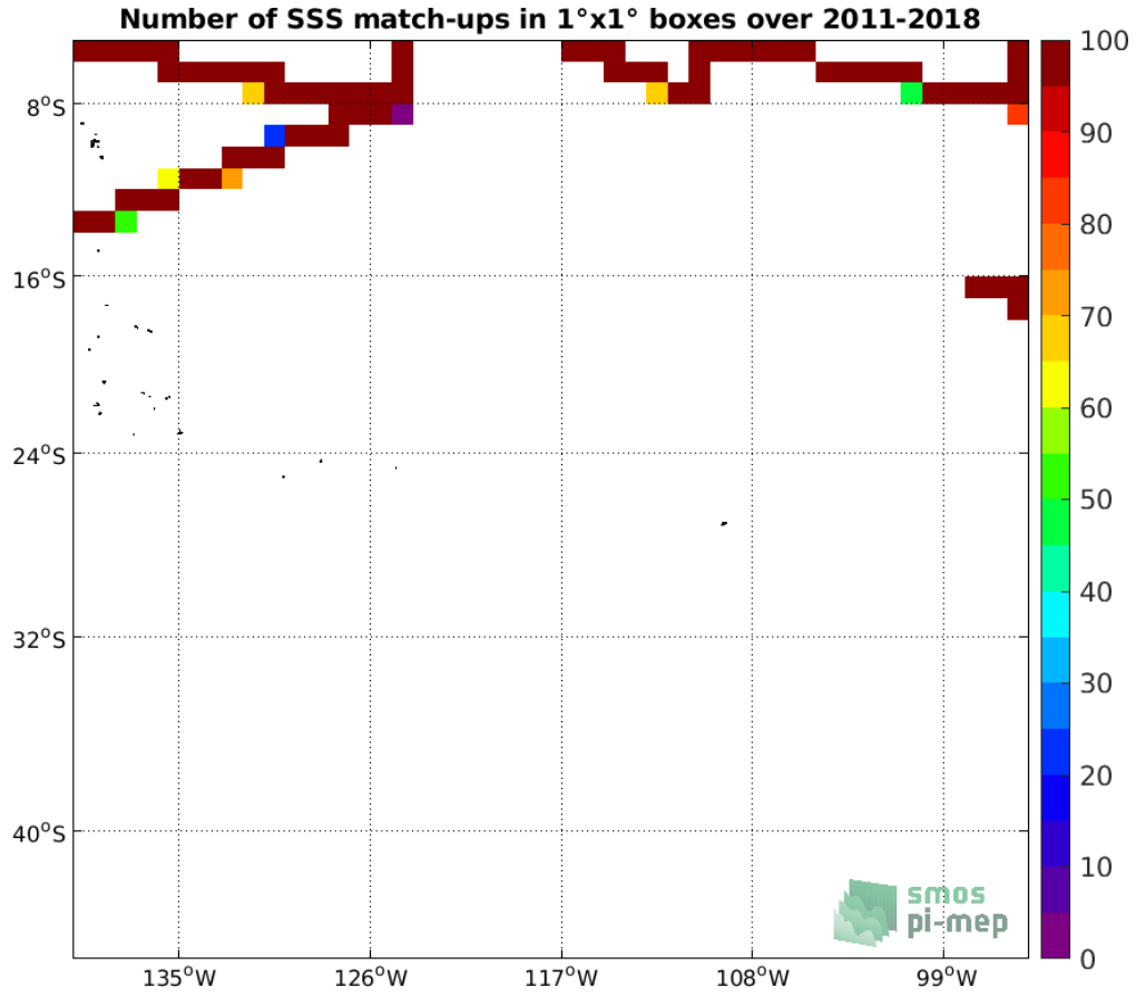
Figure 4: Number of SSS match-ups between TSG (SAMOS) SSS and the SMOS SSS L3 v2 - 9-Days (BEC) SSS product for the OTT zone Pi-MEP region over 1^\circ \times 1^\circ boxes and for the full satellite product period.
