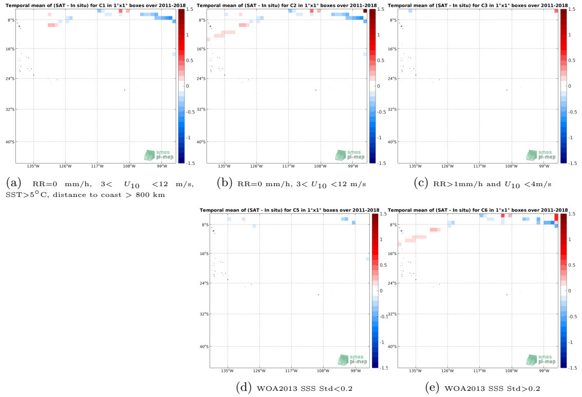
Figure 12: Temporal mean gridded over spatial boxes of size 1^\circ \times 1^\circ of \Delta SSS (SMOS SSS L3 v2 - 9-Days (BEC) - TSG (SAMOS)) for 5 different subdatasets corresponding to: RR=0 mm/h, 3 < U_{10} < 12 m/s, SST > 5^\circ C , distance to coast > 800 km (a), RR=0 mm/h, 3 < U_{10} < 12 m/s (b), RR > 1 mm/h and U_{10} < 4 m/s (c), WOA2013 SSS Std < 0.2 (d), WOA2013 SSS Std > 0.2 (e).
