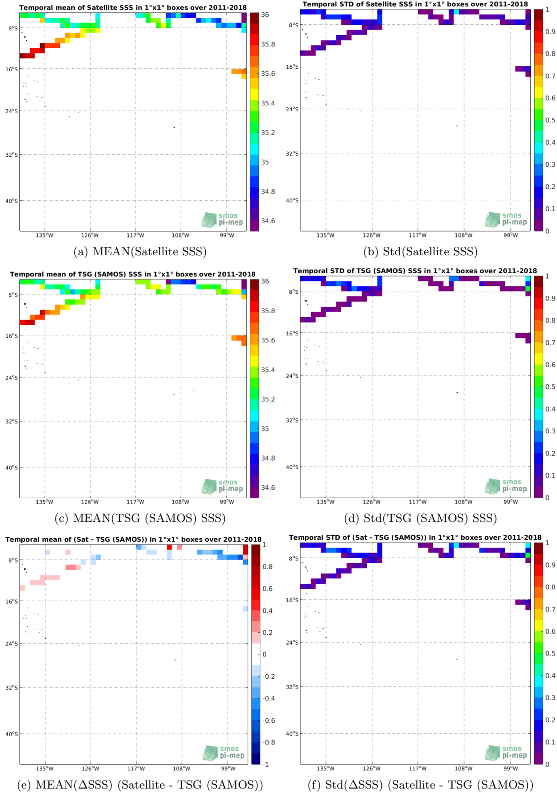
Figure 6: Temporal mean (left) and Std (right) of SSS from SMOS SSS L3 v2 - 9-Days (BEC) (top), TSG (SAMOS) (middle), and of \Delta SSS (Satellite - TSG (SAMOS)). Only match-up pairs are used to generate these maps.
