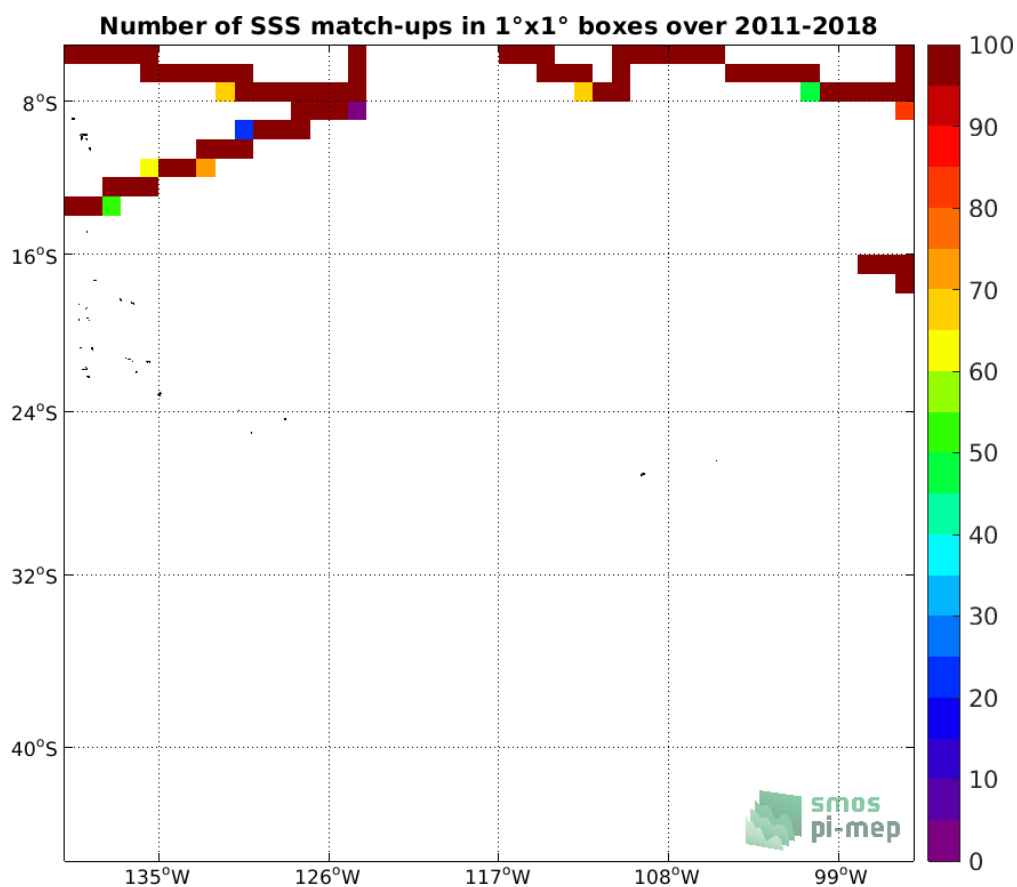
Figure 4: Number of SSS match-ups between TSG (SAMOS) SSS and the SMOS SSS L3 v2 - 9-Days (BEC) SSS product for the OTT zone Pi-MEP region over 1°x1° boxes and for the full satellite product period.
