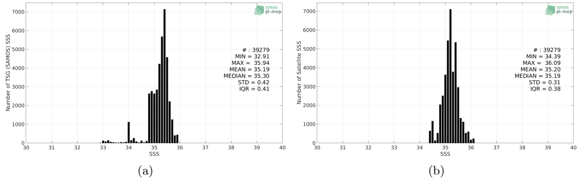
Figure 2: Histograms of SSS from TSG (SAMOS) (a) and SMOS SSS L3 v2 - 9-Days (BEC) (b) considering all match-up pairs per bins of 0.1 over the OTT zone Pi-MEP region and for the full satellite product period.
