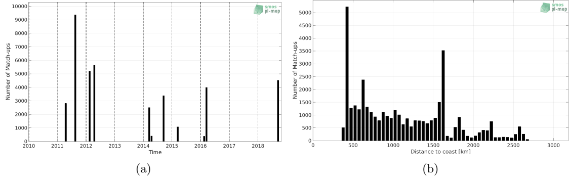
Figure 1: Number of match-ups between TSG (SAMOS) and SMOS SSS L3 v2 - 9-Days (BEC) SSS as a function of time (a) and as function of the distance to coast (b) over the OTT zone Pi-MEP region and for the full satellite product period.
